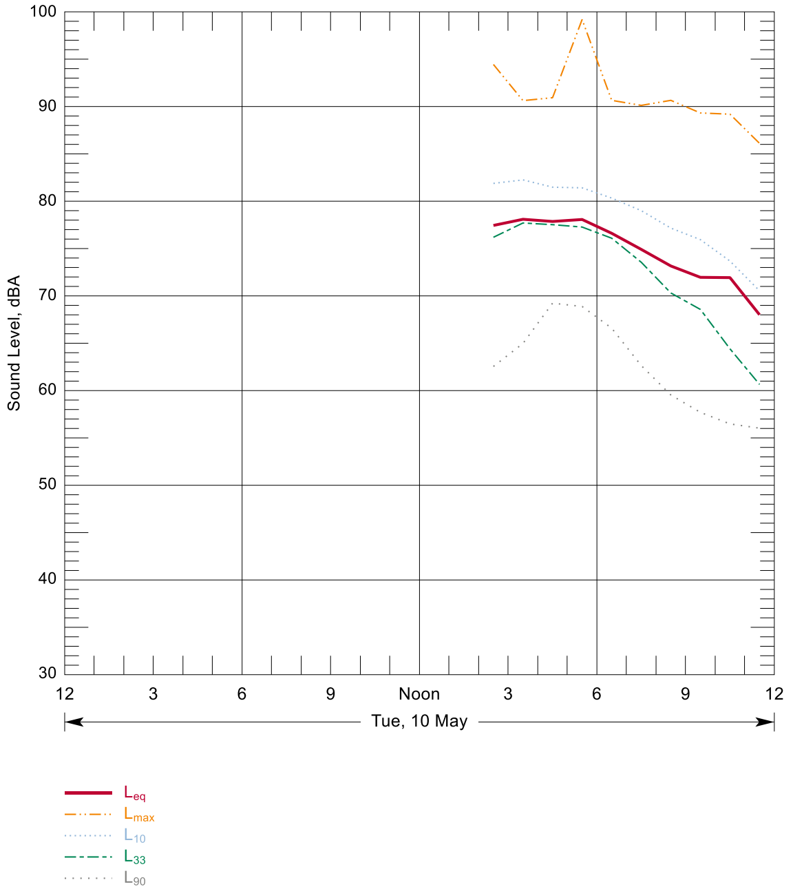
Figure B-81: Hourly Summary of Noise Levels Measured at N100 on 10 May, 2016
