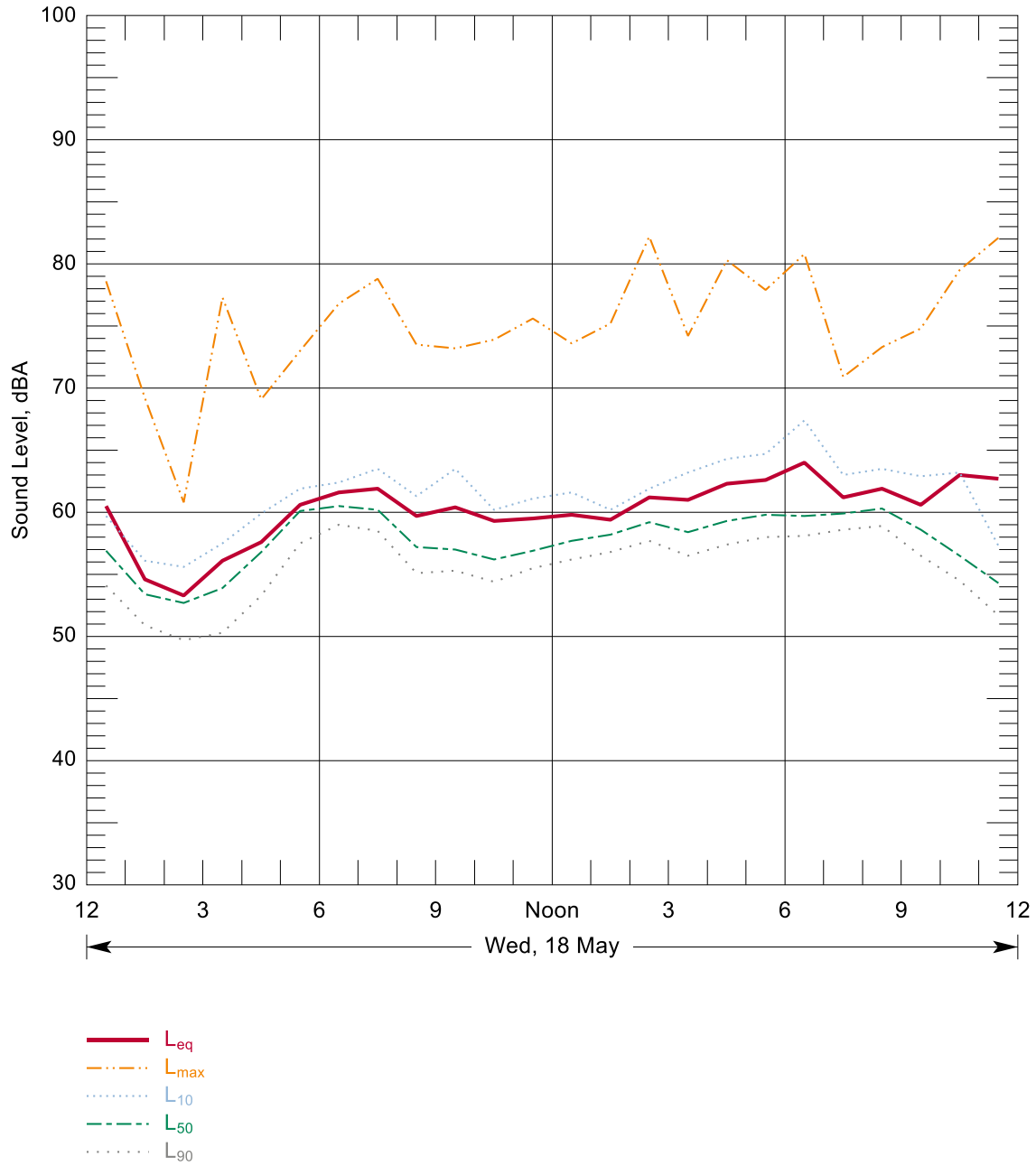
Figure B-32: Hourly Summary of Noise Levels Measured at N83 on 18 May, 2016
