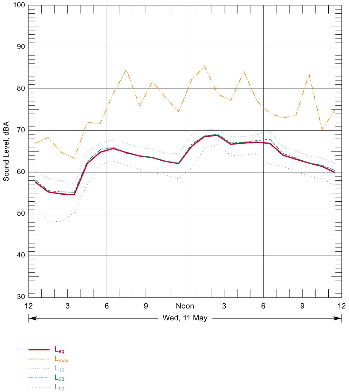
Figure B-91: Hourly Summary of Noise Levels Measured at N102 on 11 May, 2016
