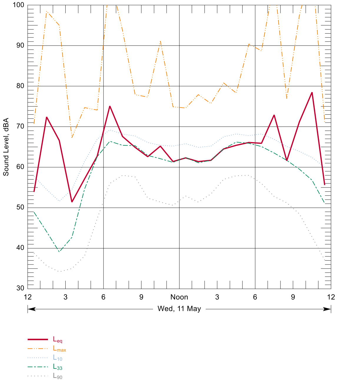
Figure B-87: Hourly Summary of Noise Levels Measured at N101 on 11 May, 2016
