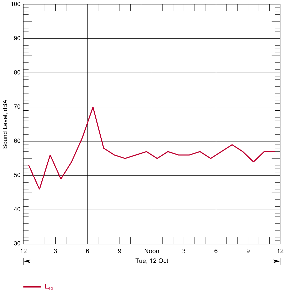
Figure B-37: Hourly Summary of Noise Levels Measured at N85 on 12 Oct, 2010
