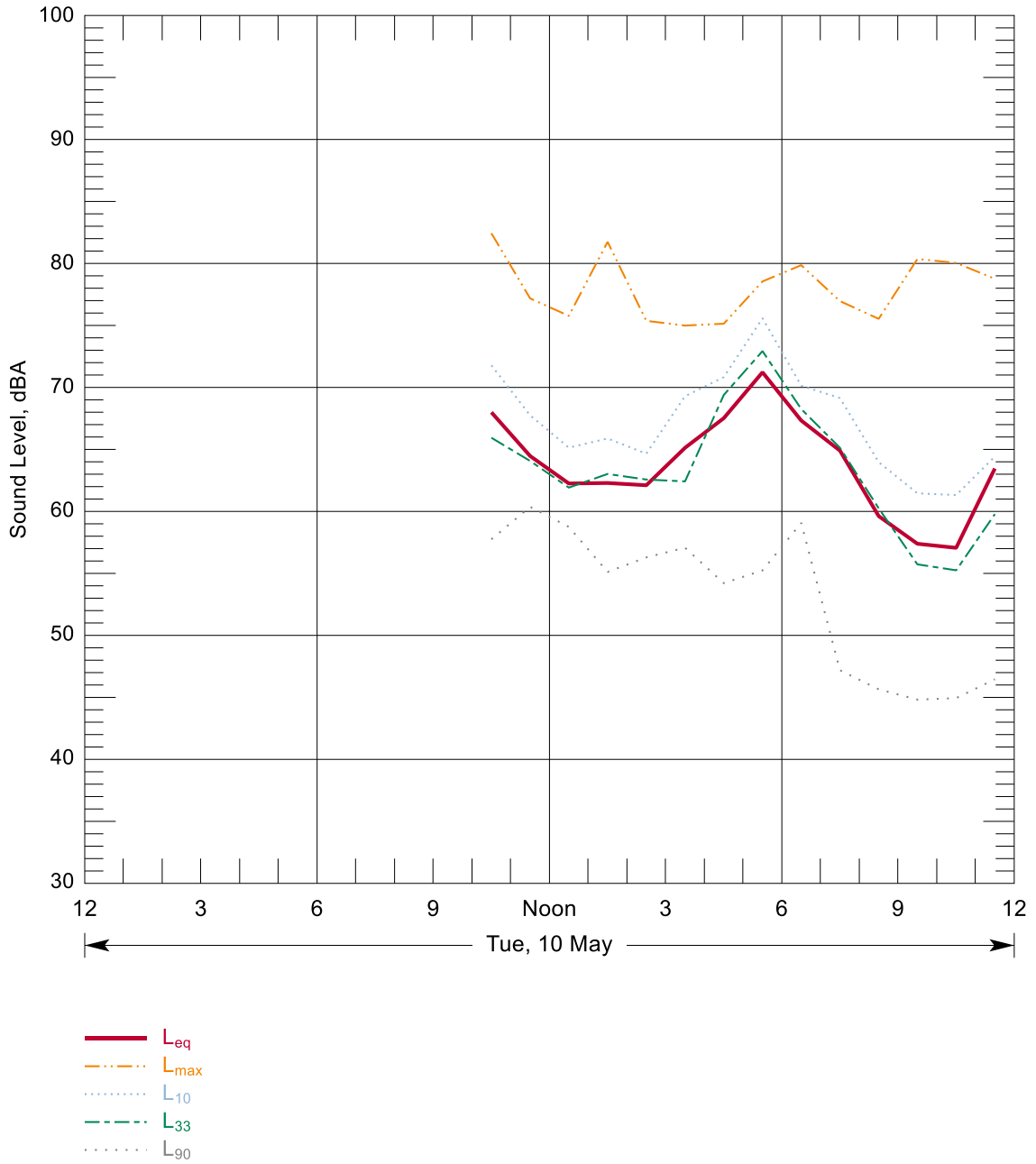
Figure B-17: Hourly Summary of Noise Levels Measured at N79 on 10 May, 2016
