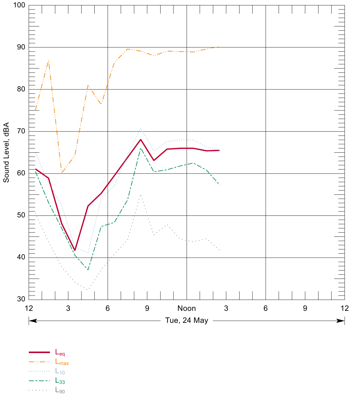
Figure B-213: Hourly Summary of Noise Levels Measured at N138 on 24 May, 2016
