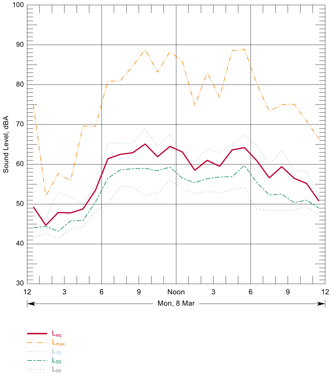
Figure B-15: Hourly Summary of Noise Levels Measured at N78 on 08 Mar, 2010
