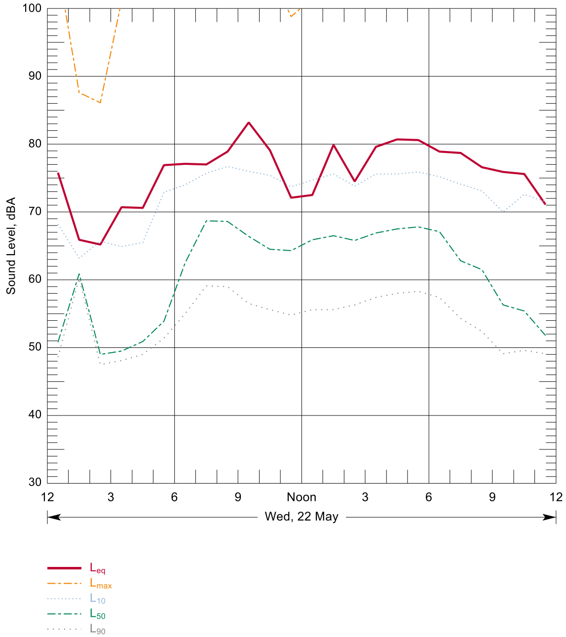
Figure B-216: Hourly Summary of Noise Levels Measured at N139 on 22 May, 2013
