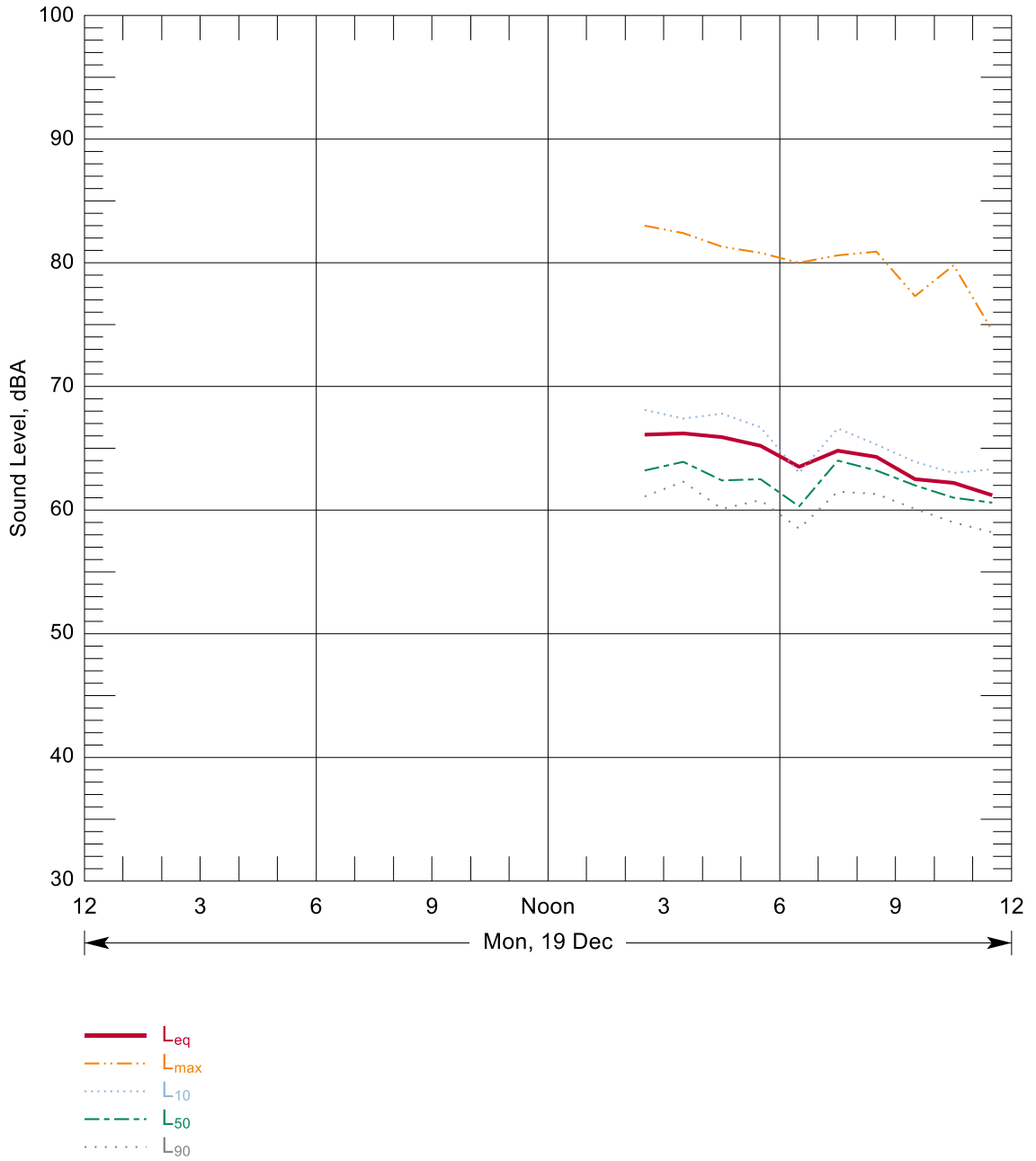
Figure B-113: Hourly Summary of Noise Levels Measured at N110 on 19 Dec, 2016
