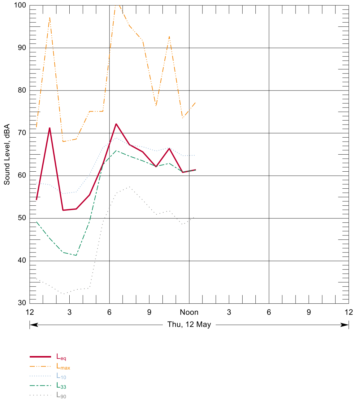
Figure B-88: Hourly Summary of Noise Levels Measured at N101 on 12 May, 2016
