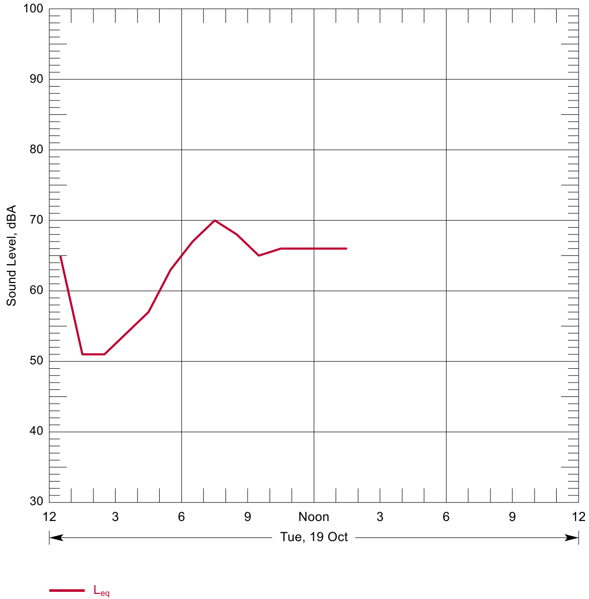
Figure B-94: Hourly Summary of Noise Levels Measured at N103 on 19 Oct, 2010
