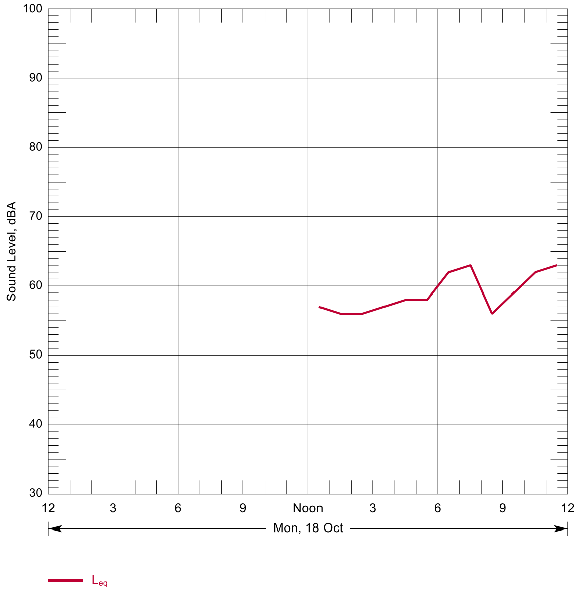
Figure B-108: Hourly Summary of Noise Levels Measured at N108 on 18 Oct, 2010
