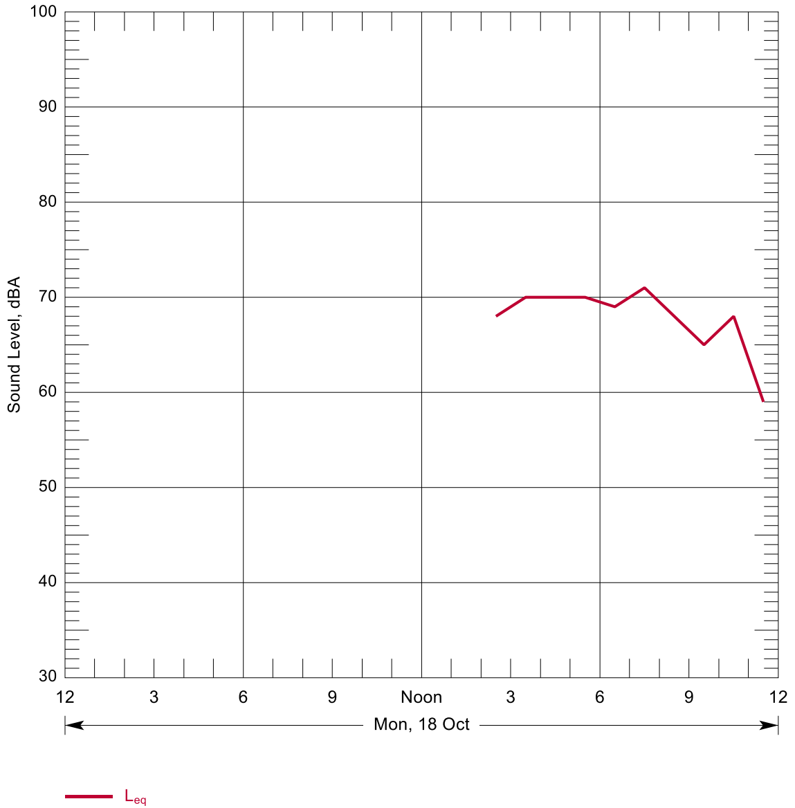
Figure B-93: Hourly Summary of Noise Levels Measured at N103 on 18 Oct, 2010
