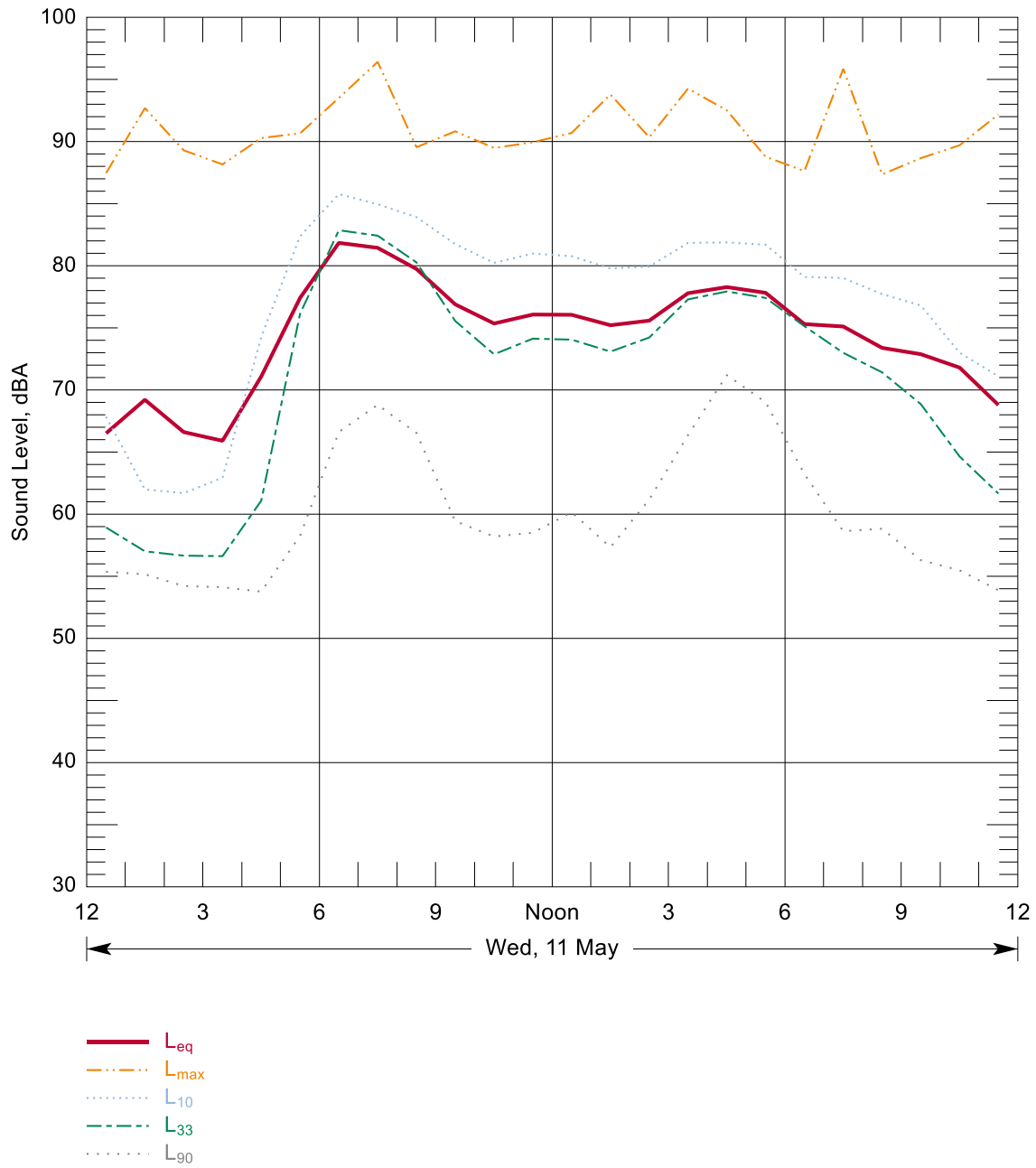
Figure B-82: Hourly Summary of Noise Levels Measured at N100 on 11 May, 2016
