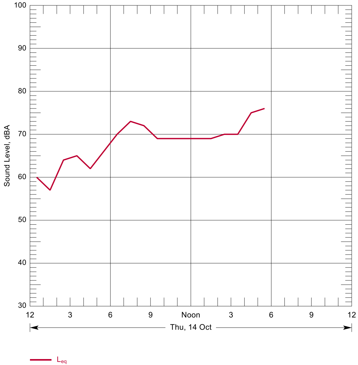
Figure B-66: Hourly Summary of Noise Levels Measured at N94 on 14 Oct, 2010
