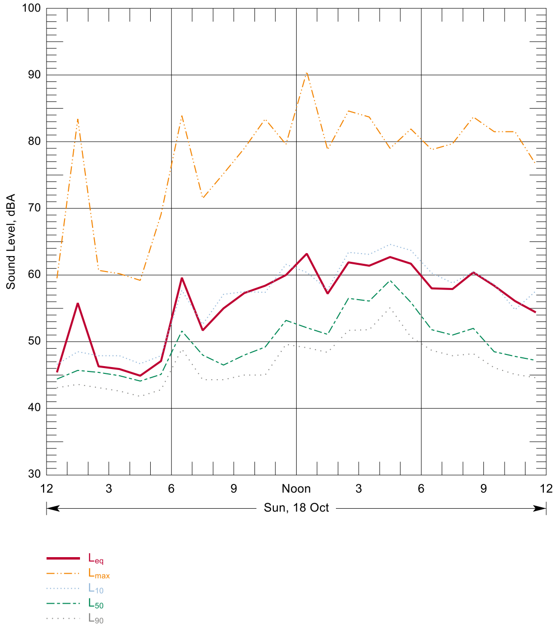
Figure B-8: Hourly Summary of Noise Levels Measured at N77 on 18 Oct, 2009
