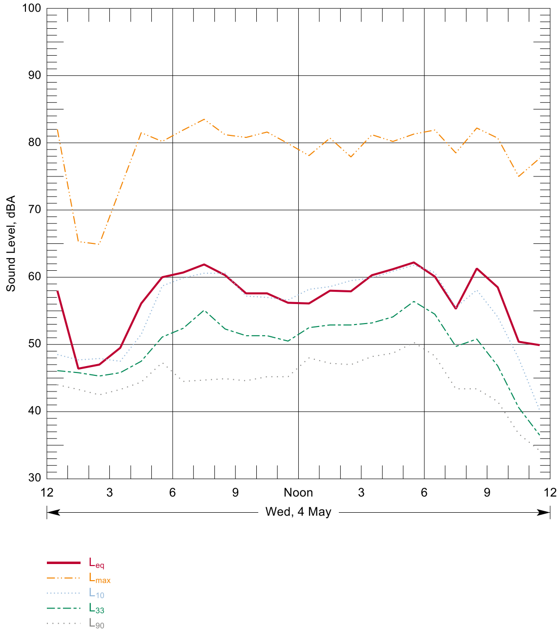
Figure B-2: Hourly Summary of Noise Levels Measured at N76 on 04 May, 2016
