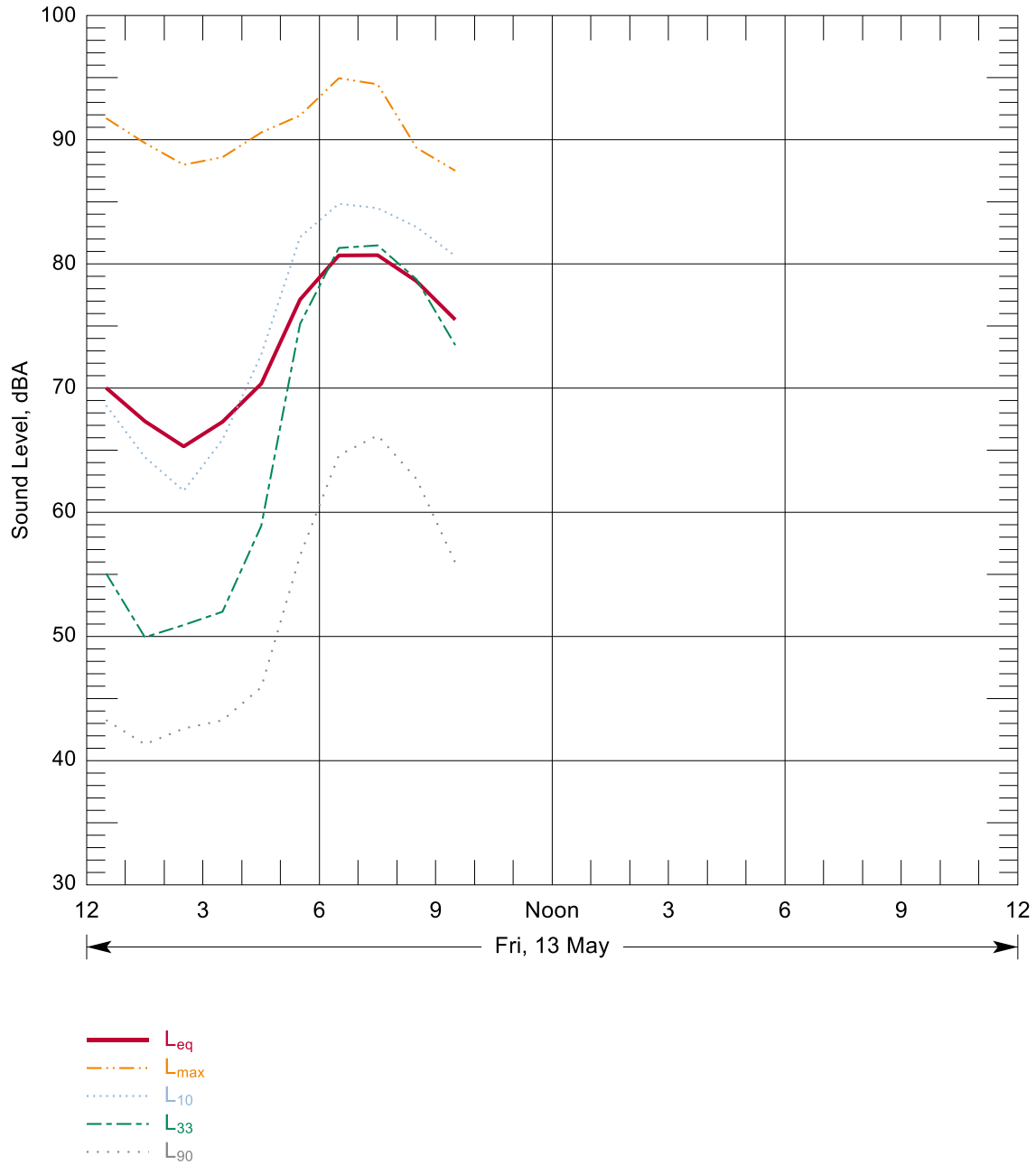
Figure B-84: Hourly Summary of Noise Levels Measured at N100 on 13 May, 2016
