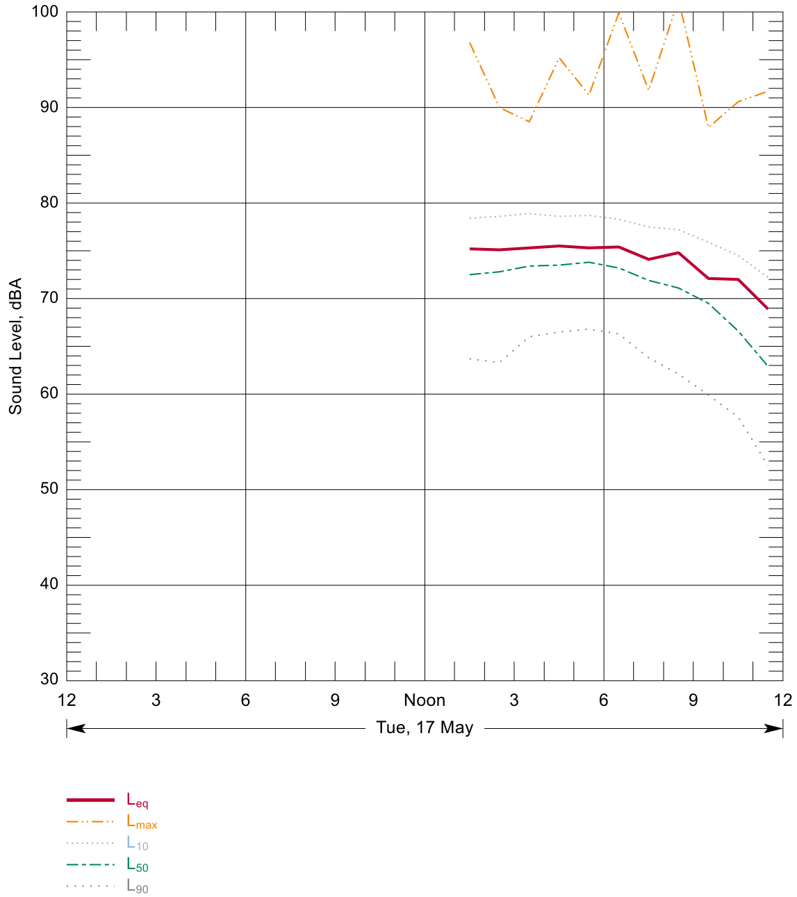
Figure B-42: Hourly Summary of Noise Levels Measured at N87 on 17 May, 2016
