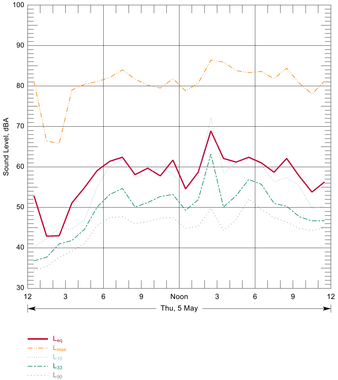
Figure B-3: Hourly Summary of Noise Levels Measured at N76 on 05 May, 2016
