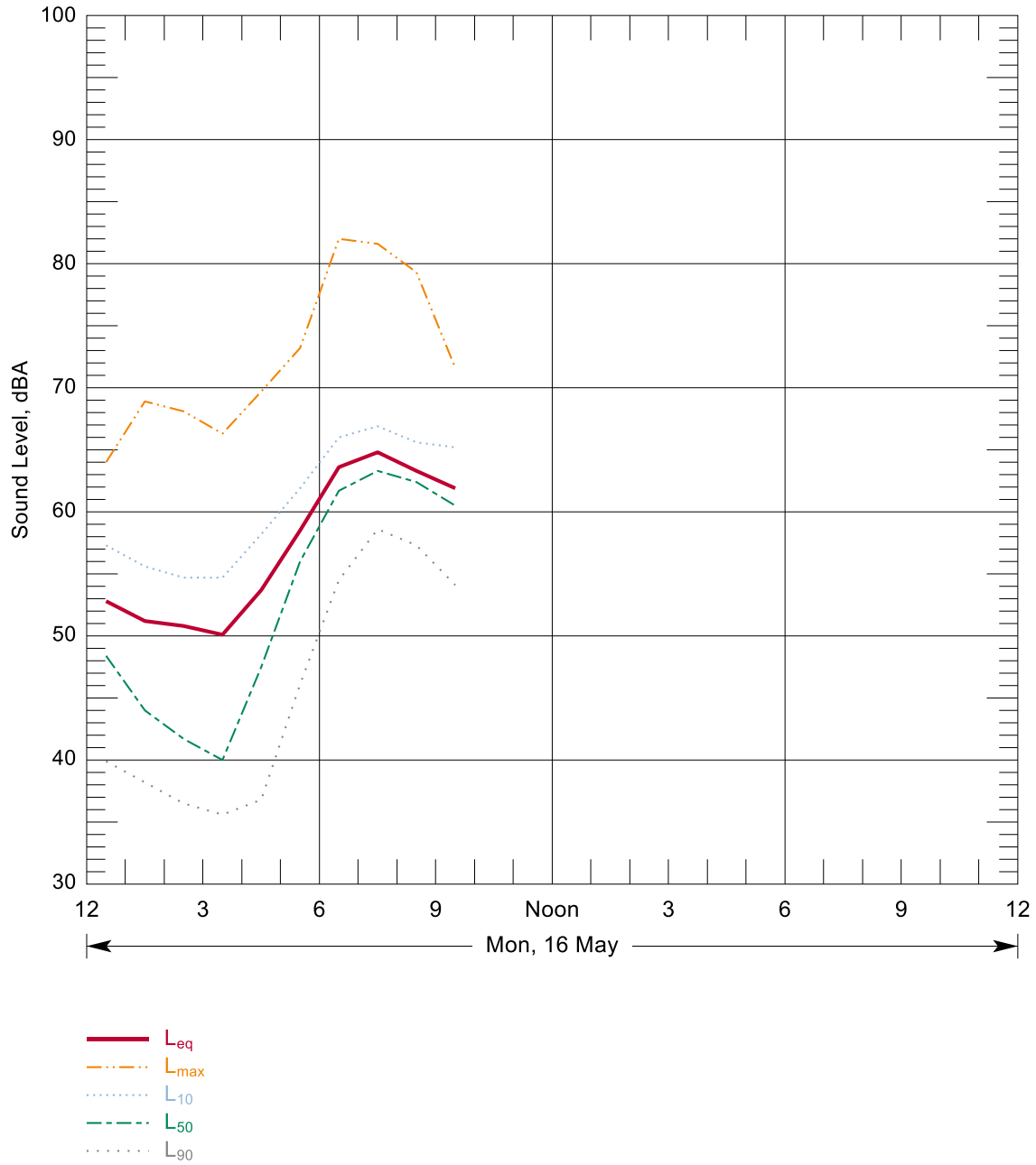
Figure B-58: Hourly Summary of Noise Levels Measured at N91 on 16 May, 2016
