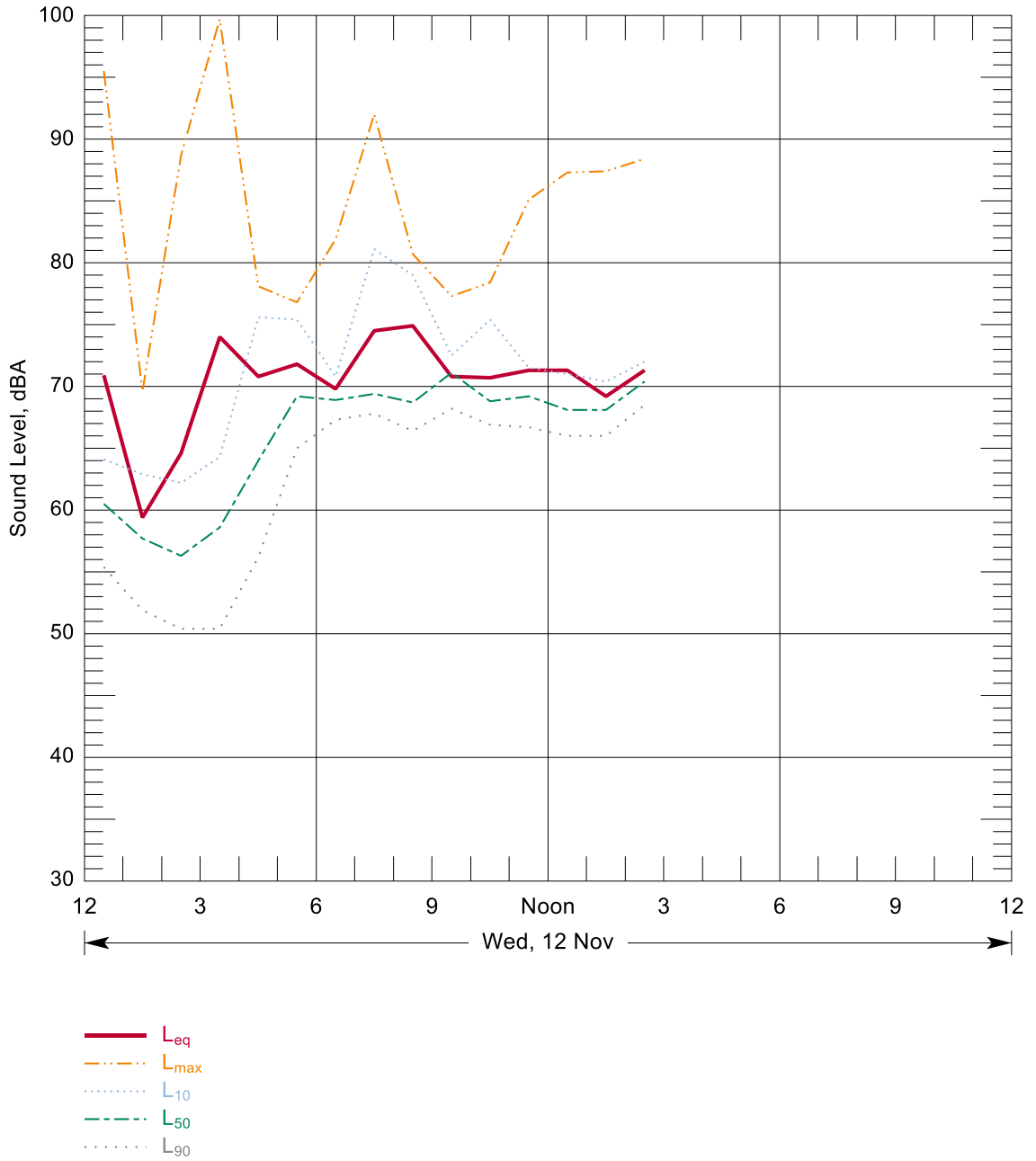
Figure B-35: Hourly Summary of Noise Levels Measured at N84 on 12 Nov, 2014
