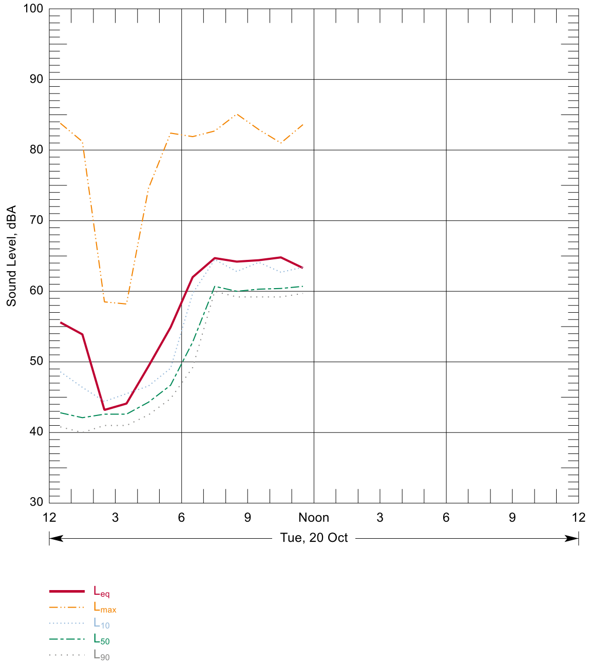
Figure B-10: Hourly Summary of Noise Levels Measured at N77 on 20 Oct, 2009
