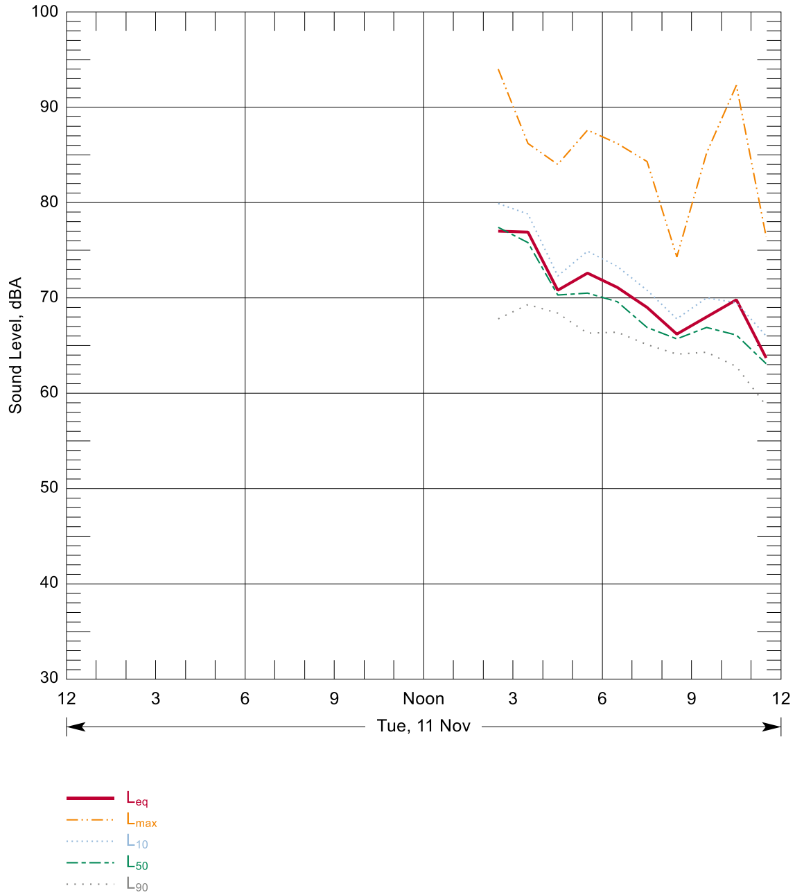
Figure B-34: Hourly Summary of Noise Levels Measured at N84 on 11 Nov, 2014
