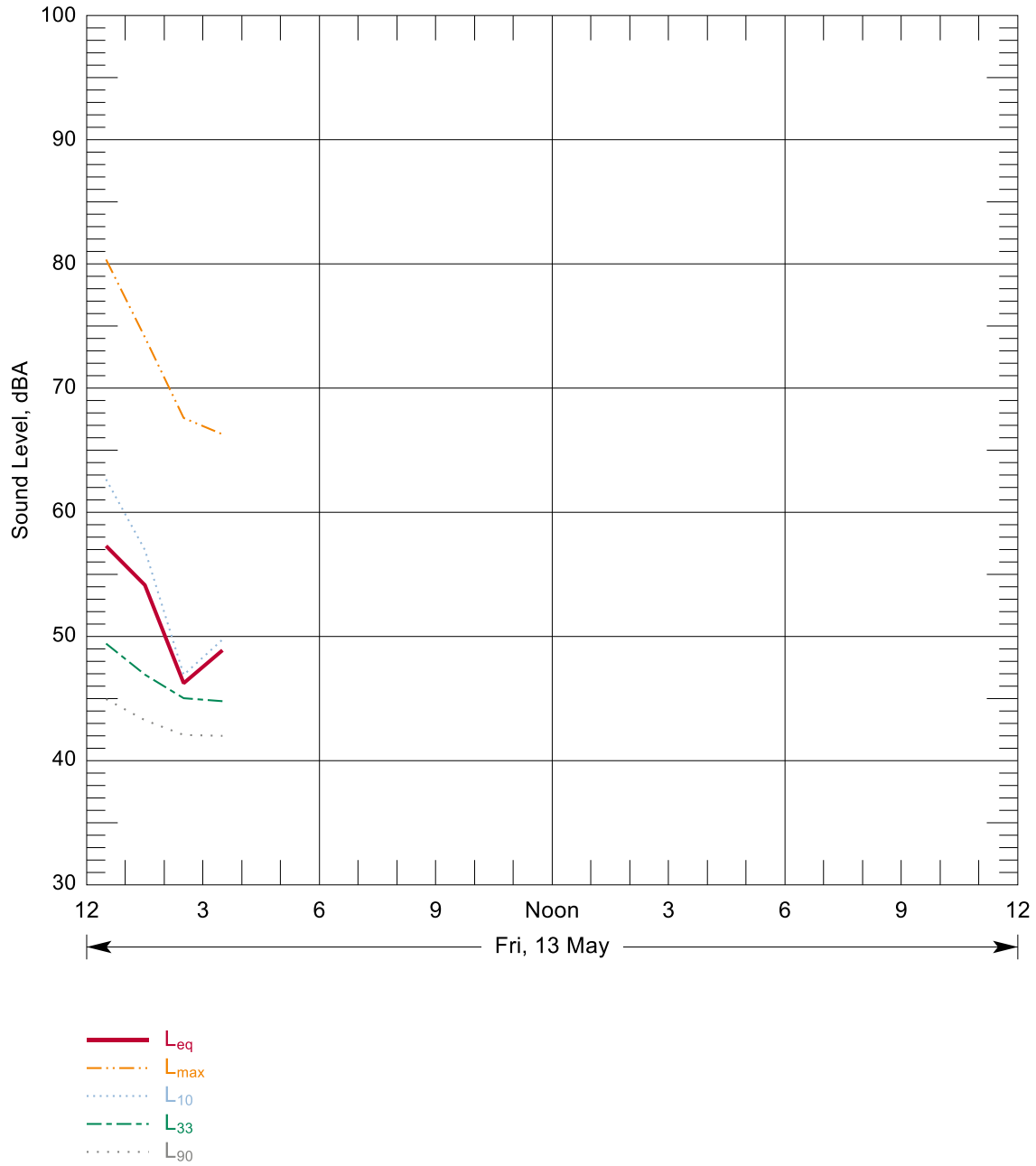
Figure B-20: Hourly Summary of Noise Levels Measured at N79 on 13 May, 2016
