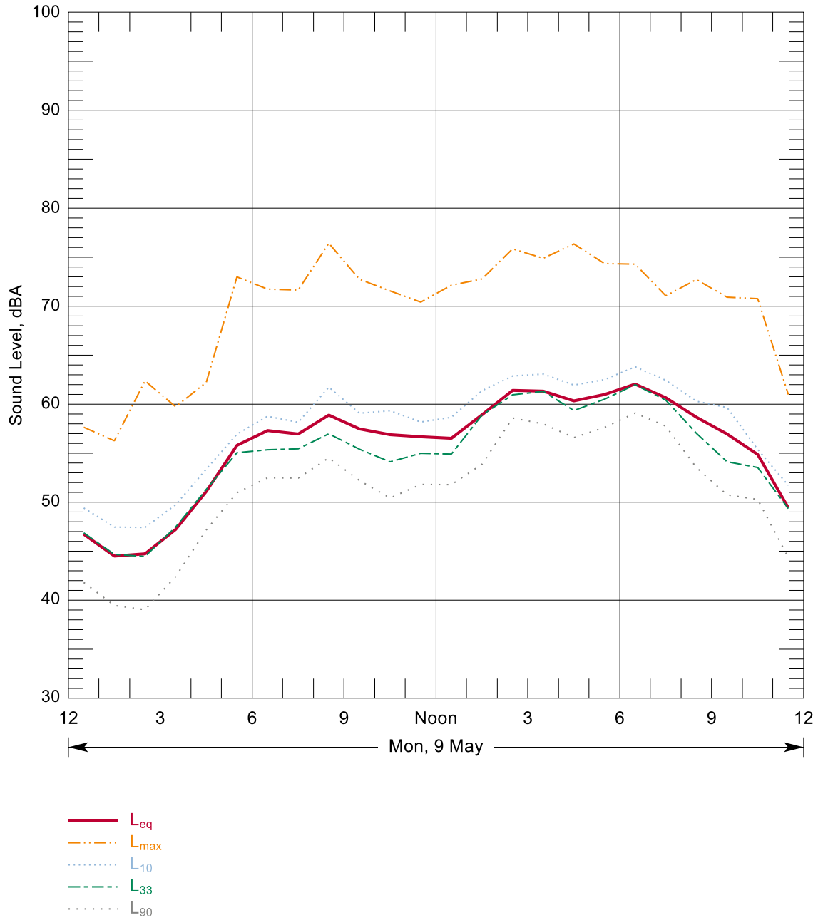
Figure B-26: Hourly Summary of Noise Levels Measured at N81 on 09 May, 2016
