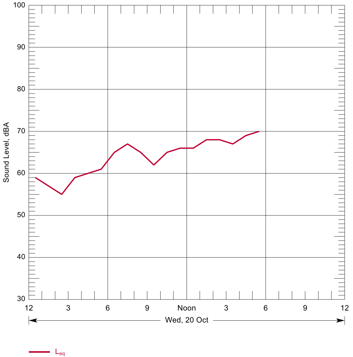
Figure B-107: Hourly Summary of Noise Levels Measured at N107 on 20 Oct, 2010
