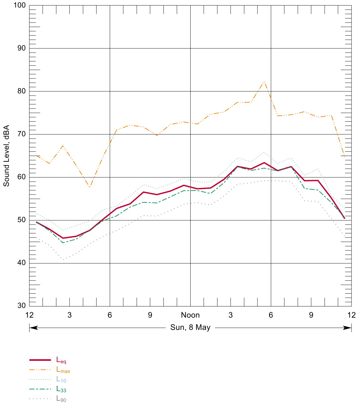
Figure B-25: Hourly Summary of Noise Levels Measured at N81 on 08 May, 2016
