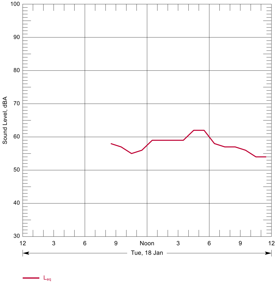
Figure B-79: Hourly Summary of Noise Levels Measured at N99 on 18 Jan, 2011
