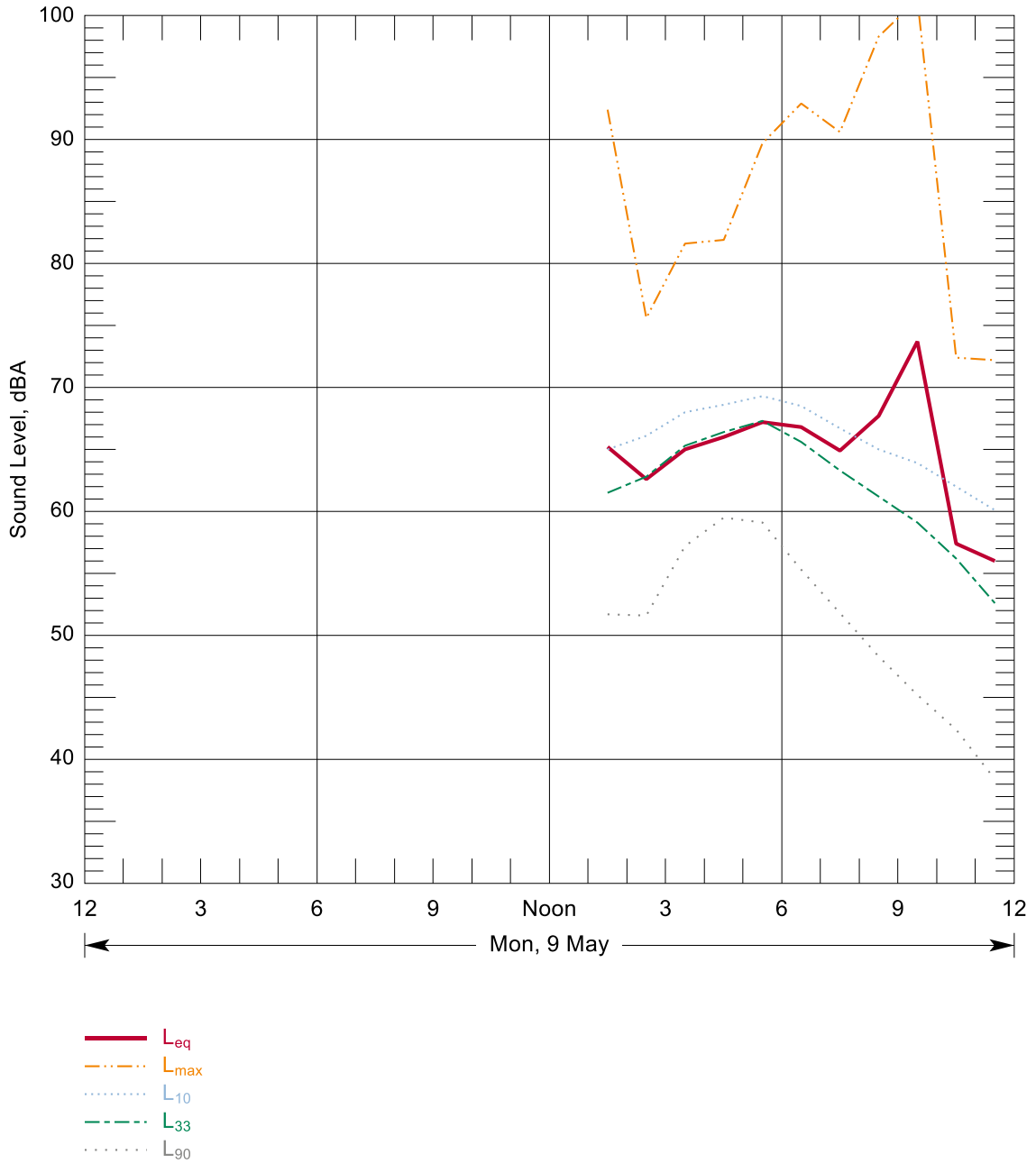
Figure B-85: Hourly Summary of Noise Levels Measured at N101 on 09 May, 2016
