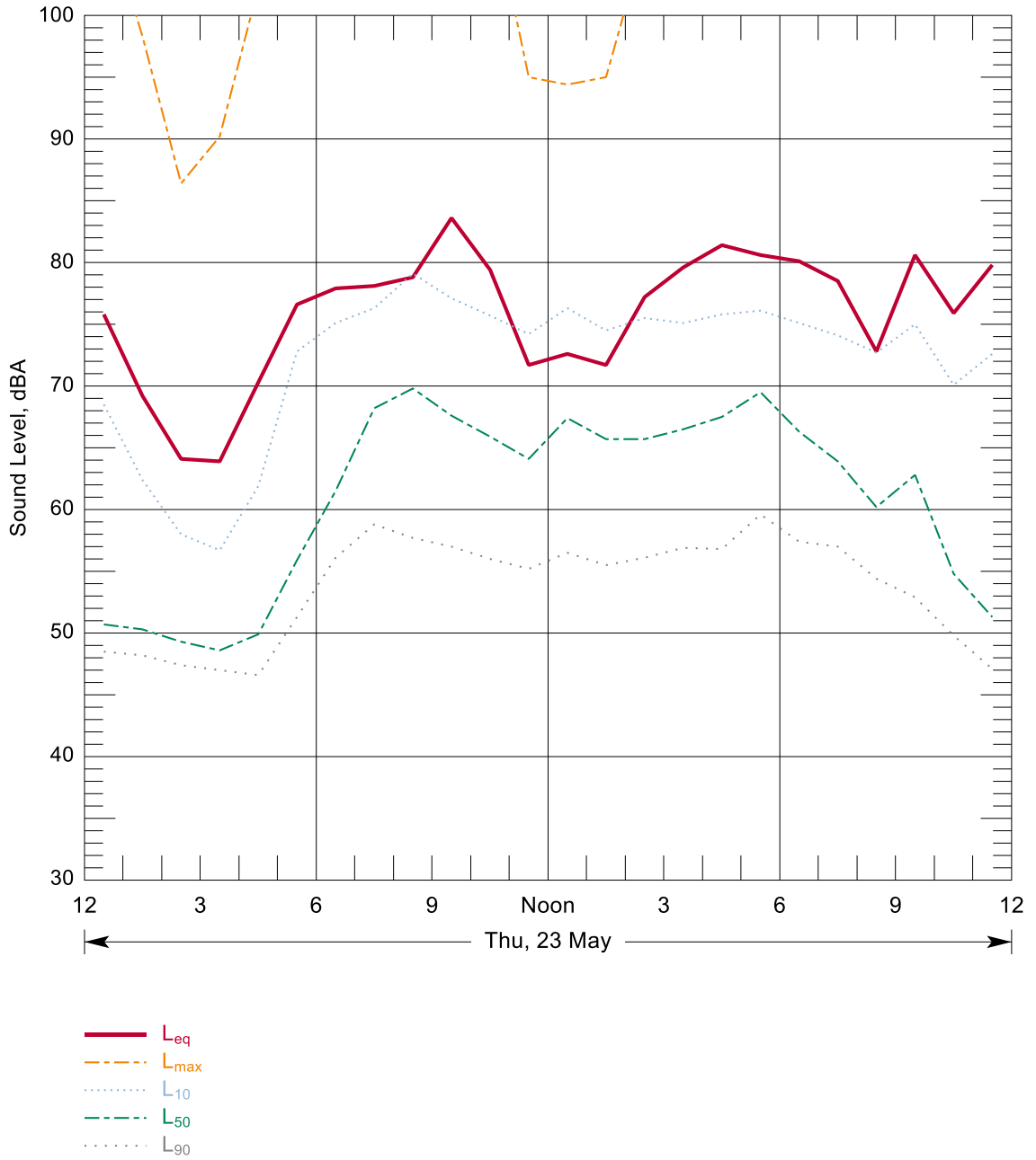
Figure B-217: Hourly Summary of Noise Levels Measured at N139 on 23 May, 2013
