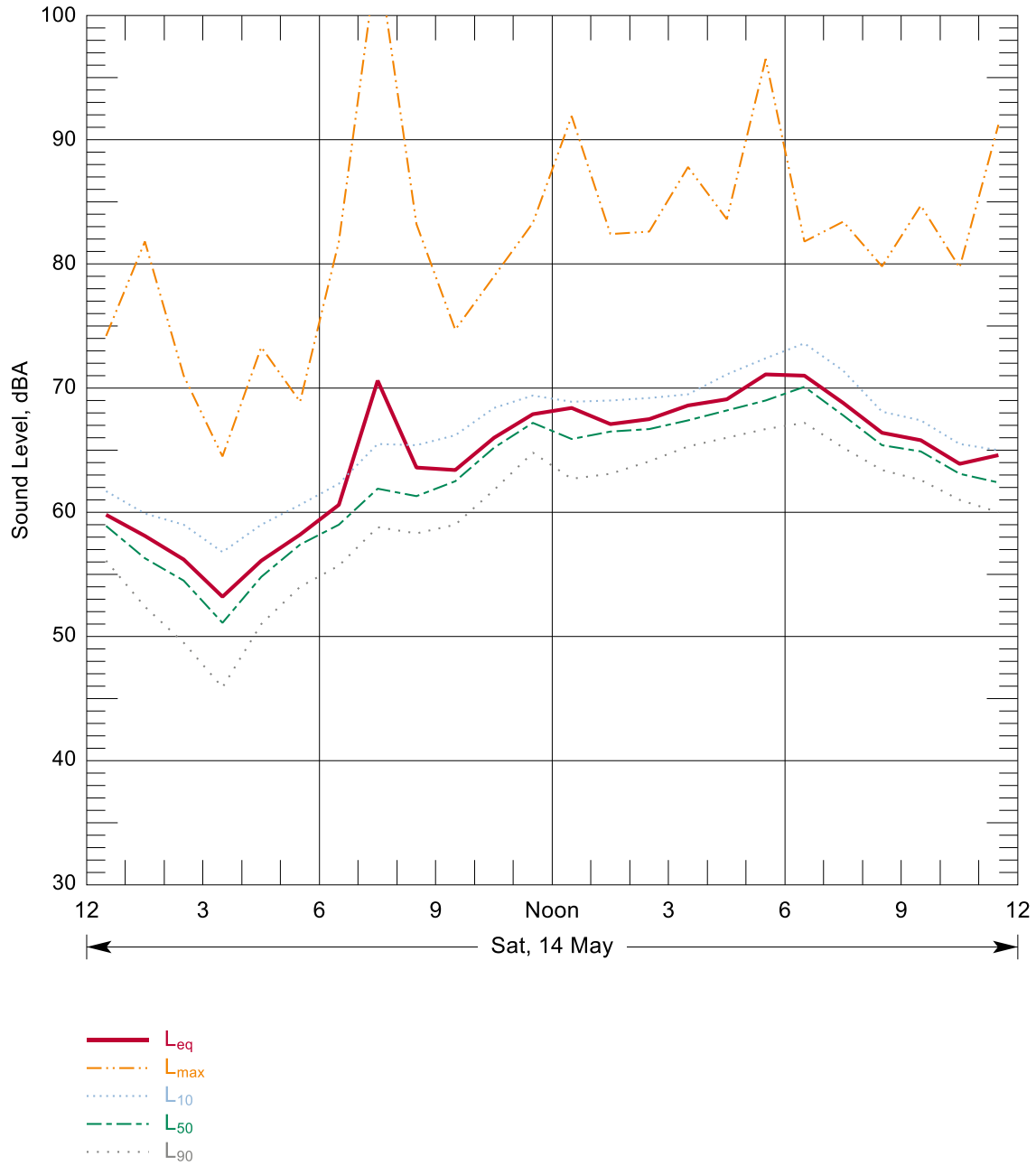
Figure B-100: Hourly Summary of Noise Levels Measured at N105 on 14 May, 2016
