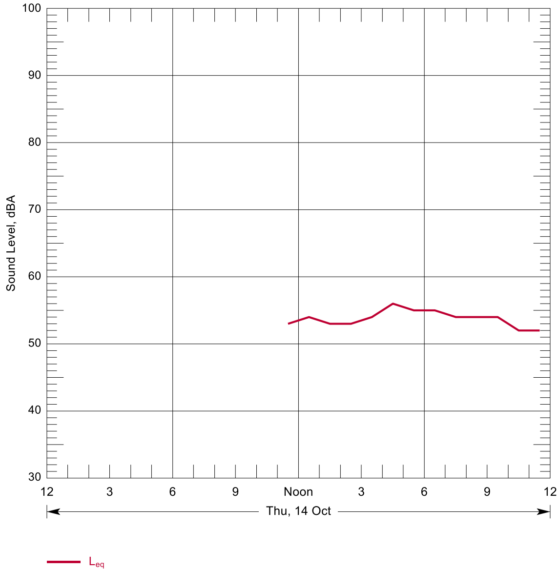
Figure B-74: Hourly Summary of Noise Levels Measured at N97 on 14 Oct, 2010
