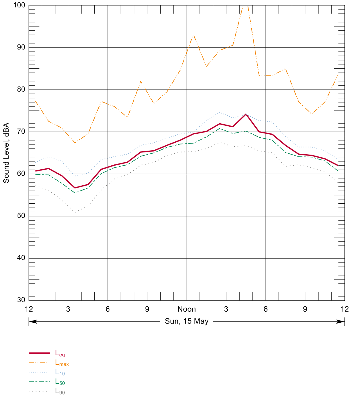
Figure B-101: Hourly Summary of Noise Levels Measured at N105 on 15 May, 2016
