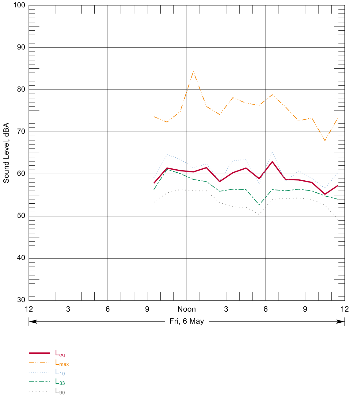
Figure B-23: Hourly Summary of Noise Levels Measured at N81 on 06 May, 2016
