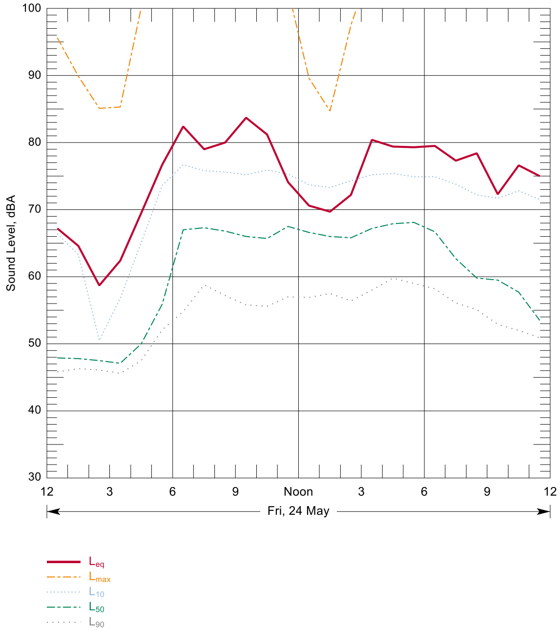
Figure B-218: Hourly Summary of Noise Levels Measured at N139 on 24 May, 2013
