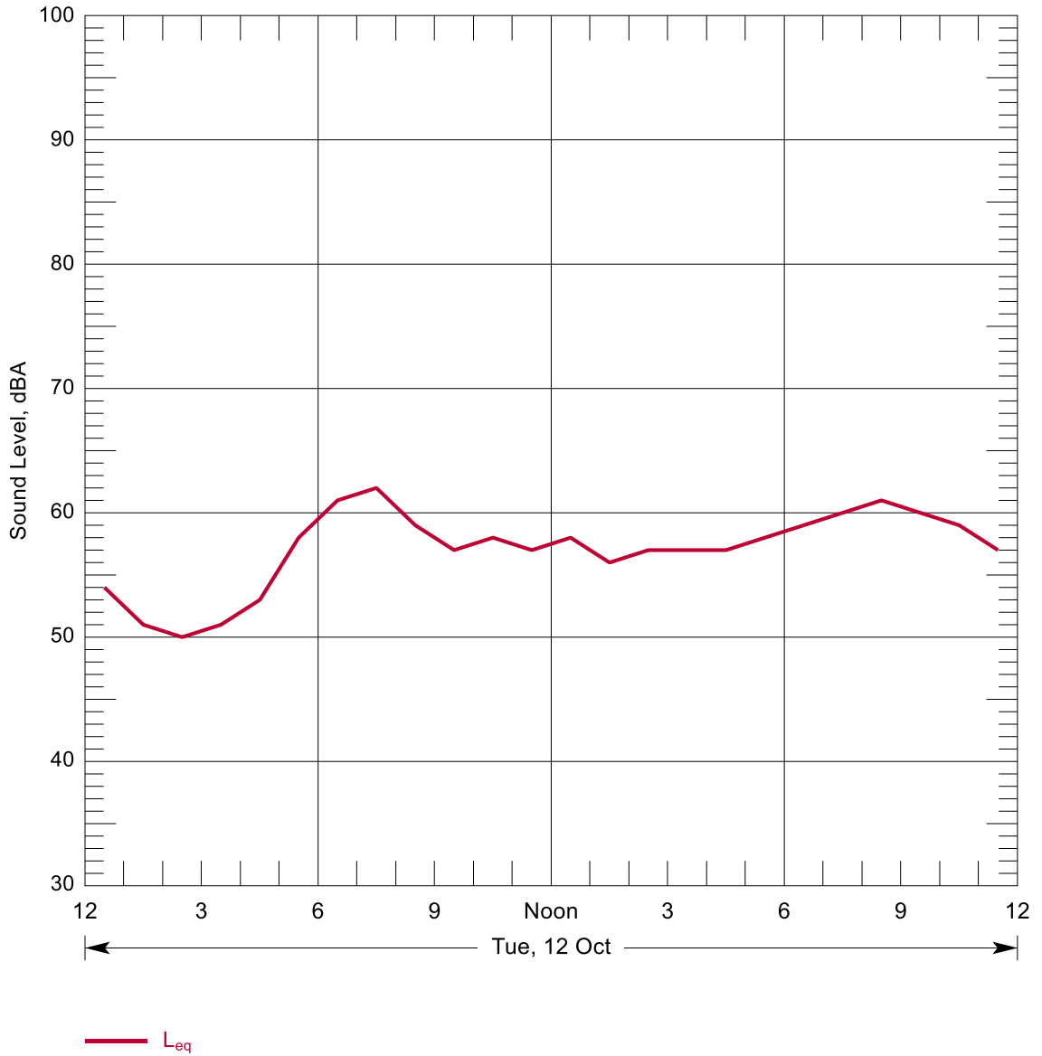
Figure B-29: Hourly Summary of Noise Levels Measured at N82 on 12 Oct, 2010
