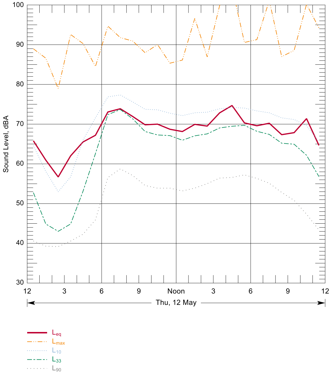
Figure B-63: Hourly Summary of Noise Levels Measured at N93 on 12 May, 2016
