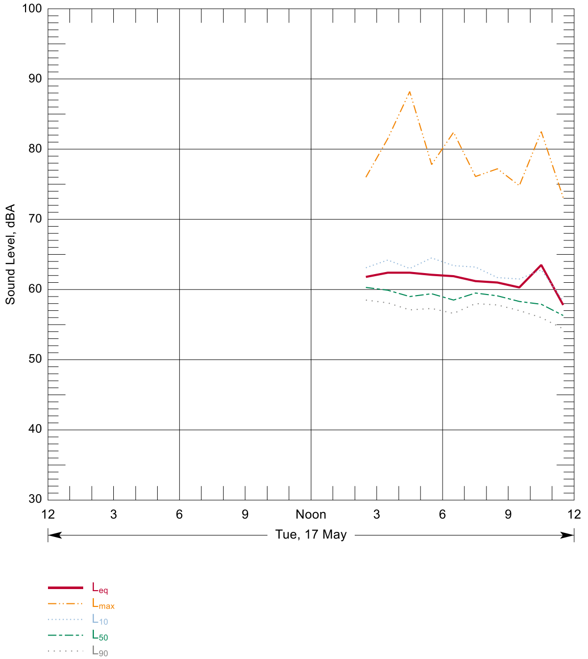
Figure B-31: Hourly Summary of Noise Levels Measured at N83 on 17 May, 2016
