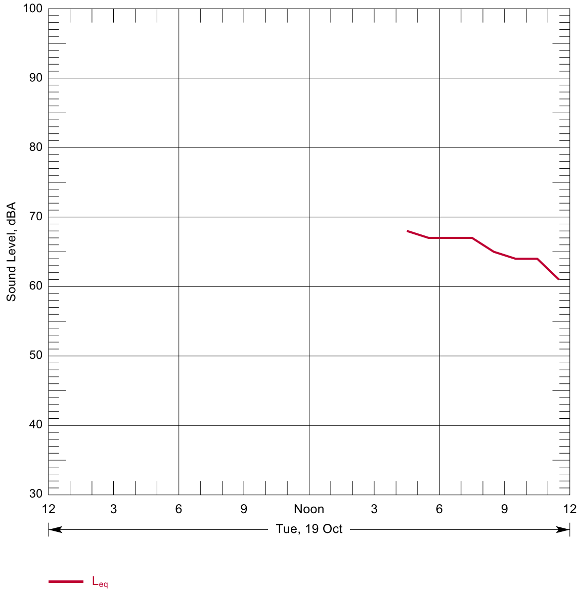
Figure B-106: Hourly Summary of Noise Levels Measured at N107 on 19 Oct, 2010
