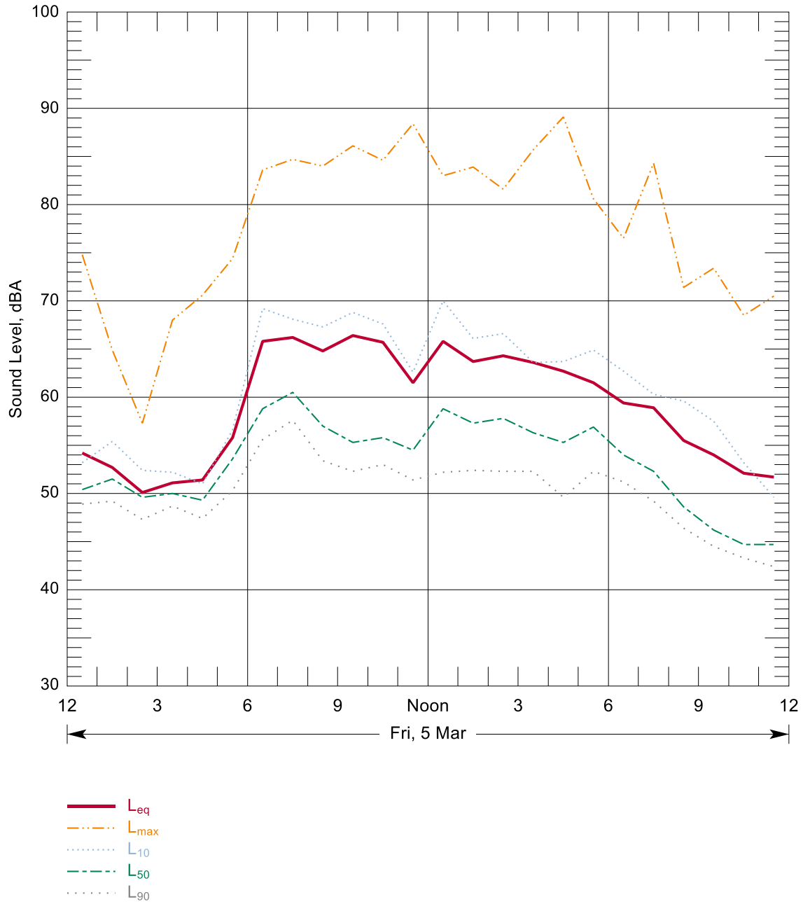
Figure B-12: Hourly Summary of Noise Levels Measured at N78 on 05 Mar, 2010
