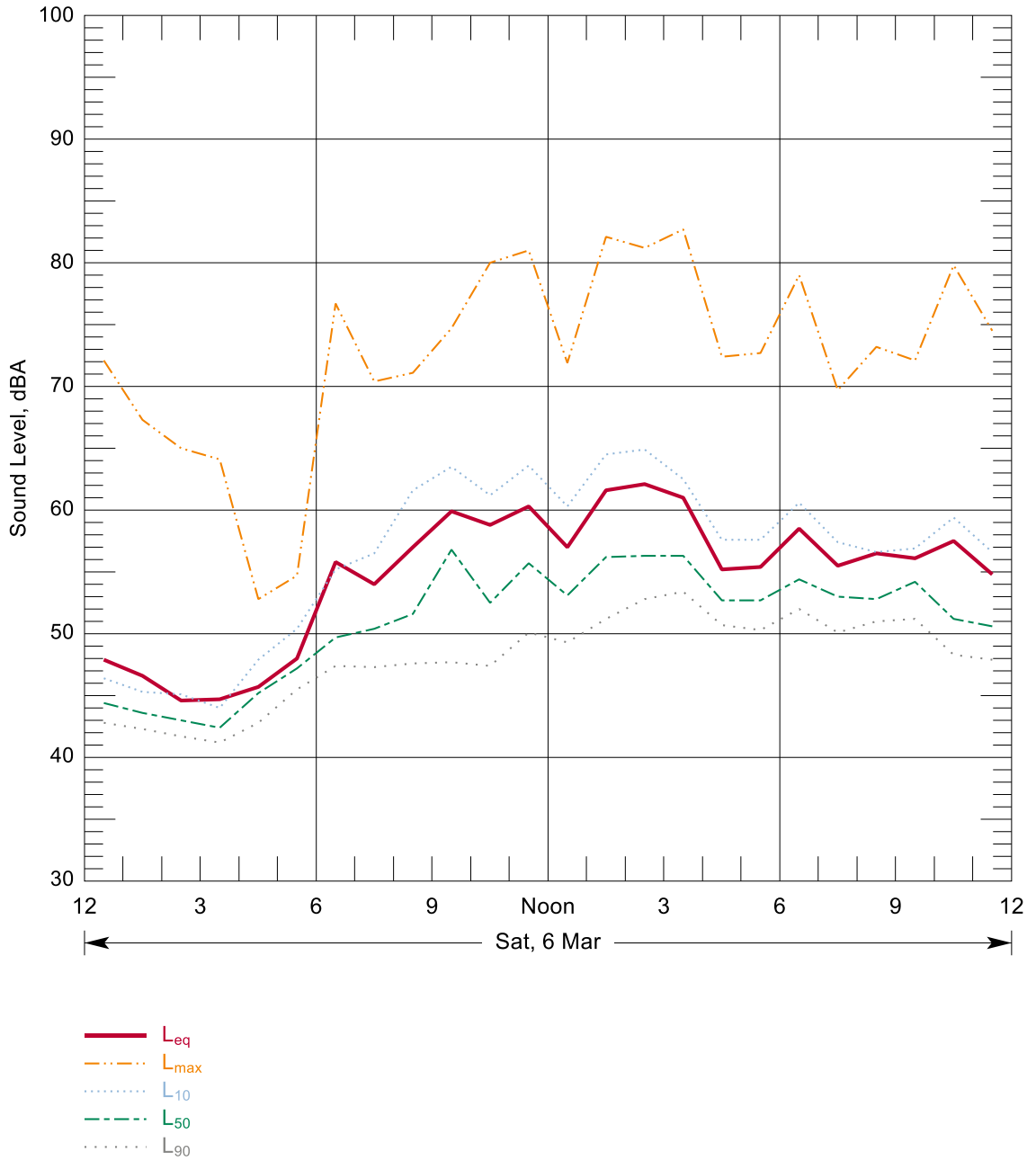
Figure B-13: Hourly Summary of Noise Levels Measured at N78 on 06 Mar, 2010
