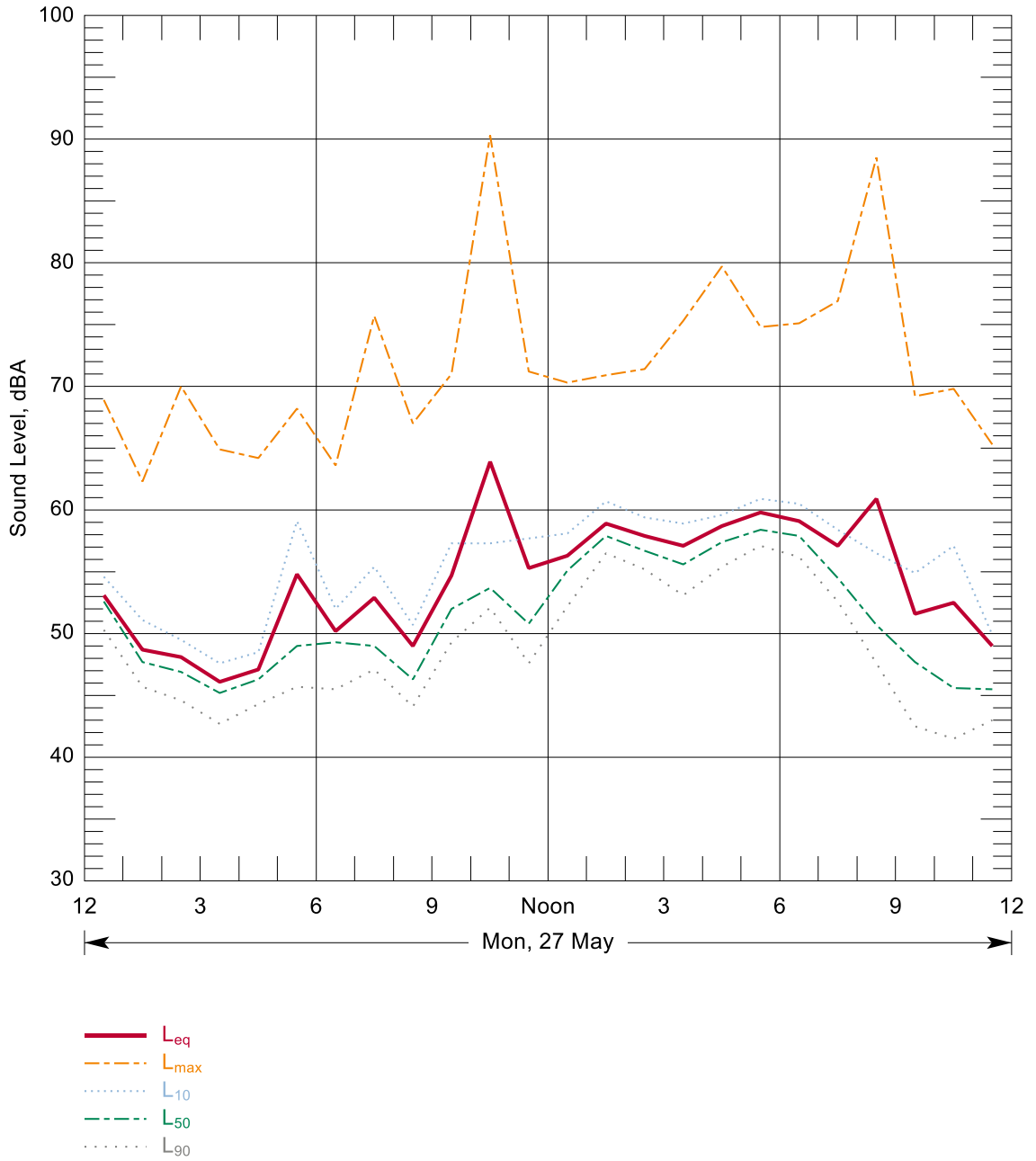
Figure B-225: Hourly Summary of Noise Levels Measured at N140 on 27 May, 2013
