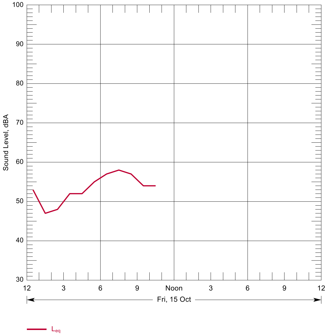
Figure B-75: Hourly Summary of Noise Levels Measured at N97 on 15 Oct, 2010
