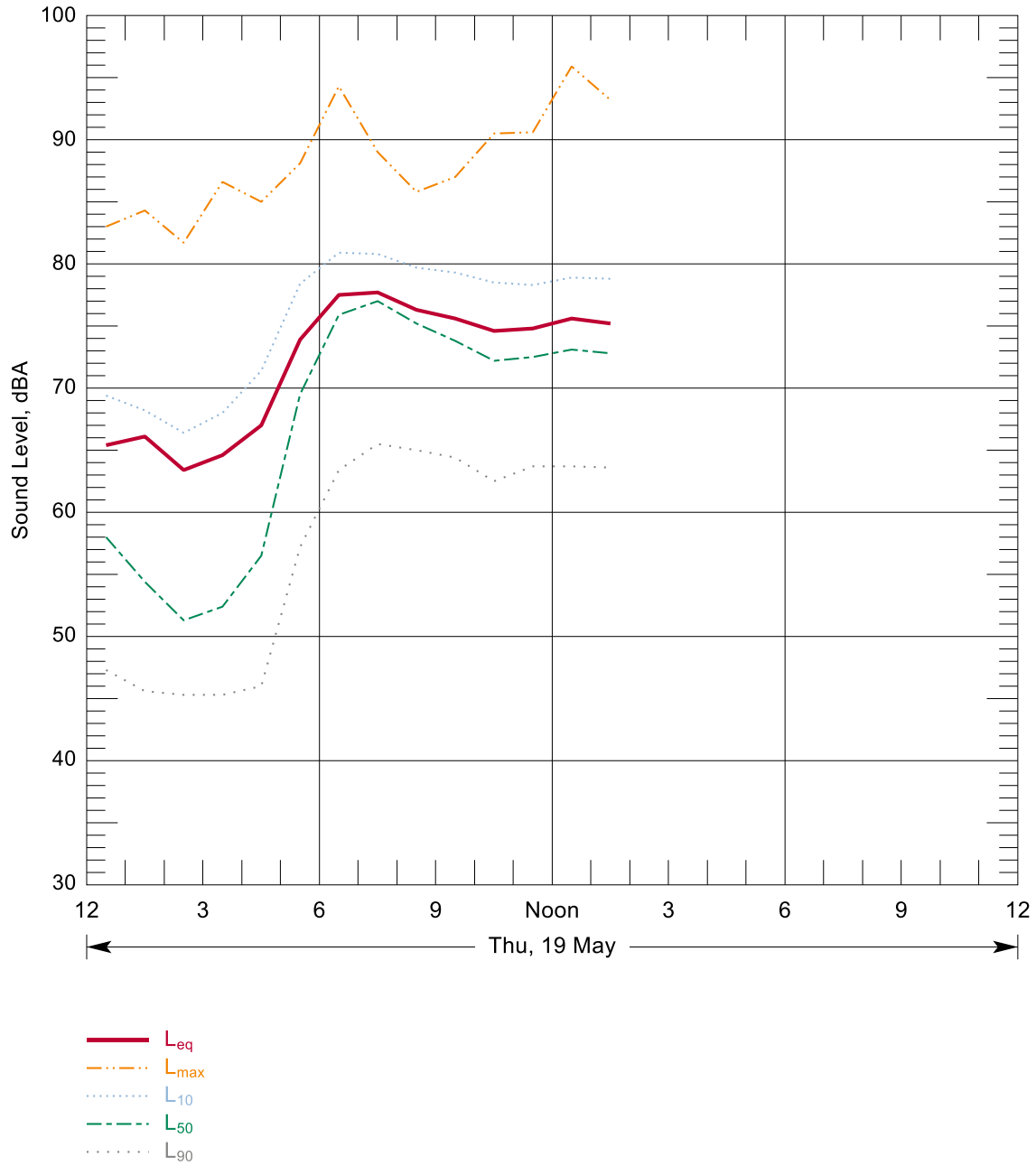
Figure B-44: Hourly Summary of Noise Levels Measured at N87 on 19 May, 2016
