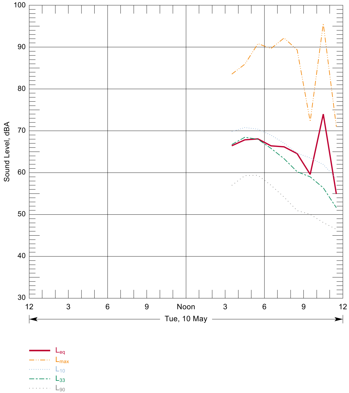
Figure B-70: Hourly Summary of Noise Levels Measured at N96 on 10 May, 2016
