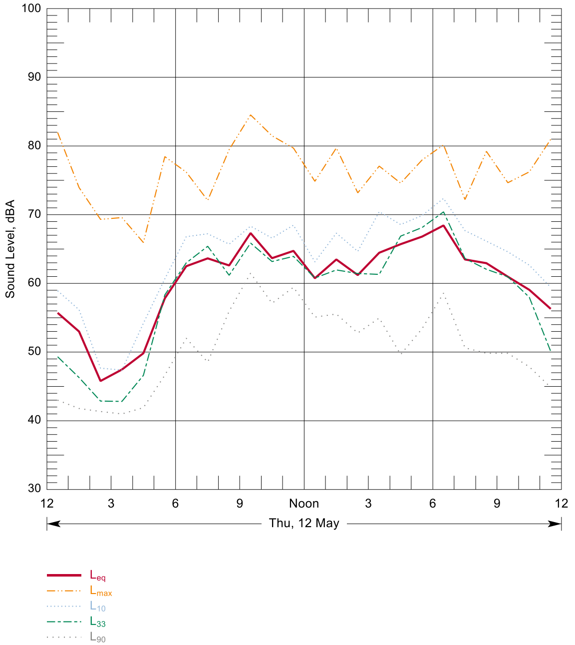
Figure B-19: Hourly Summary of Noise Levels Measured at N79 on 12 May, 2016
