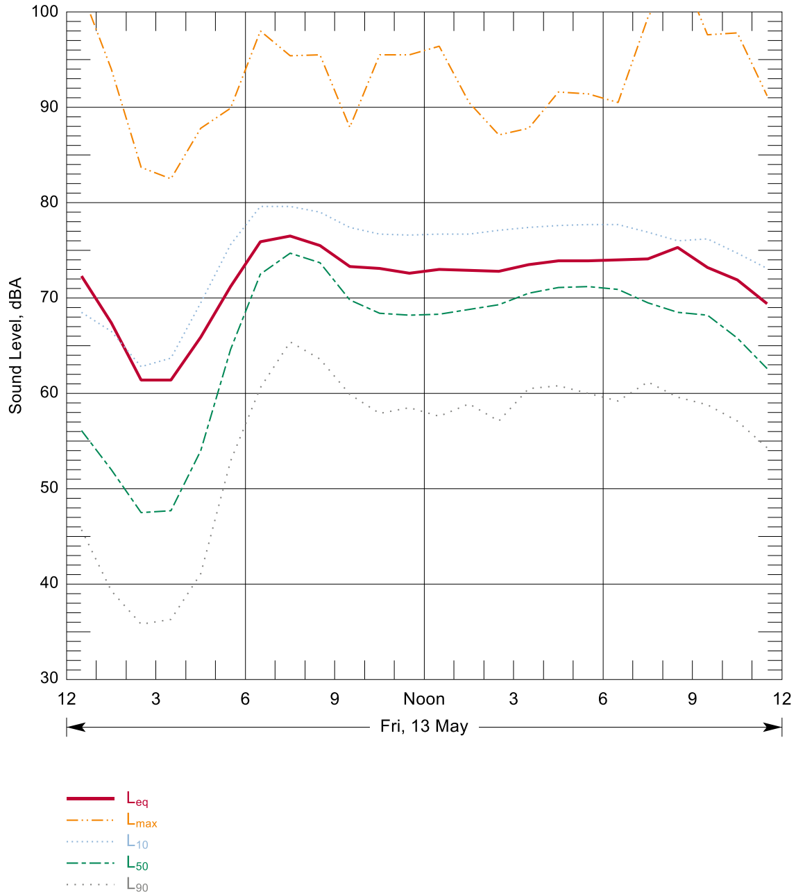
Figure B-50: Hourly Summary of Noise Levels Measured at N90 on 13 May, 2016
