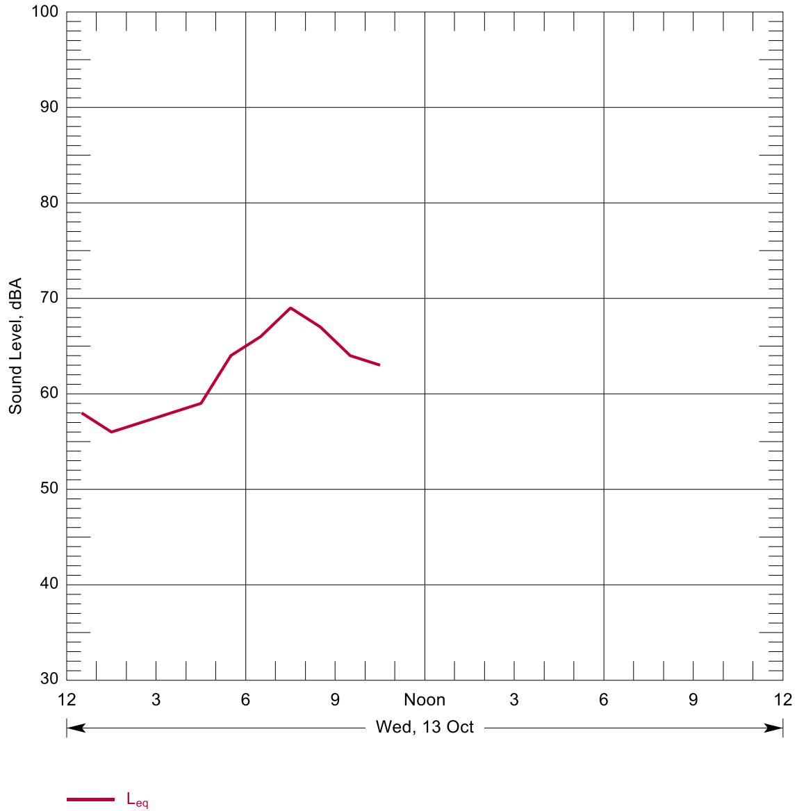
Figure B-22: Hourly Summary of Noise Levels Measured at N80 on 13 Oct, 2010
