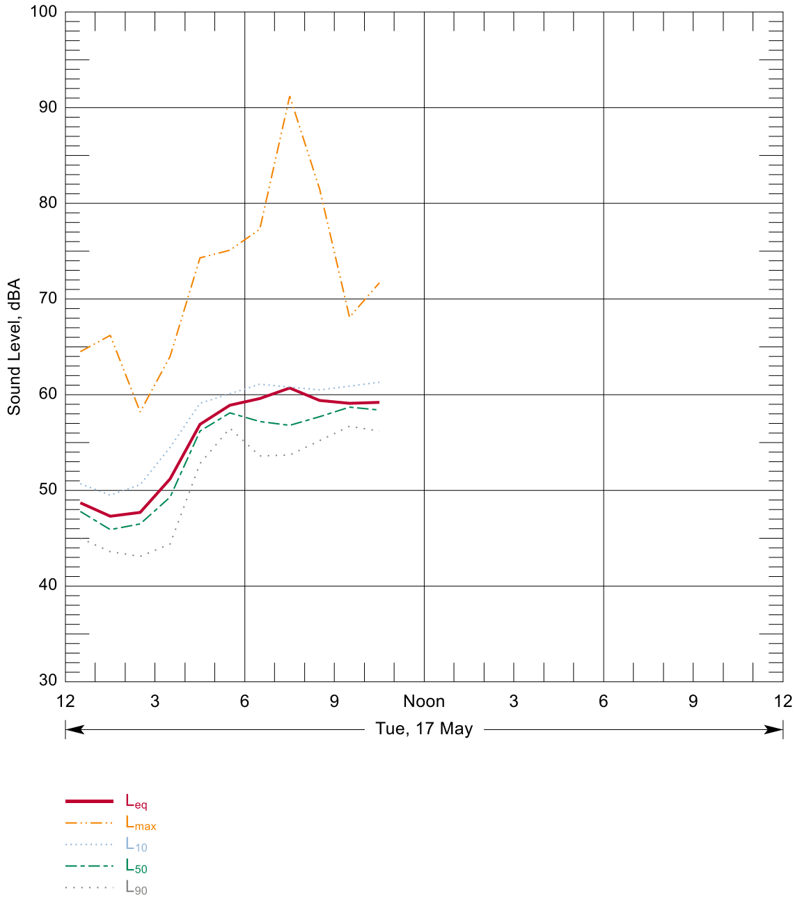
Figure B-103: Hourly Summary of Noise Levels Measured at N105 on 17 May, 2016
