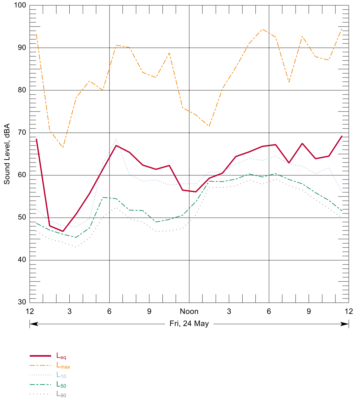
Figure B-224: Hourly Summary of Noise Levels Measured at N140 on 24 May, 2013
