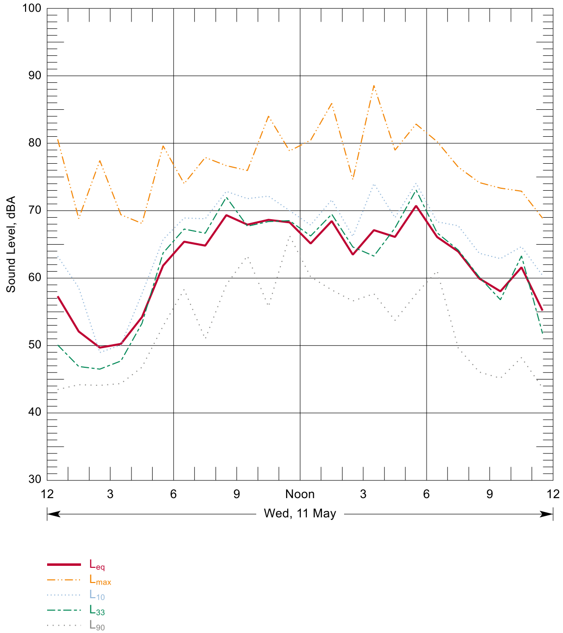
Figure B-18: Hourly Summary of Noise Levels Measured at N79 on 11 May, 2016
