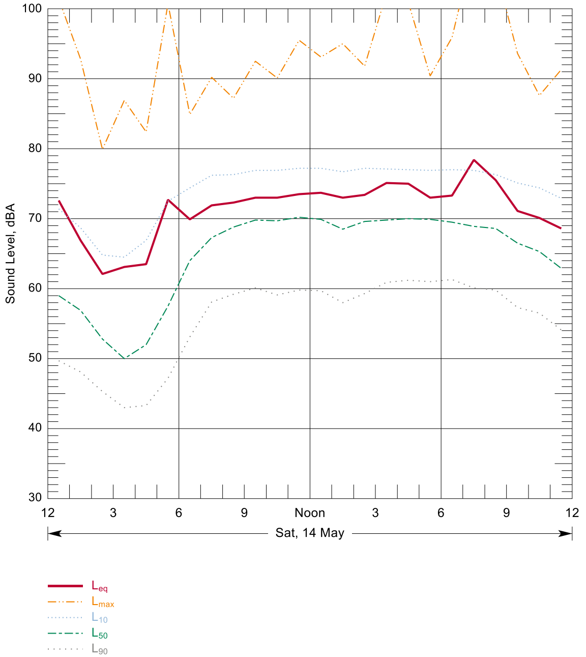
Figure B-51: Hourly Summary of Noise Levels Measured at N90 on 14 May, 2016
