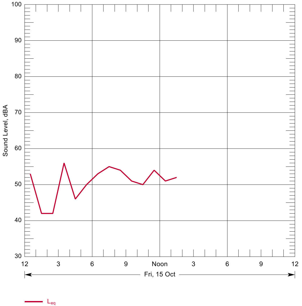
Figure B-69: Hourly Summary of Noise Levels Measured at N95 on 15 Oct, 2010
