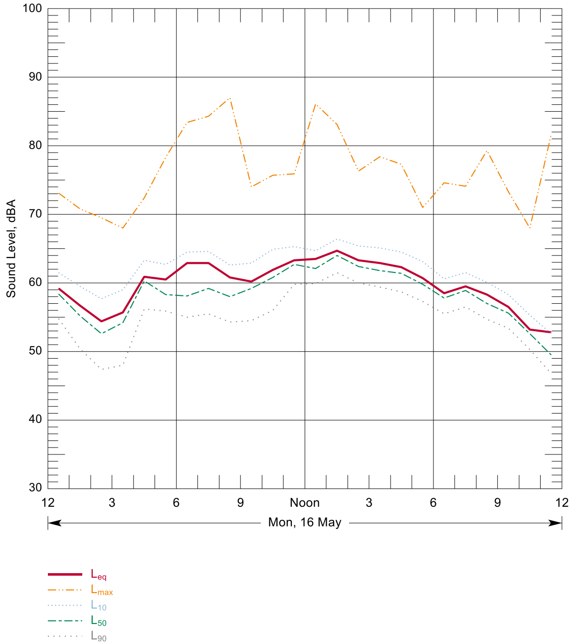
Figure B-102: Hourly Summary of Noise Levels Measured at N105 on 16 May, 2016
