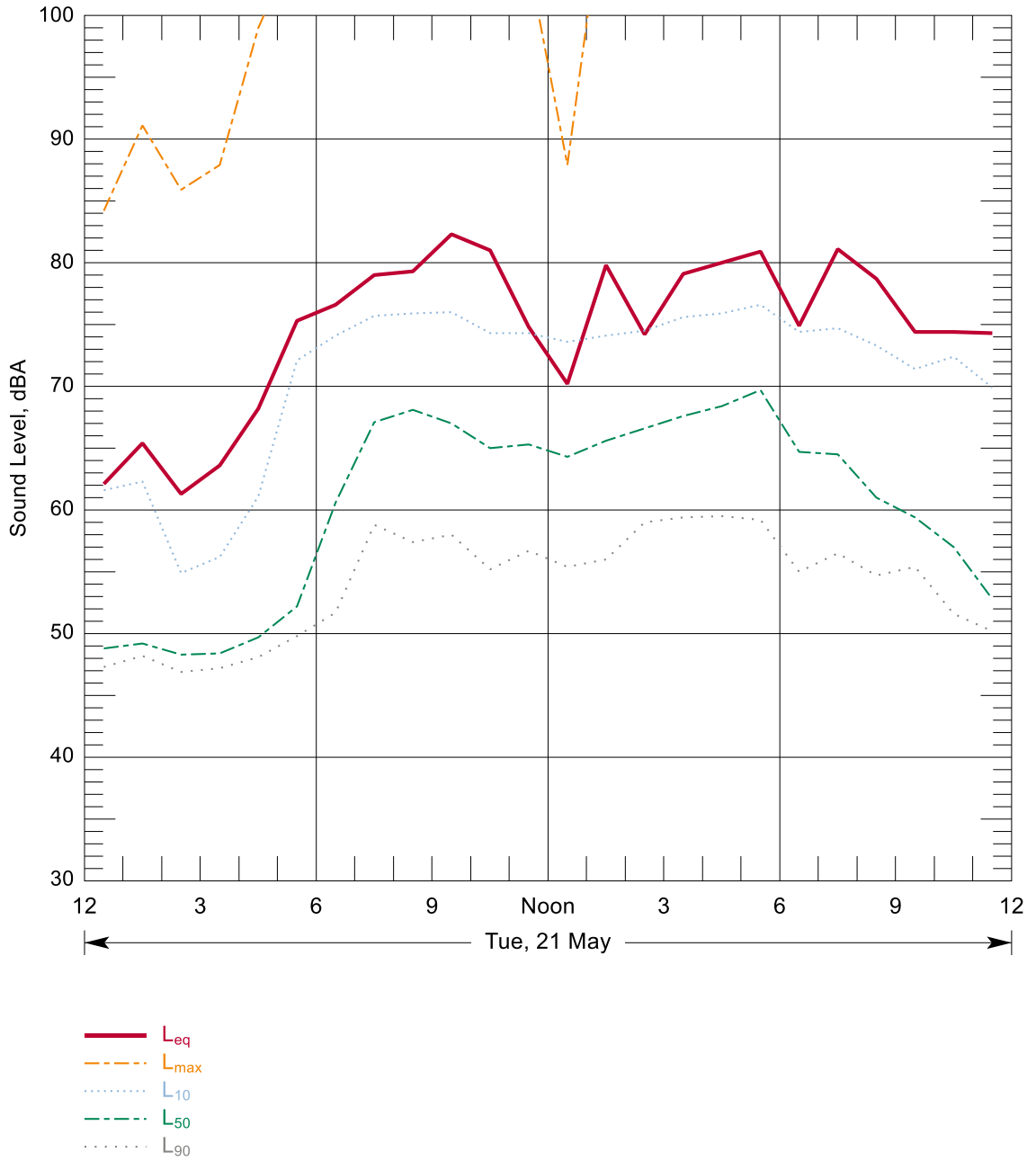
Figure B-215: Hourly Summary of Noise Levels Measured at N139 on 21 May, 2013
