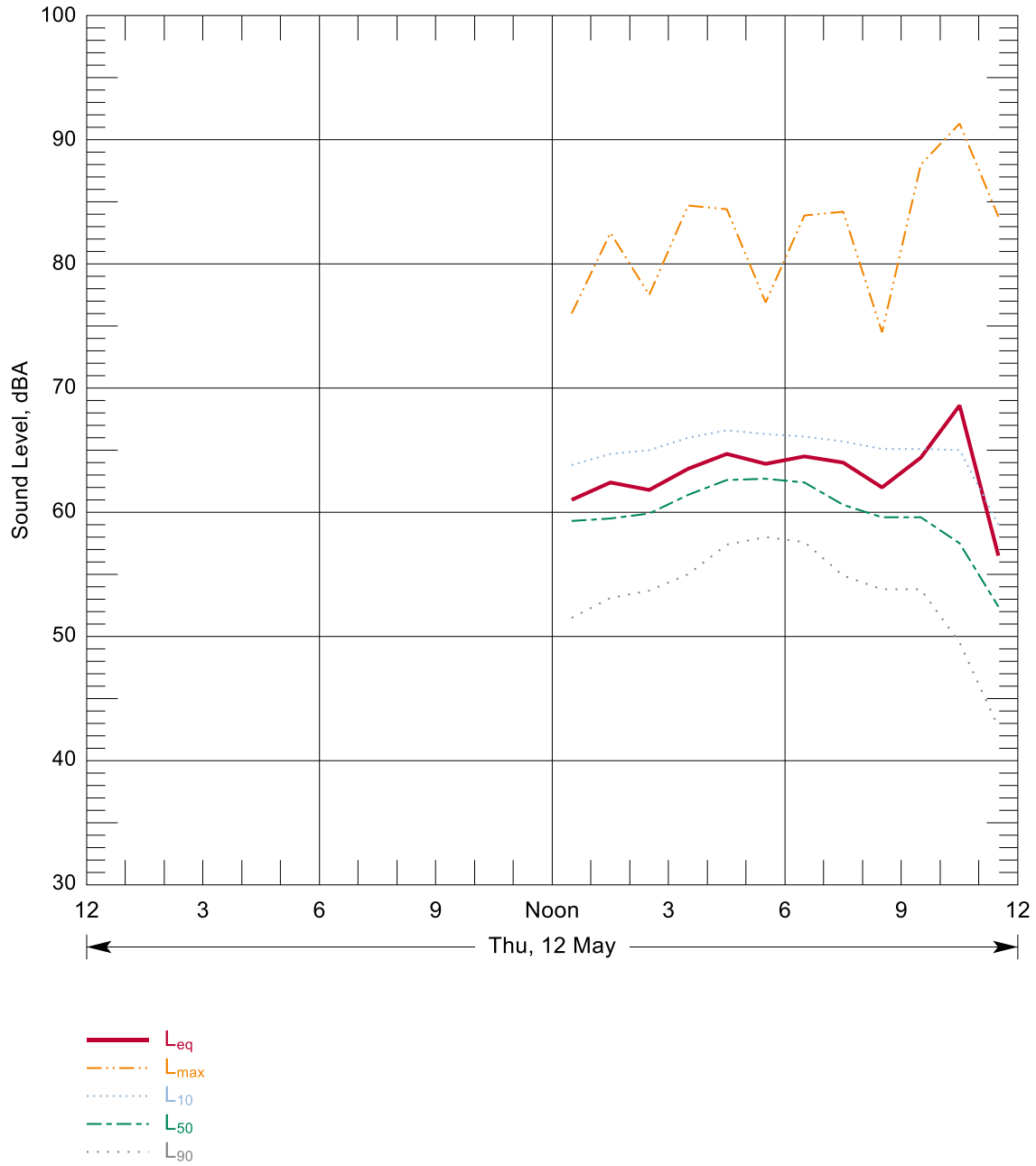
Figure B-54: Hourly Summary of Noise Levels Measured at N91 on 12 May, 2016
