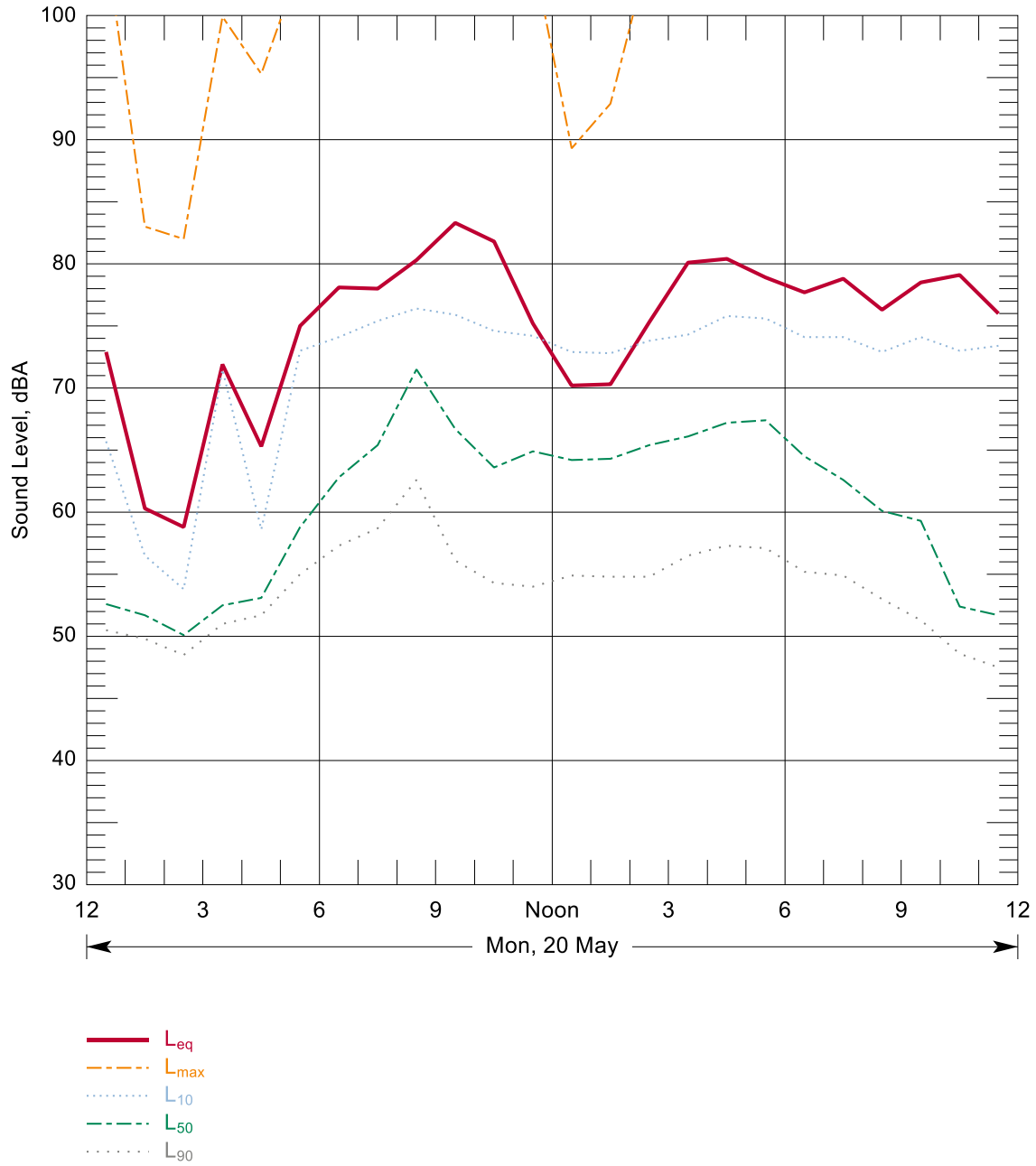
Figure B-214: Hourly Summary of Noise Levels Measured at N139 on 20 May, 2013
