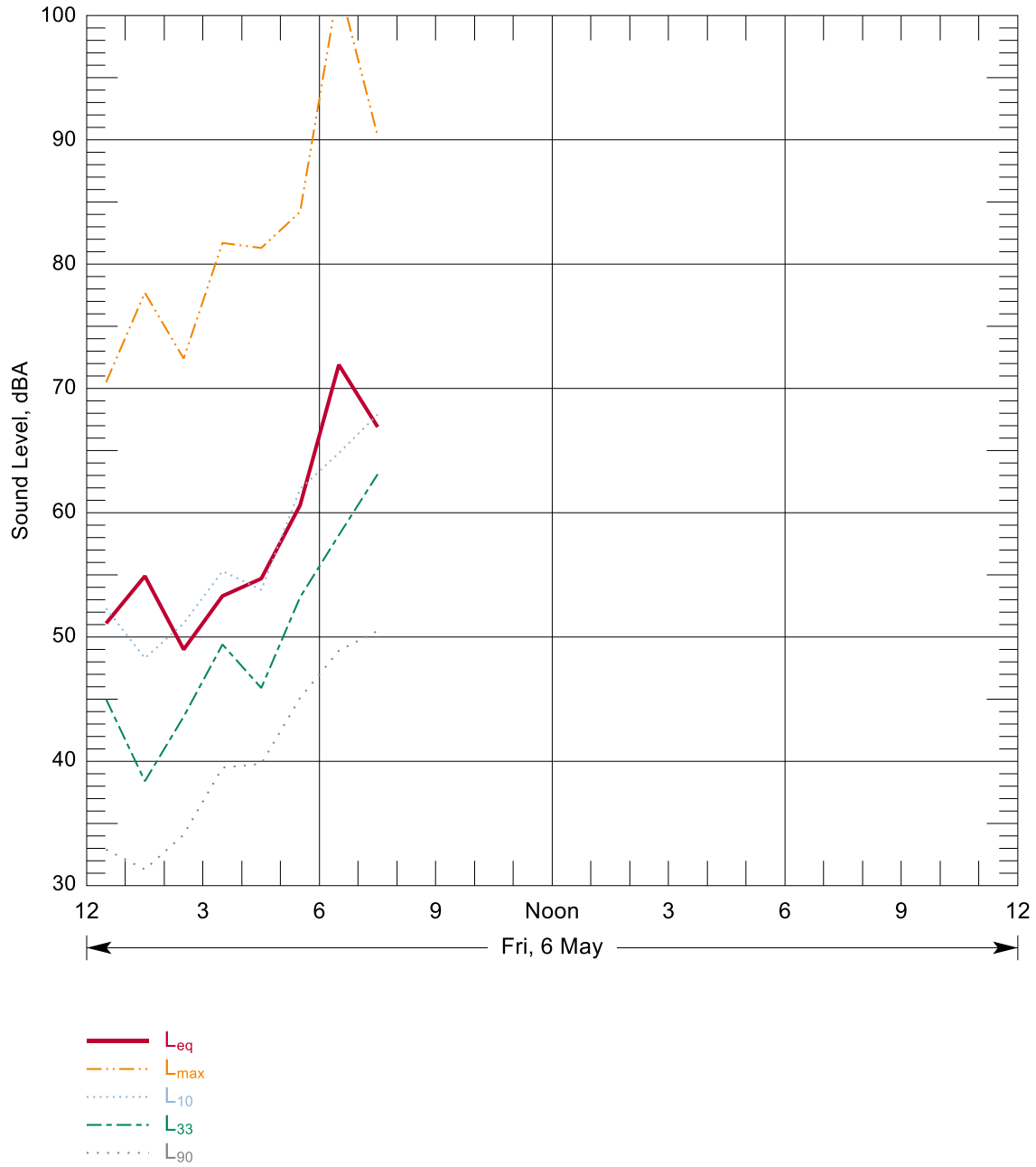
Figure B-98: Hourly Summary of Noise Levels Measured at N104 on 06 May, 2016
