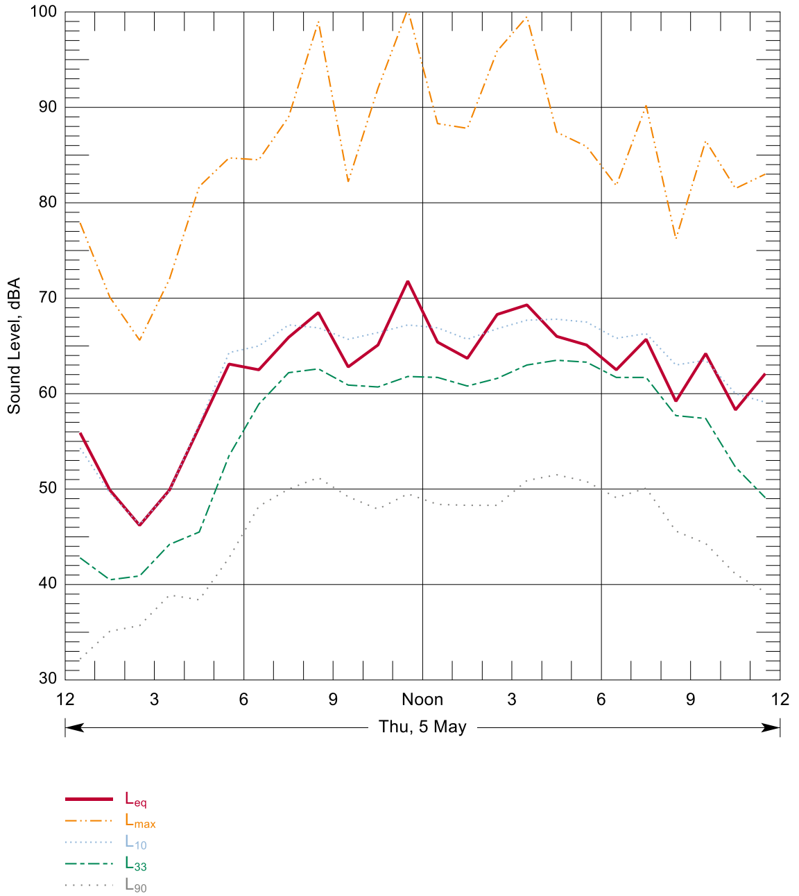
Figure B-97: Hourly Summary of Noise Levels Measured at N104 on 05 May, 2016
