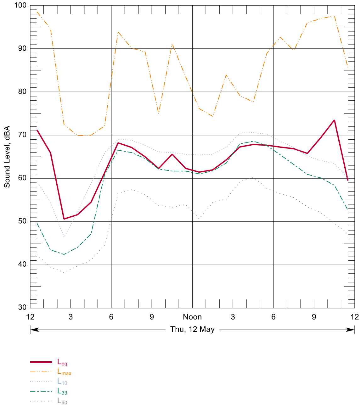
Figure B-72: Hourly Summary of Noise Levels Measured at N96 on 12 May, 2016
