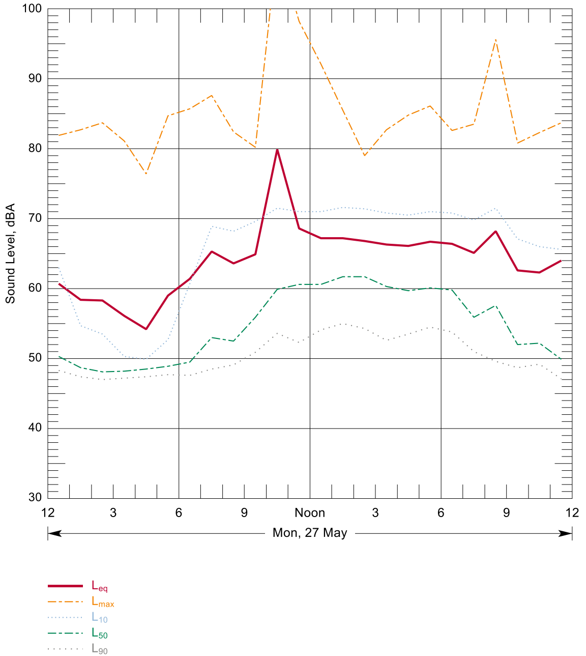
Figure B-219: Hourly Summary of Noise Levels Measured at N139 on 27 May, 2013
