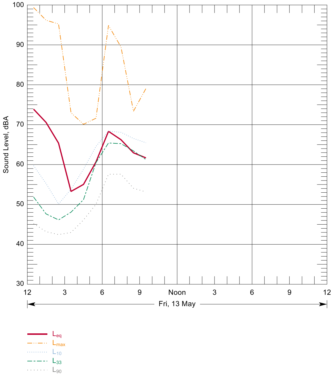
Figure B-73: Hourly Summary of Noise Levels Measured at N96 on 13 May, 2016
