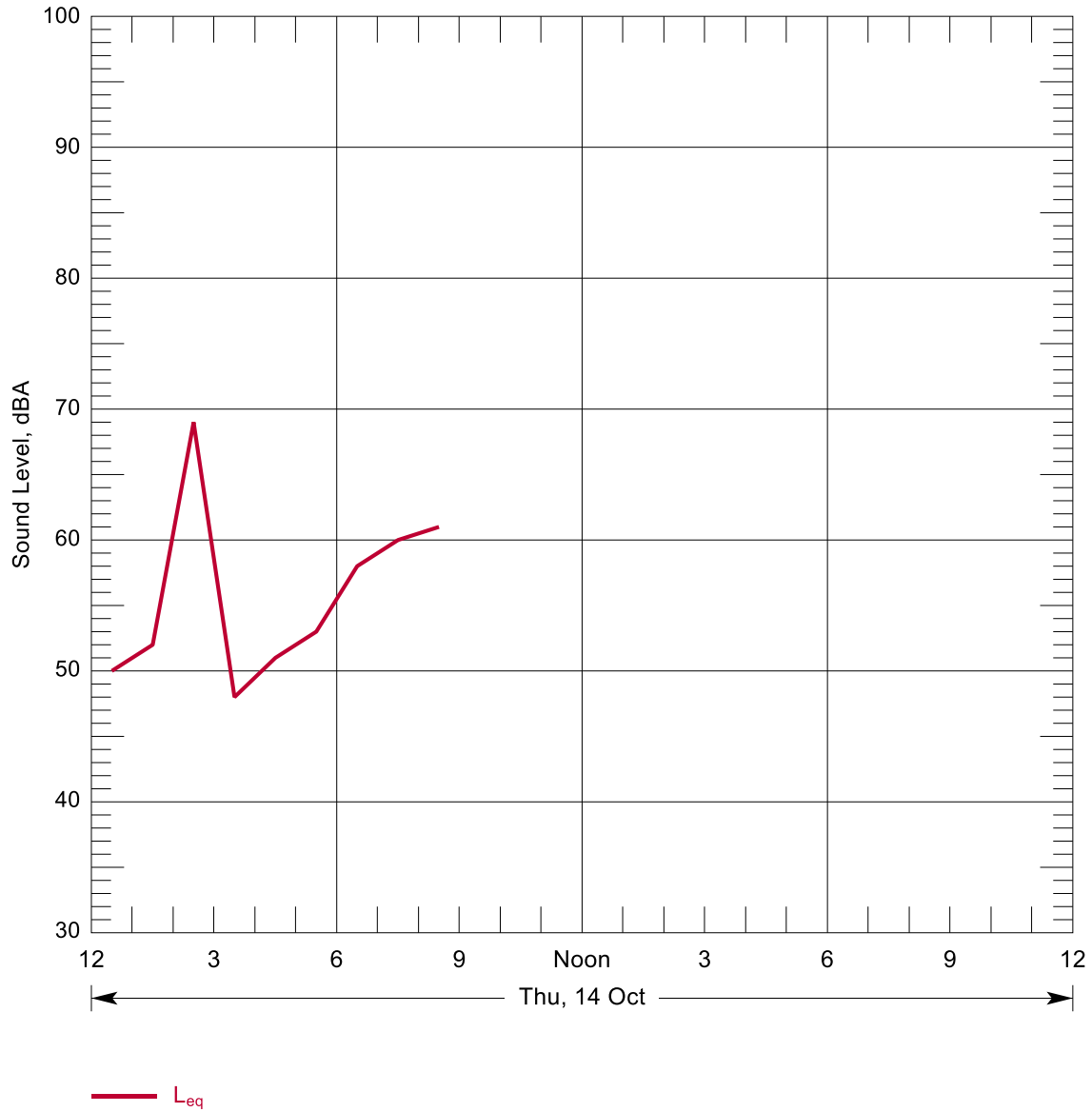
Figure B-46: Hourly Summary of Noise Levels Measured at N88 on 14 Oct, 2010
