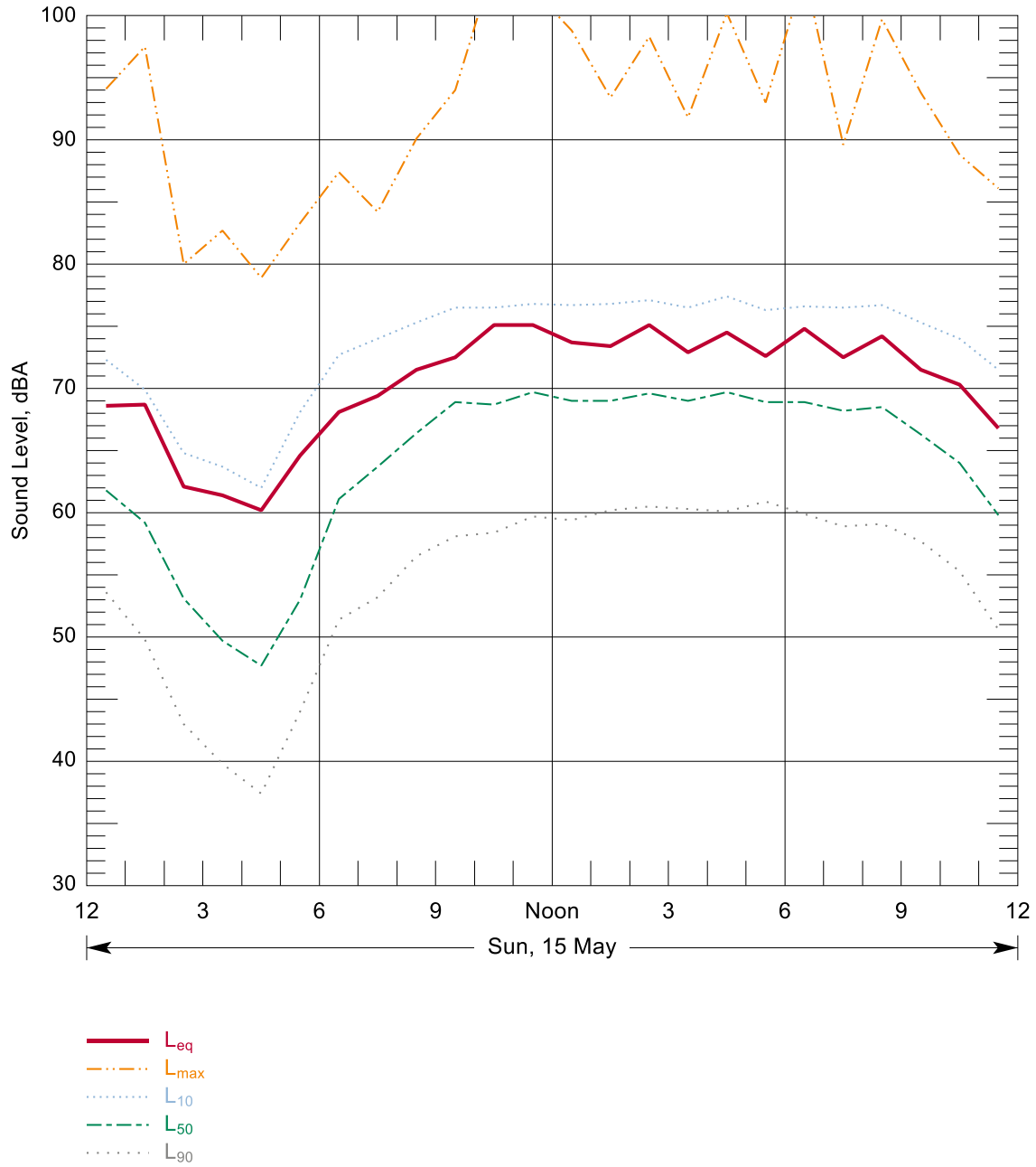
Figure B-52: Hourly Summary of Noise Levels Measured at N90 on 15 May, 2016
