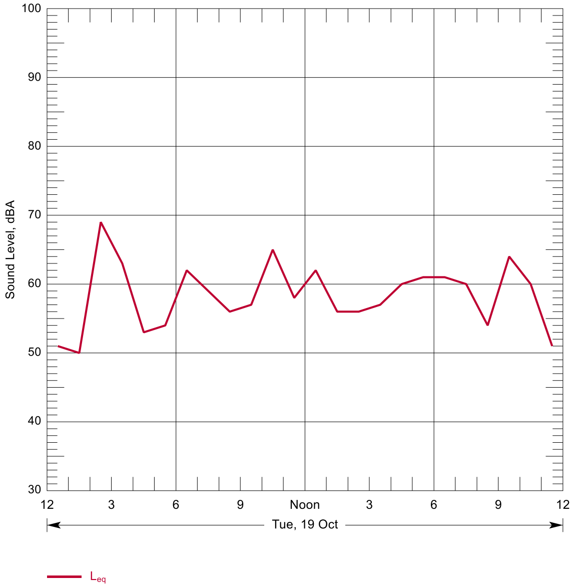
Figure B-109: Hourly Summary of Noise Levels Measured at N108 on 19 Oct, 2010
