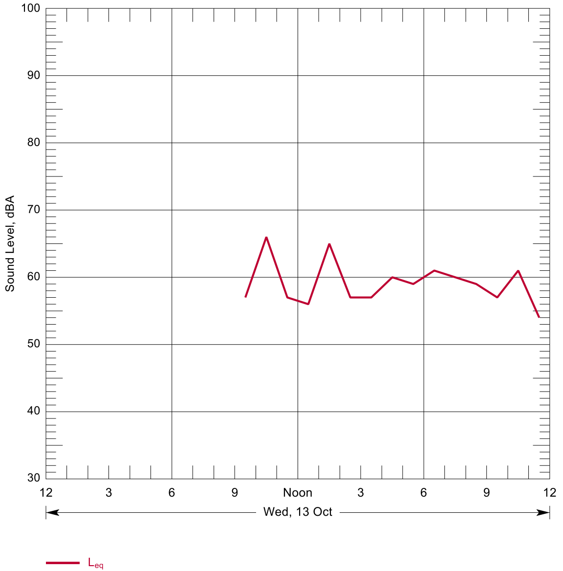
Figure B-45: Hourly Summary of Noise Levels Measured at N88 on 13 Oct, 2010
