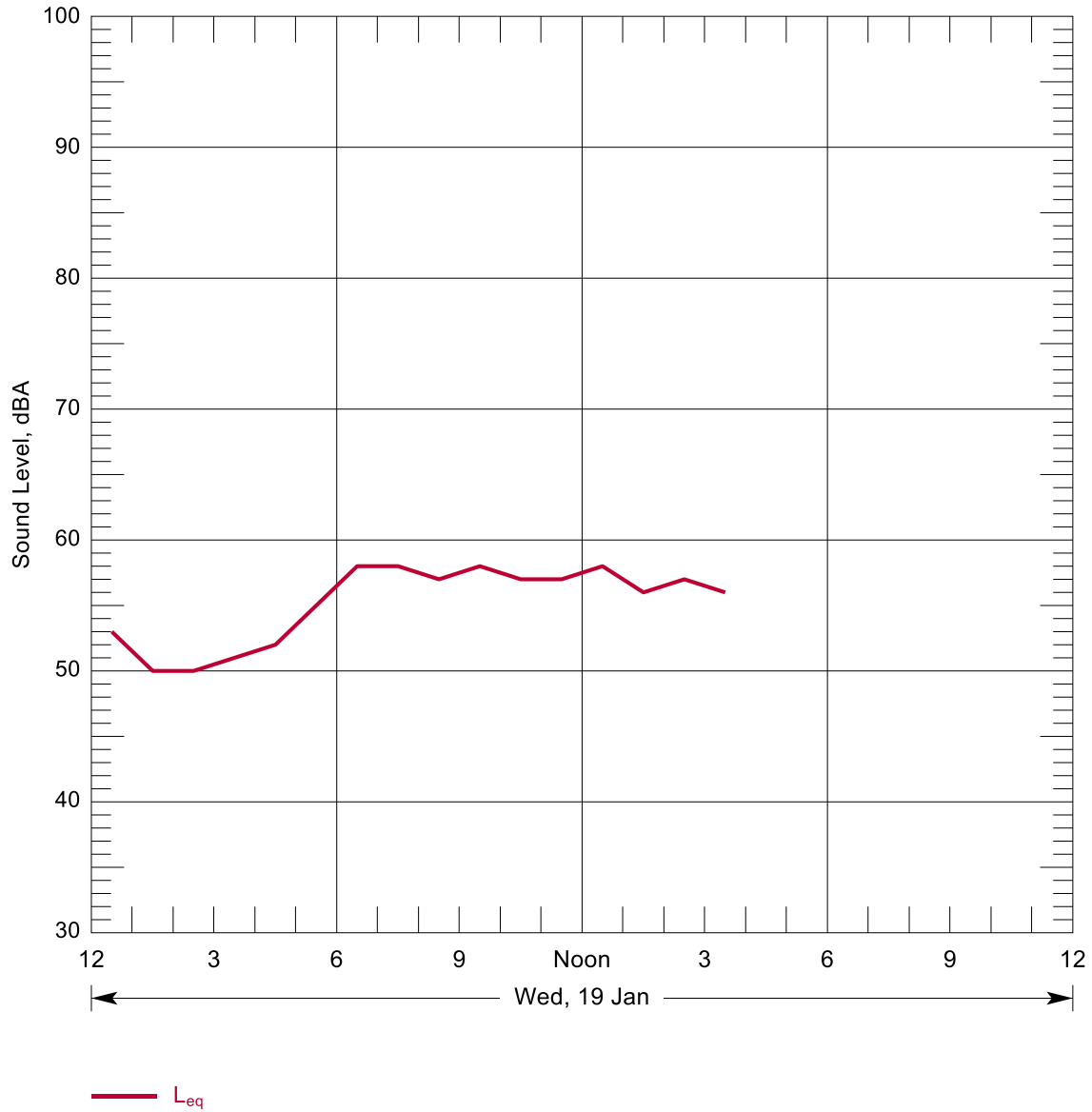
Figure B-80: Hourly Summary of Noise Levels Measured at N99 on 19 Jan, 2011
