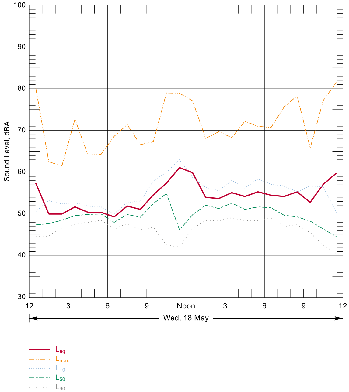
Figure B-40: Hourly Summary of Noise Levels Measured at N86 on 18 May, 2016
