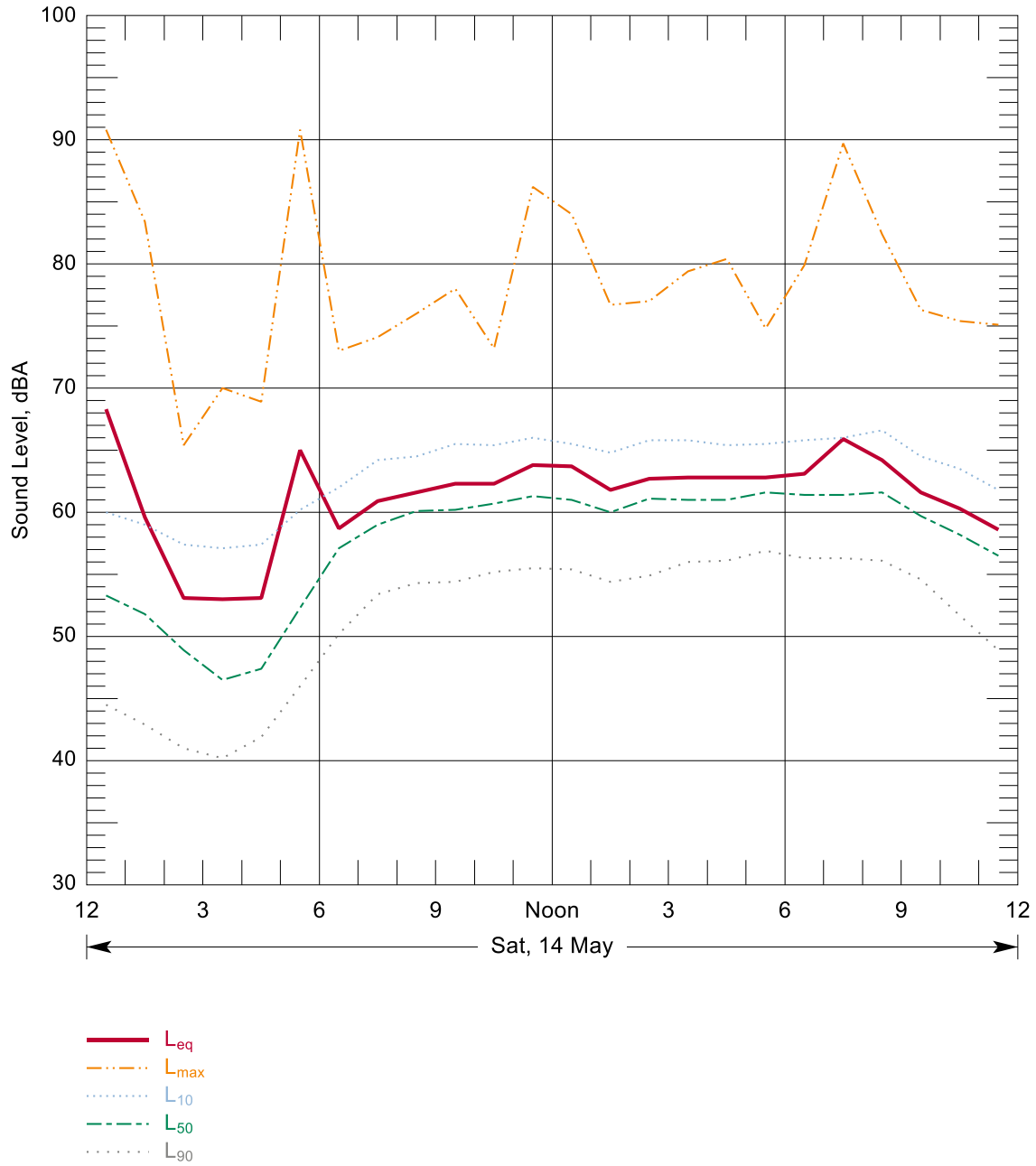
Figure B-56: Hourly Summary of Noise Levels Measured at N91 on 14 May, 2016
