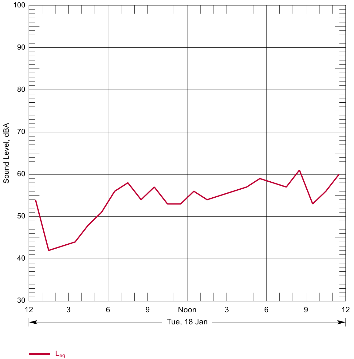
Figure B-77: Hourly Summary of Noise Levels Measured at N98 on 18 Jan, 2011
