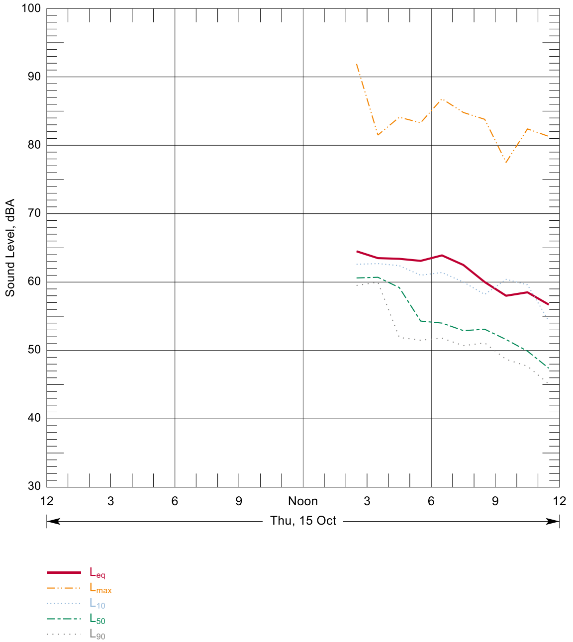
Figure B-5: Hourly Summary of Noise Levels Measured at N77 on 15 Oct, 2009
