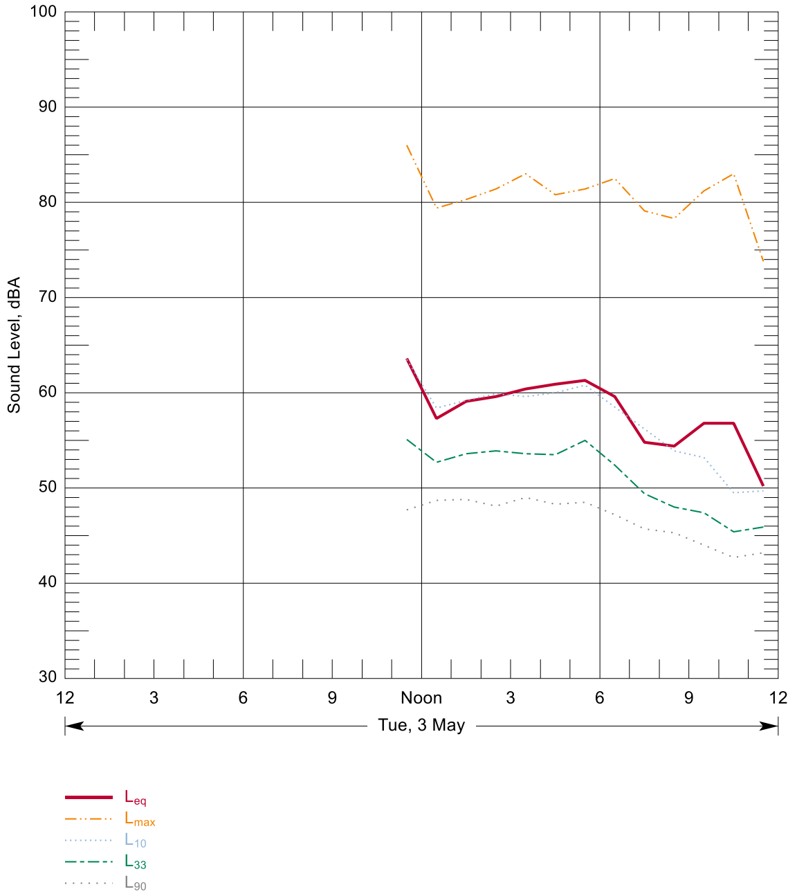
Figure B-1: Hourly Summary of Noise Levels Measured at N76 on 03 May, 2016
