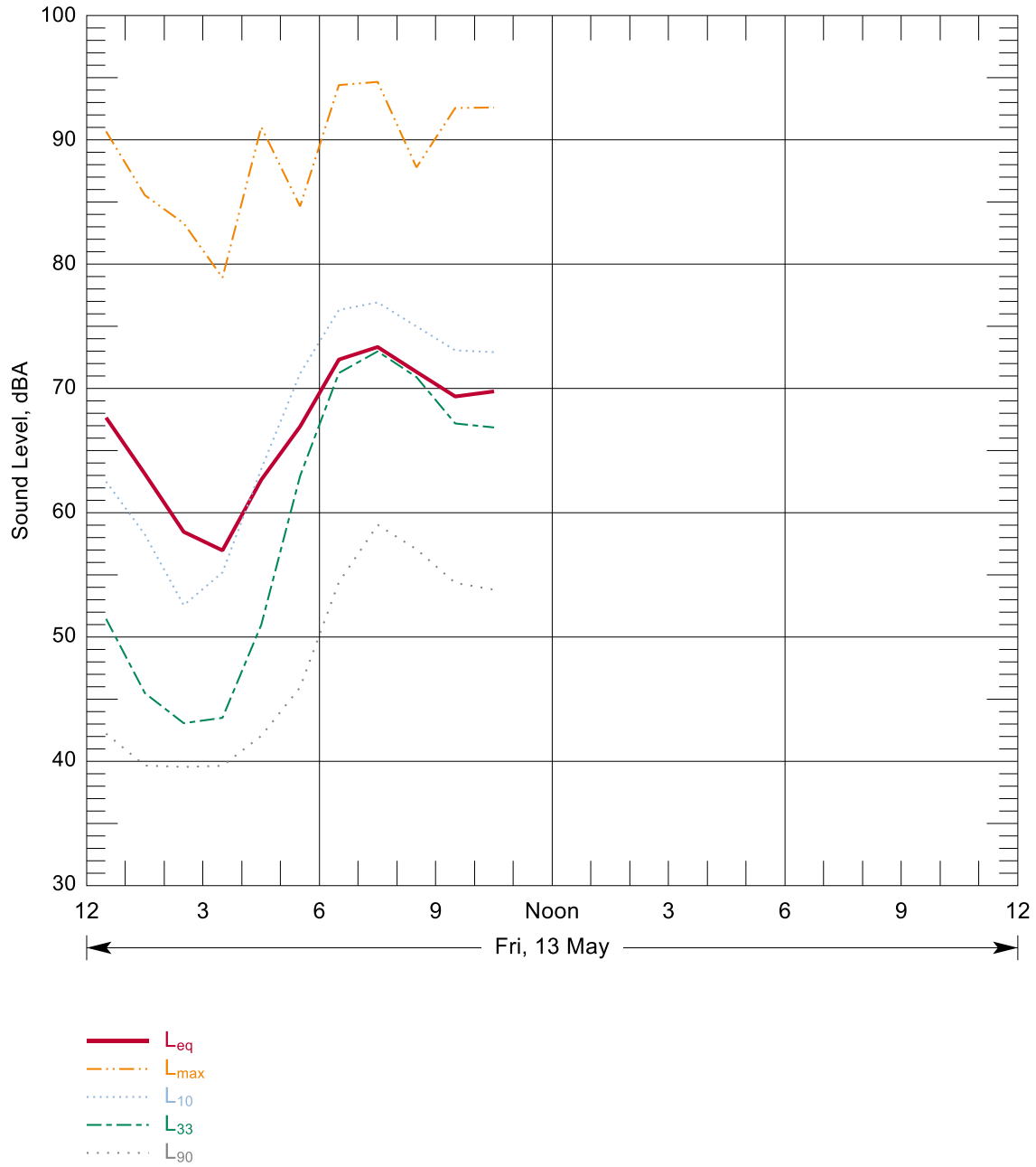
Figure B-64: Hourly Summary of Noise Levels Measured at N93 on 13 May, 2016
