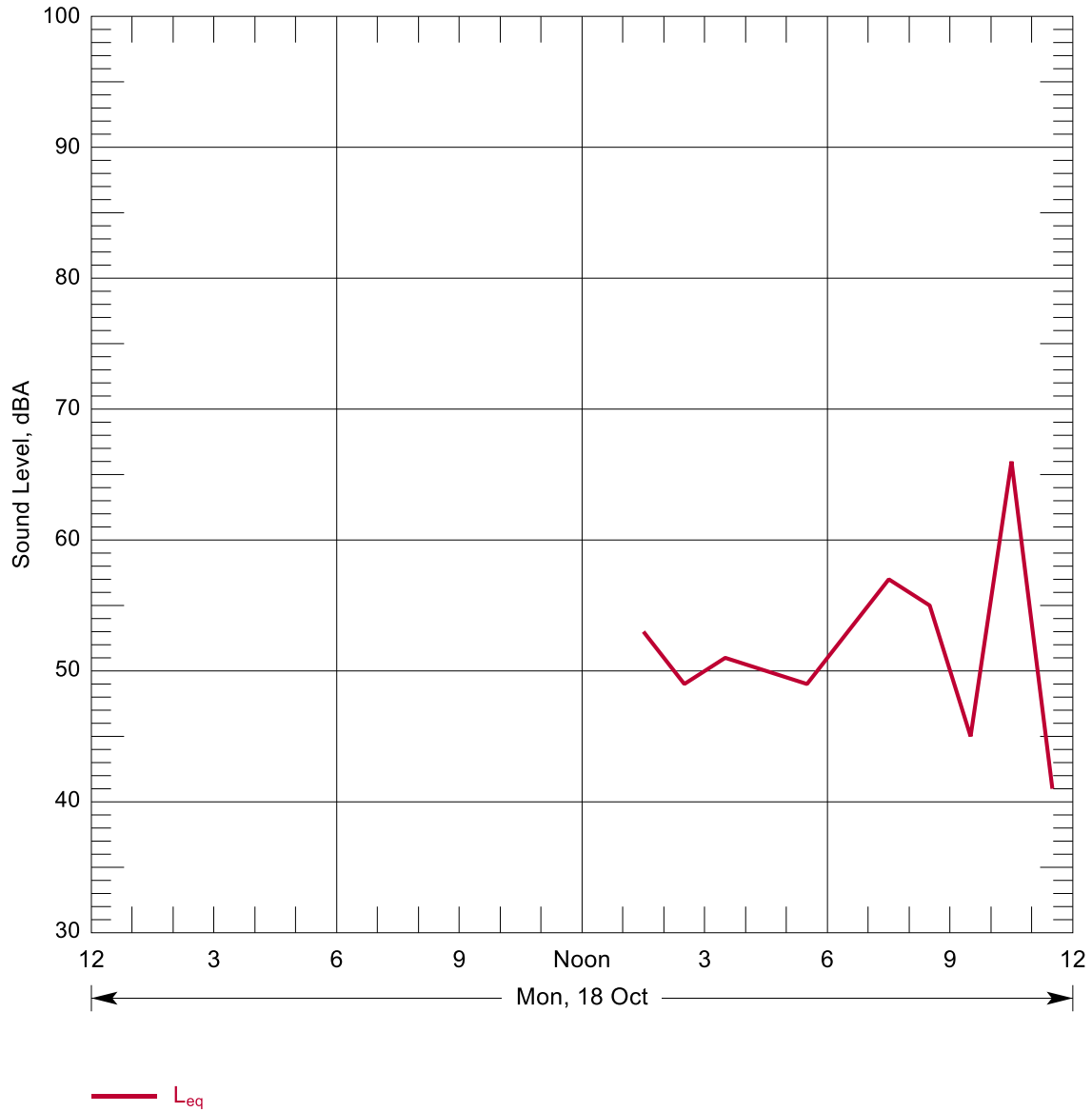
Figure B-104: Hourly Summary of Noise Levels Measured at N106 on 18 Oct, 2010
