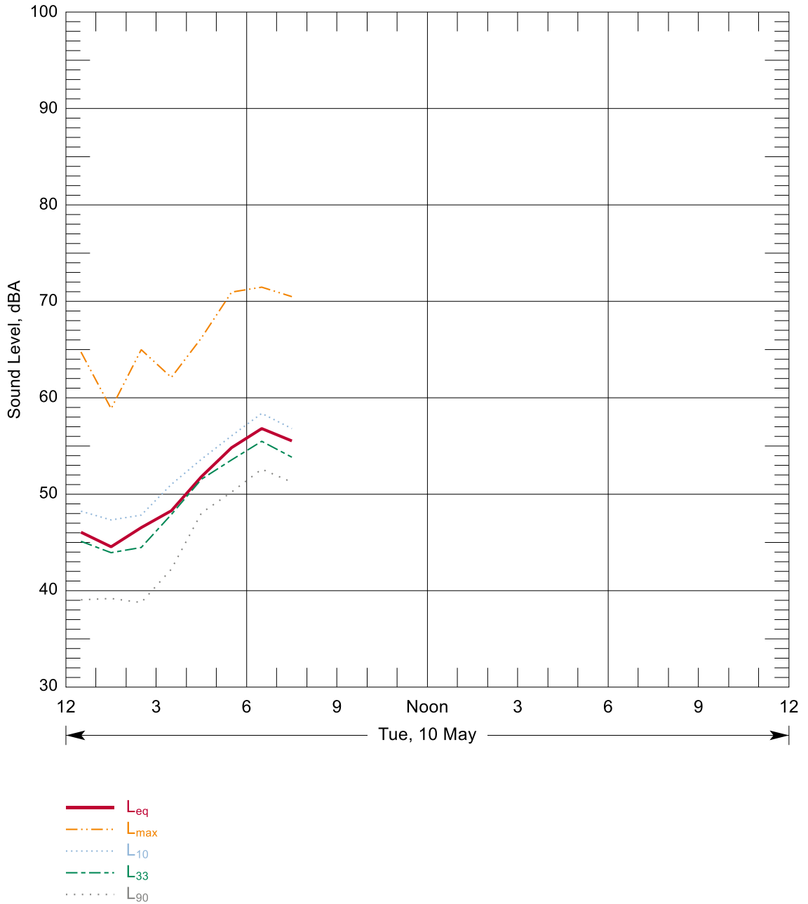
Figure B-27: Hourly Summary of Noise Levels Measured at N81 on 10 May, 2016
