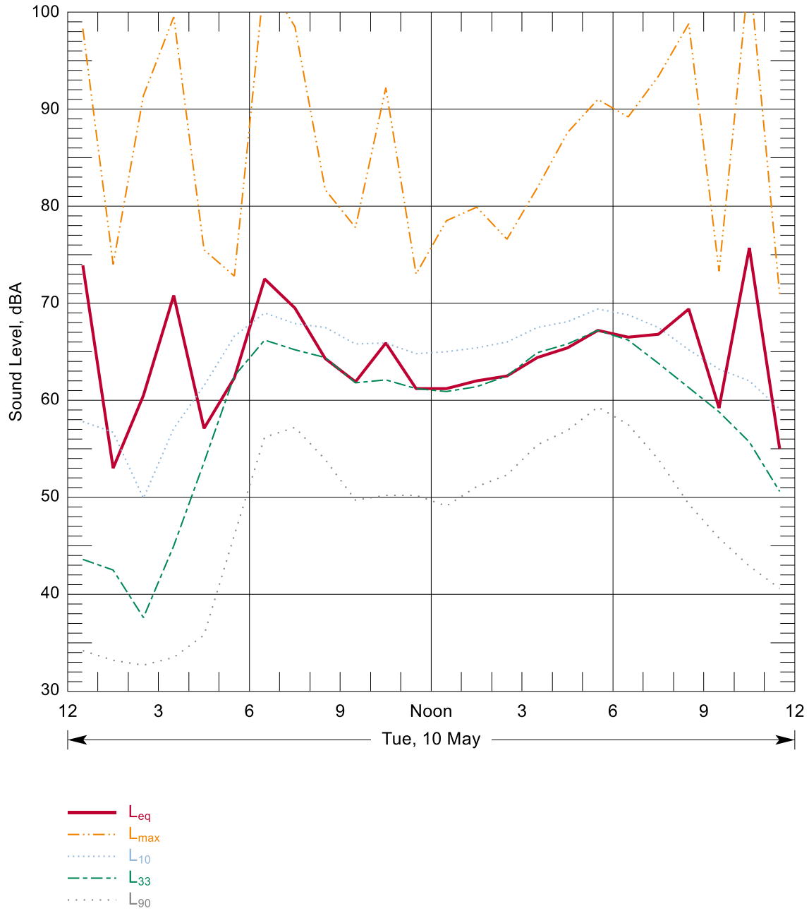
Figure B-86: Hourly Summary of Noise Levels Measured at N101 on 10 May, 2016
