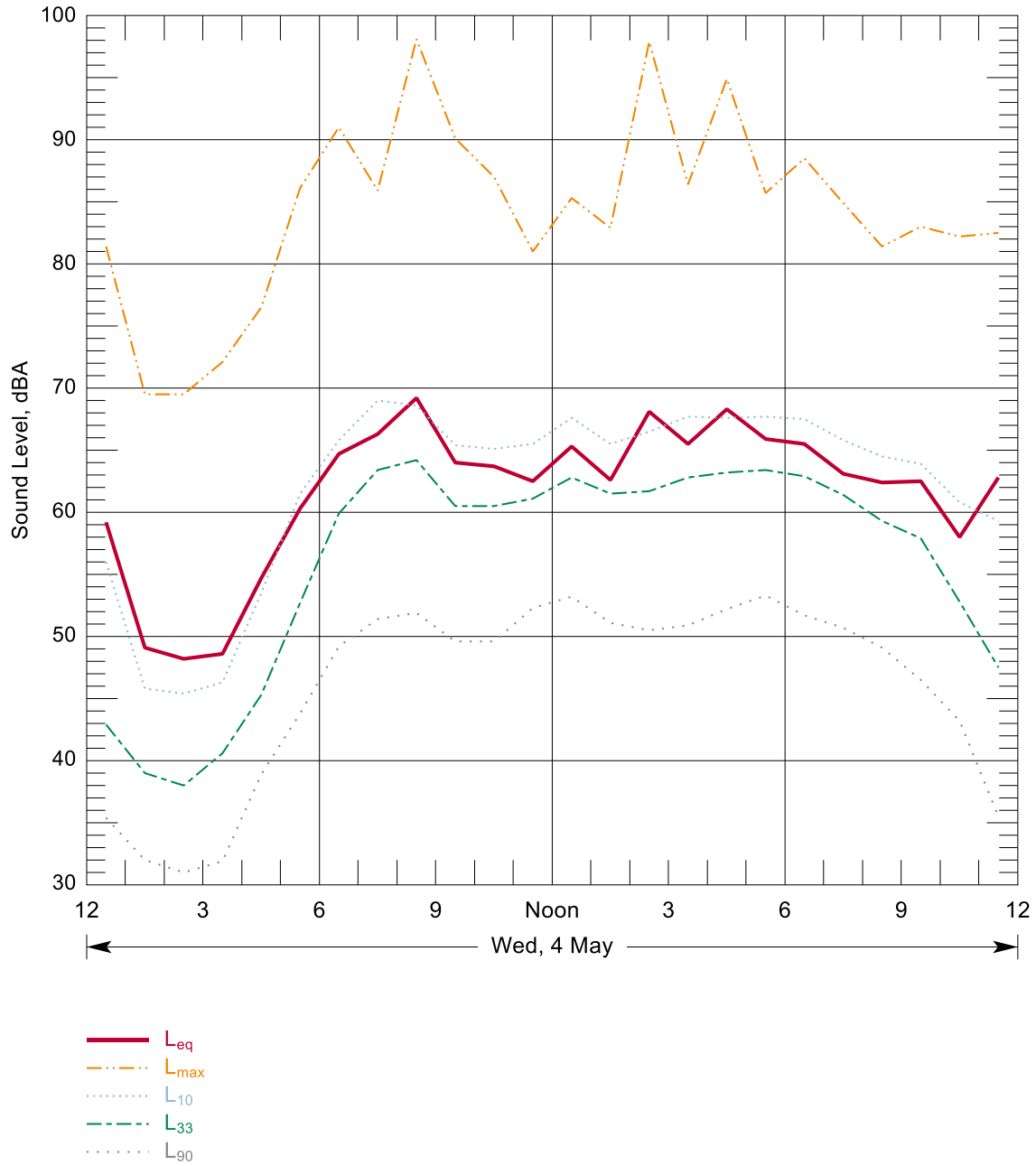
Figure B-96: Hourly Summary of Noise Levels Measured at N104 on 04 May, 2016
