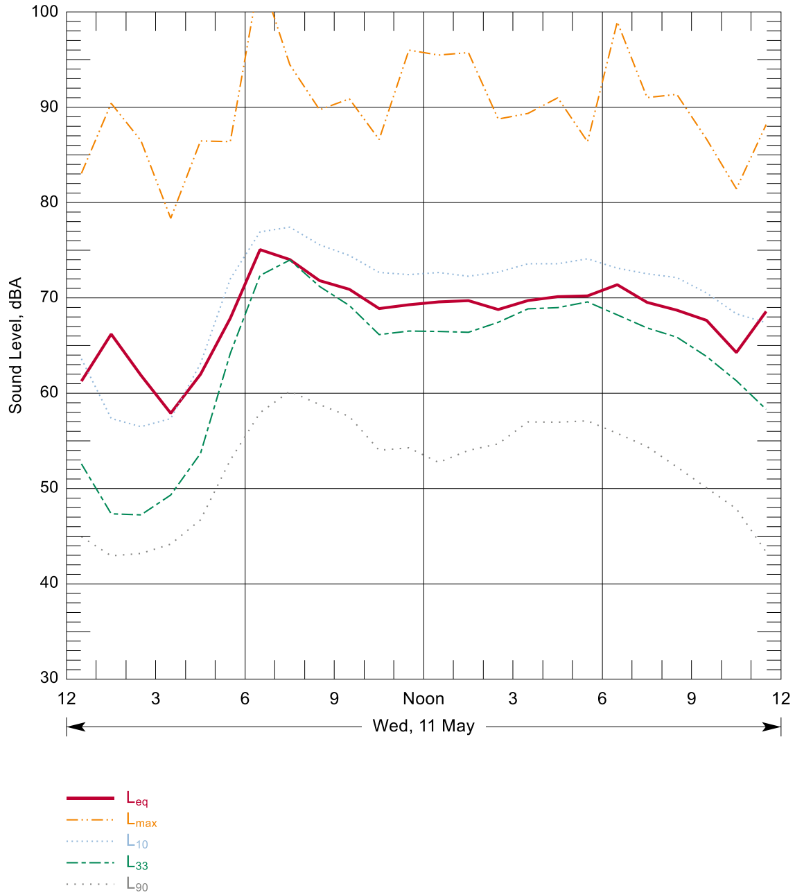
Figure B-62: Hourly Summary of Noise Levels Measured at N93 on 11 May, 2016
