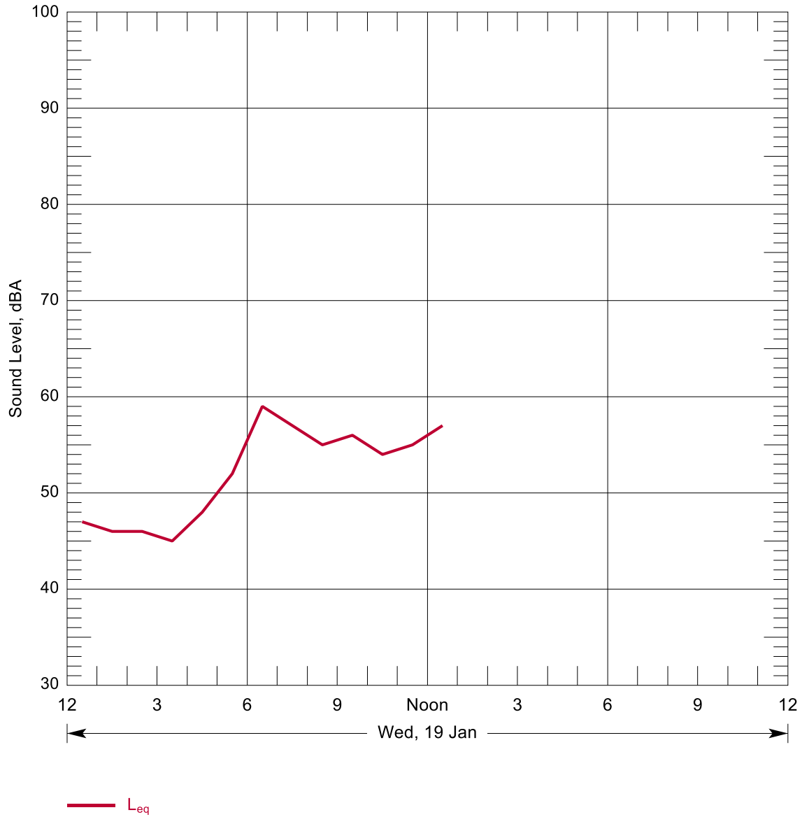
Figure B-78: Hourly Summary of Noise Levels Measured at N98 on 19 Jan, 2011
