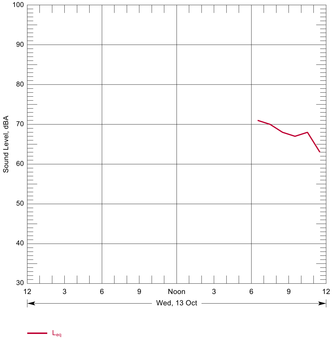
Figure B-65: Hourly Summary of Noise Levels Measured at N94 on 13 Oct, 2010
