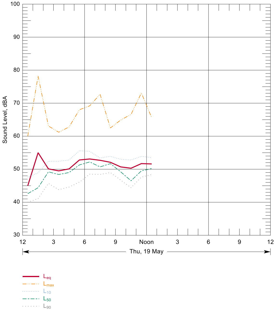
Figure B-41: Hourly Summary of Noise Levels Measured at N86 on 19 May, 2016
