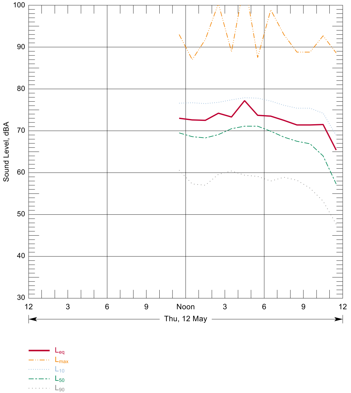
Figure B-49: Hourly Summary of Noise Levels Measured at N90 on 12 May, 2016
