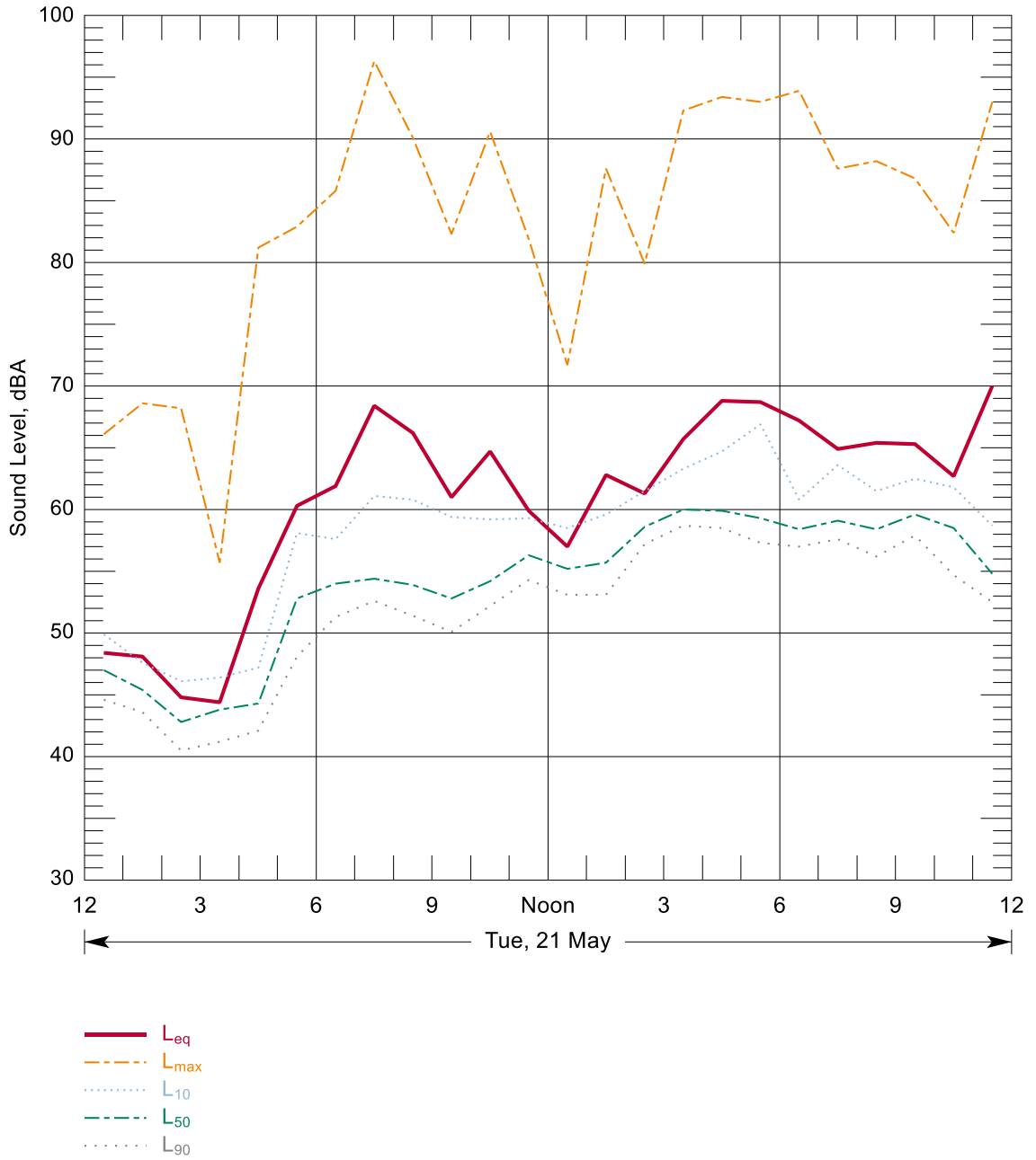
Figure B-221: Hourly Summary of Noise Levels Measured at N140 on 21 May, 2013
