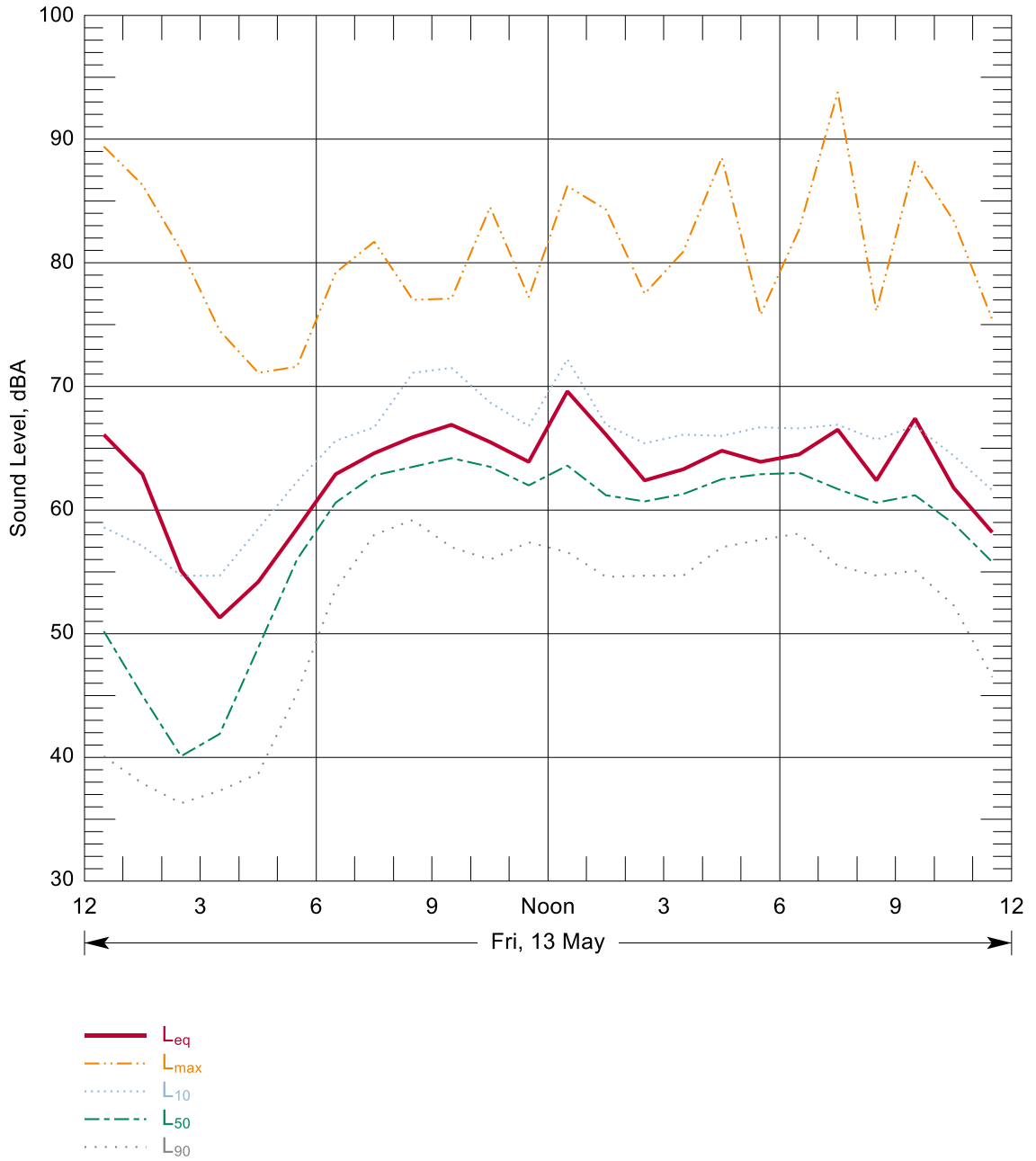
Figure B-55: Hourly Summary of Noise Levels Measured at N91 on 13 May, 2016
