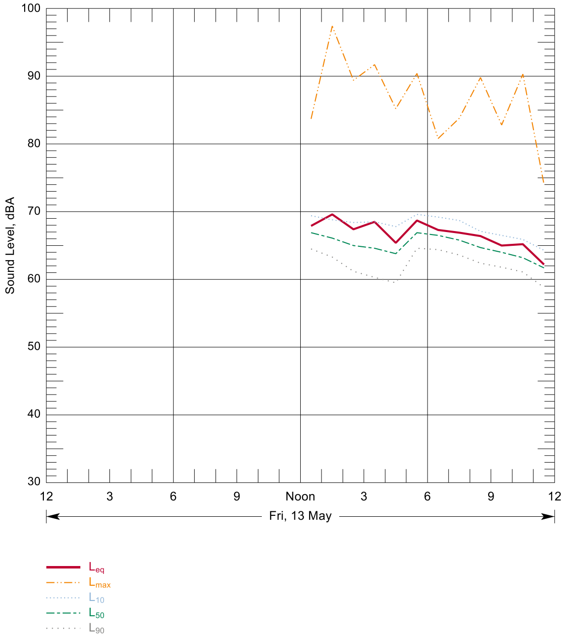
Figure B-99: Hourly Summary of Noise Levels Measured at N105 on 13 May, 2016
