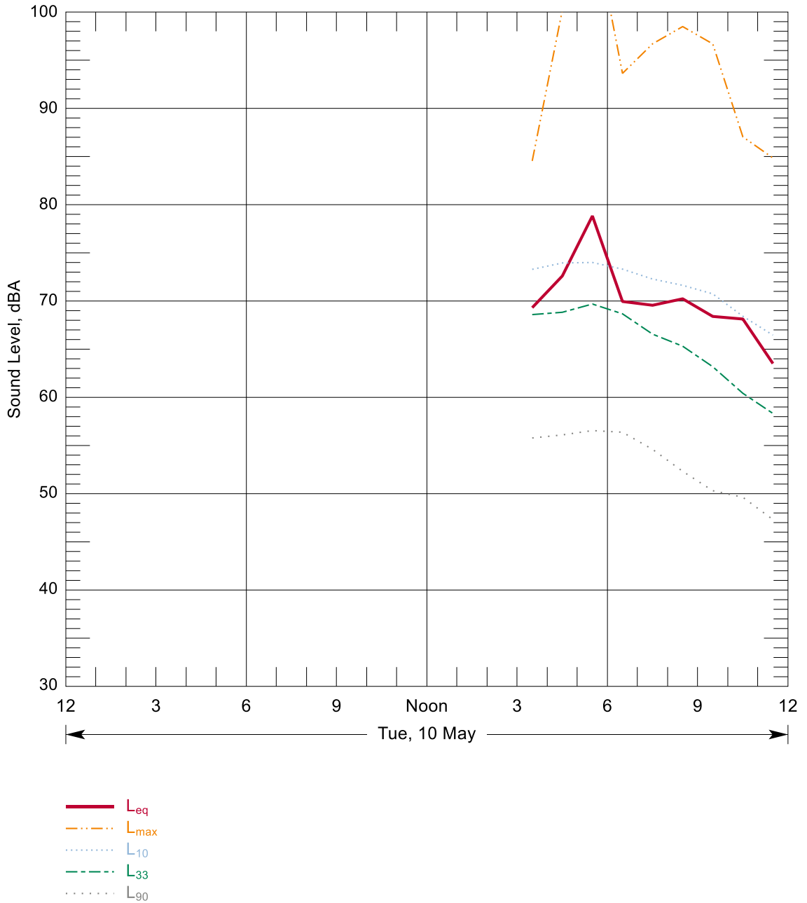
Figure B-61: Hourly Summary of Noise Levels Measured at N93 on 10 May, 2016
