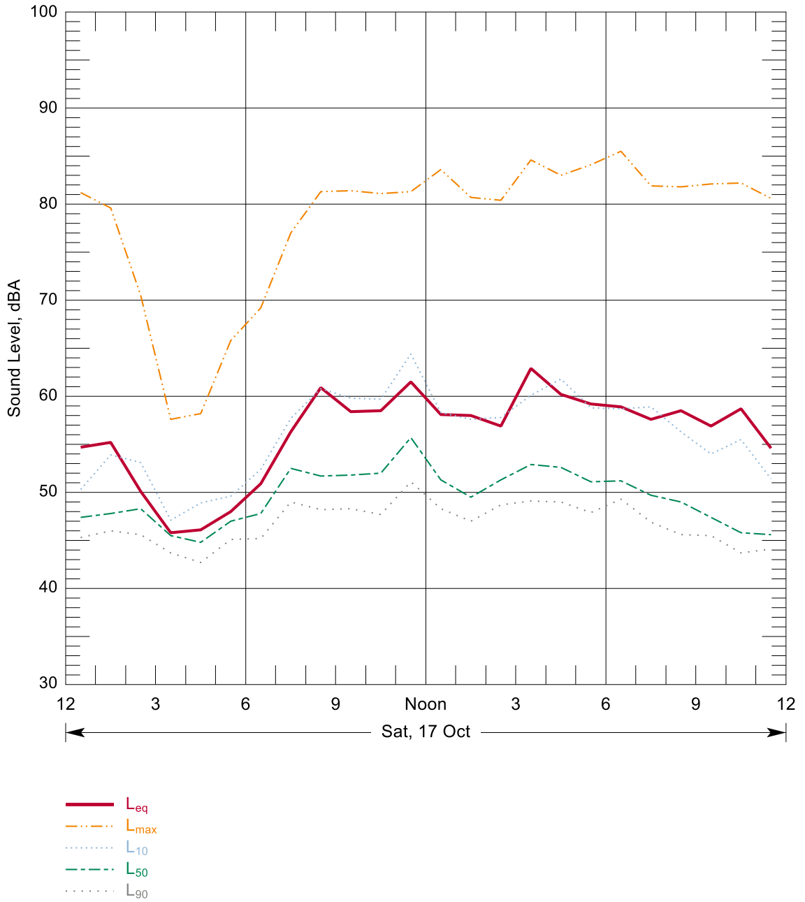
Figure B-7: Hourly Summary of Noise Levels Measured at N77 on 17 Oct, 2009
