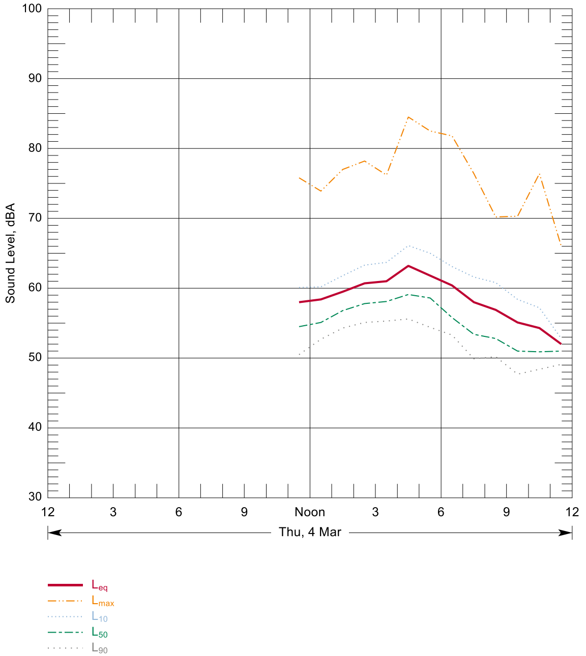
Figure B-11: Hourly Summary of Noise Levels Measured at N78 on 04 Mar, 2010
