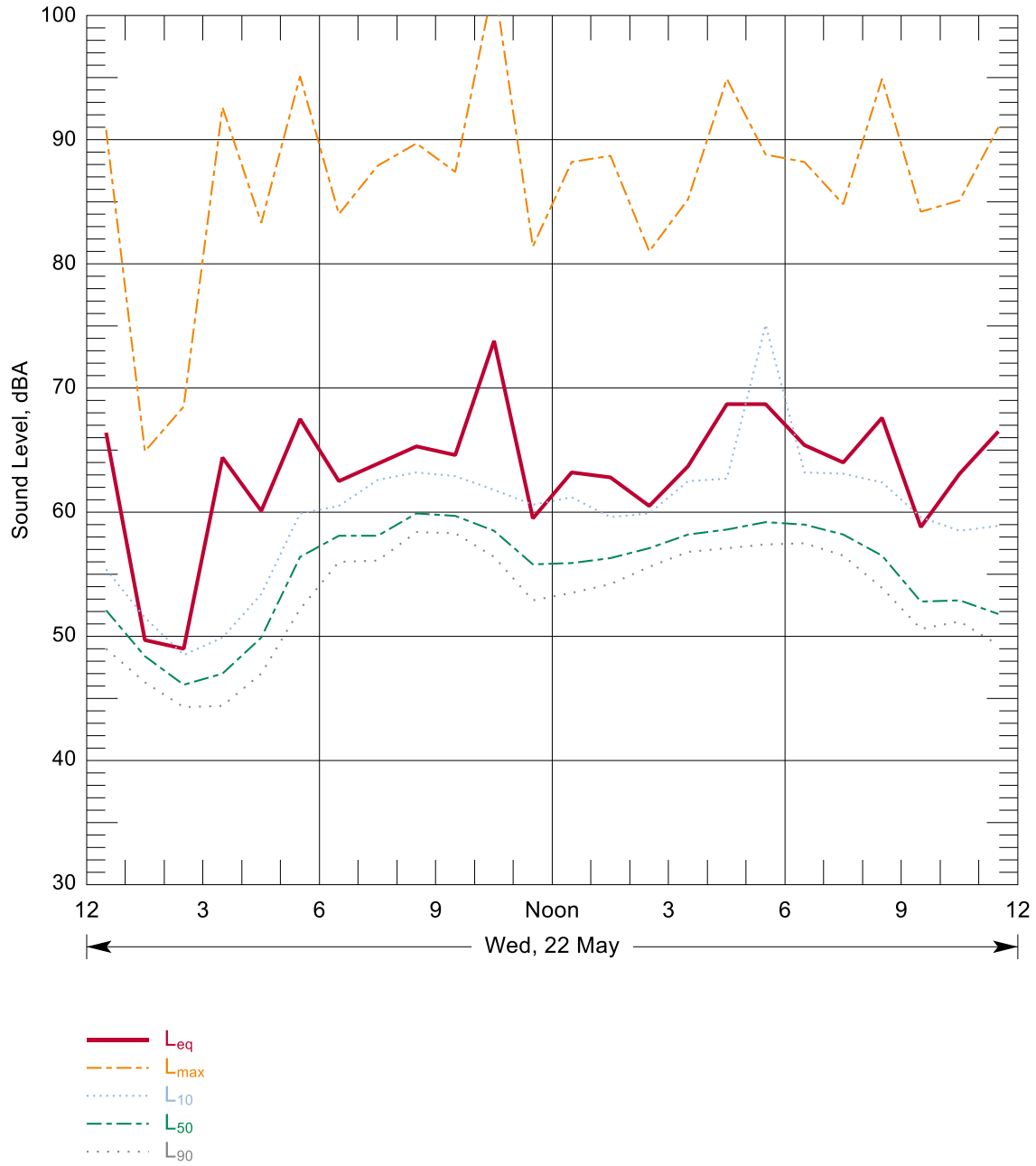
Figure B-222: Hourly Summary of Noise Levels Measured at N140 on 22 May, 2013
