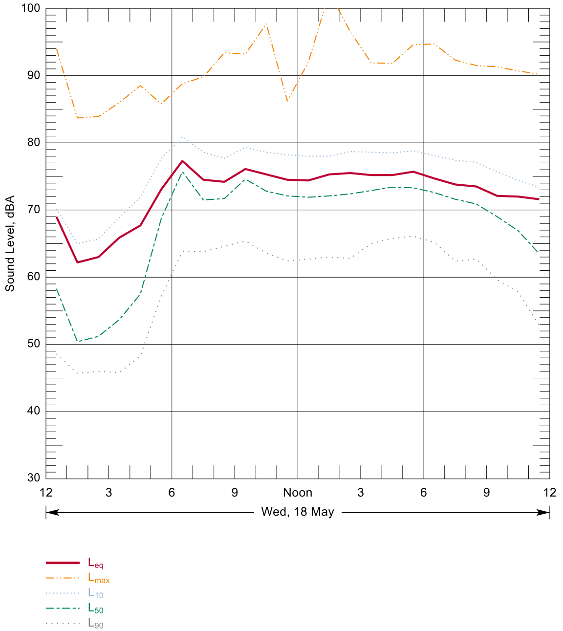
Figure B-43: Hourly Summary of Noise Levels Measured at N87 on 18 May, 2016
