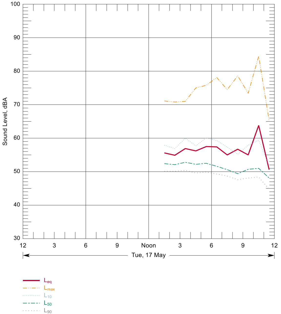
Figure B-39: Hourly Summary of Noise Levels Measured at N86 on 17 May, 2016
