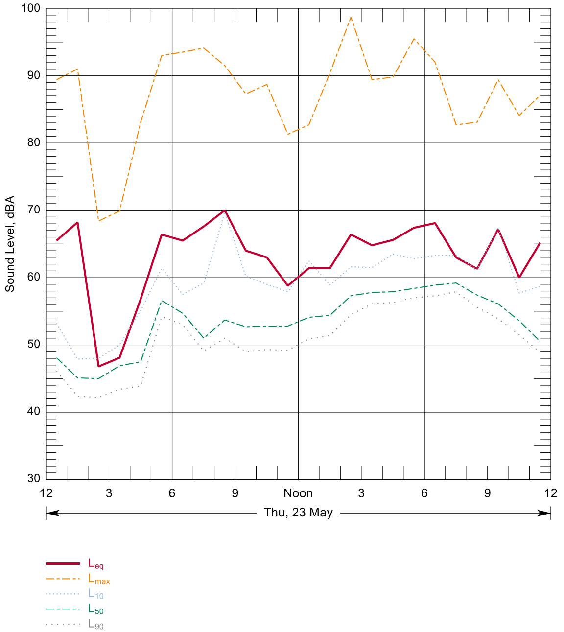
Figure B-223: Hourly Summary of Noise Levels Measured at N140 on 23 May, 2013
