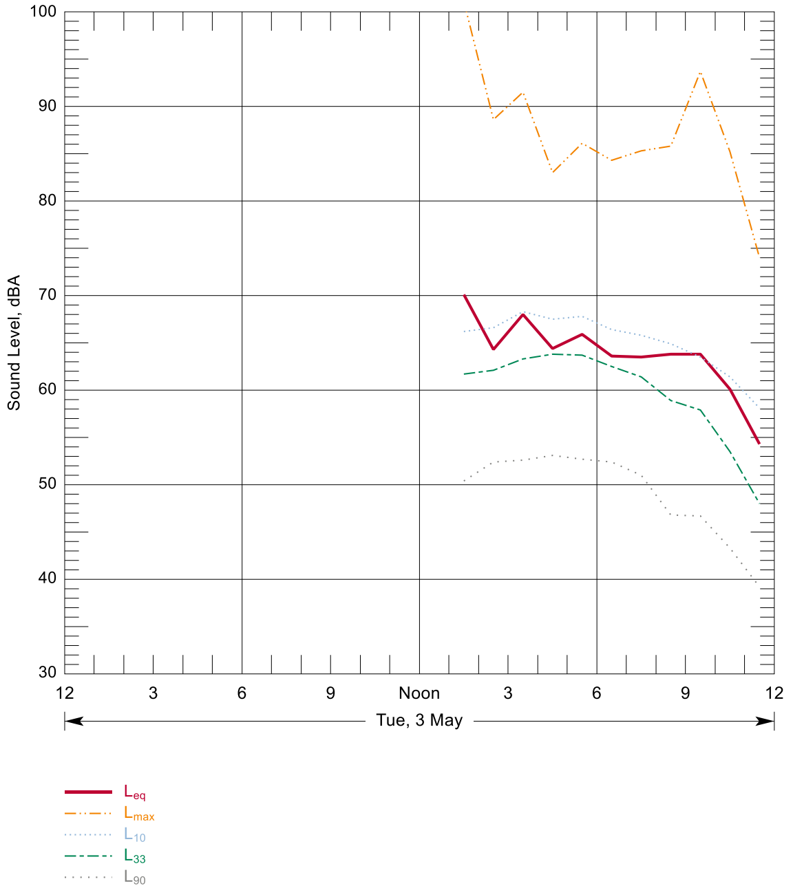
Figure B-95: Hourly Summary of Noise Levels Measured at N104 on 03 May, 2016
