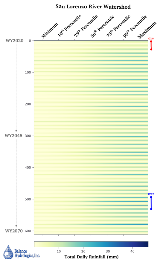
Figure 14: Heat map of population statistics for Projection 2 developed with the stochastic sampling (Figure 13). The y-axis plots how the statistics shown on the x-axis vary from month to month over the CC analysis period. Darker blue colors indicate relatively wet periods, and stronger yellow colors indicate dry periods. An example wet and dry period are indicated.
