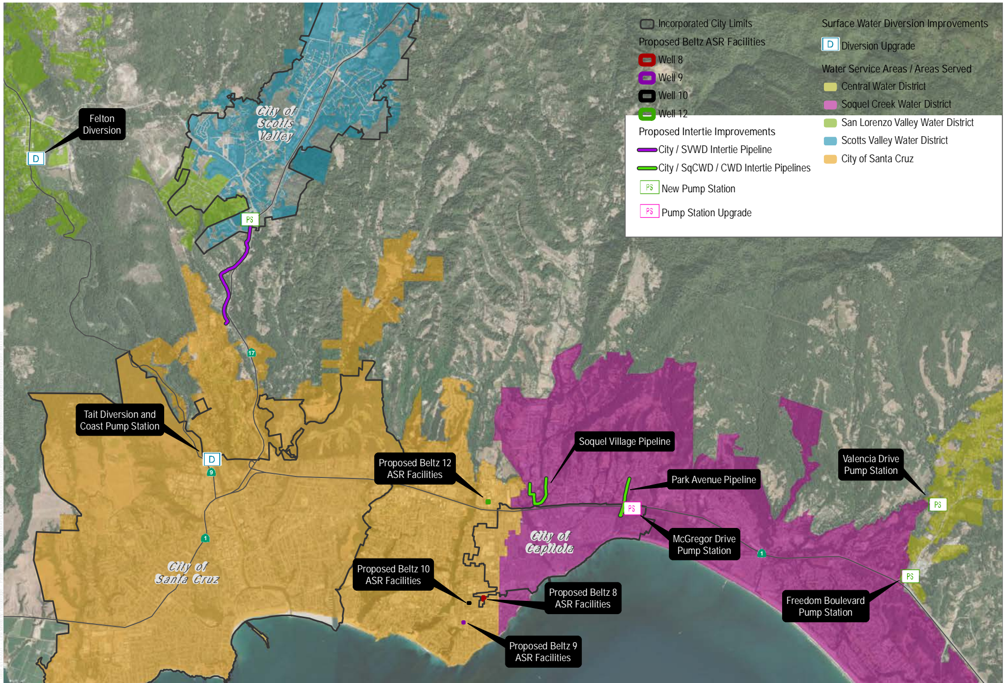
FIGURE 4 Proposed New and Upgraded Infrastructure Components Santa Cruz Water Rights Project
