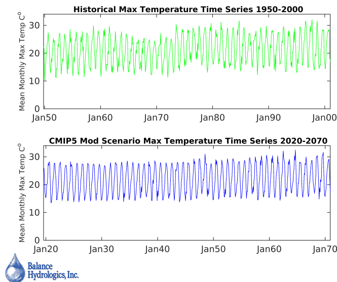
Figure 16: Comparison of an historical period observed maximum air temperature for Santa Cruz vs. the Projection 2 maximum air temperature developed using the stochastic modeling approach.
