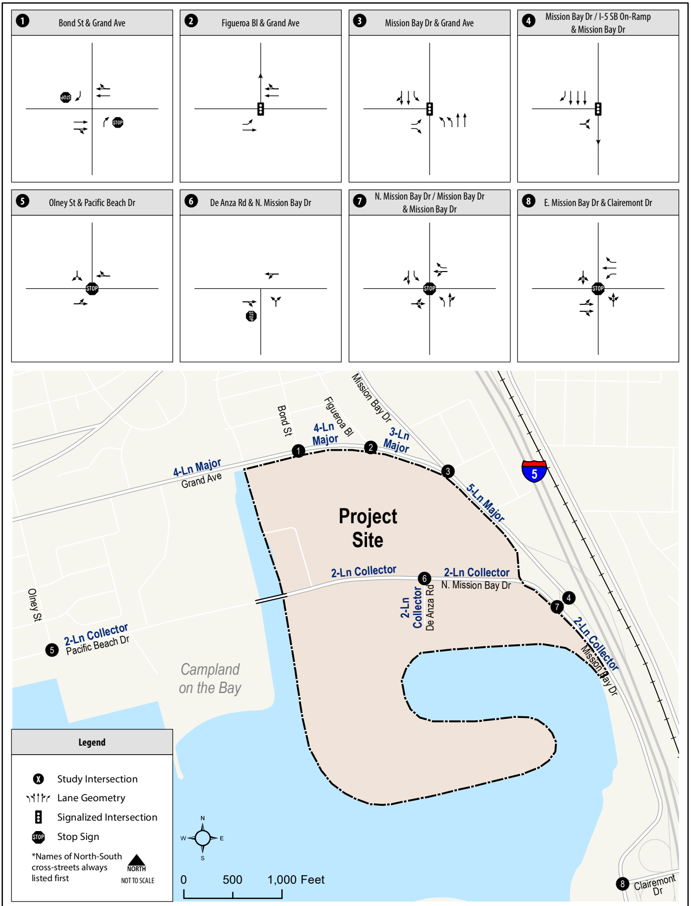
Figure 4-11 Existing Roadway and Intersection Geometrics
