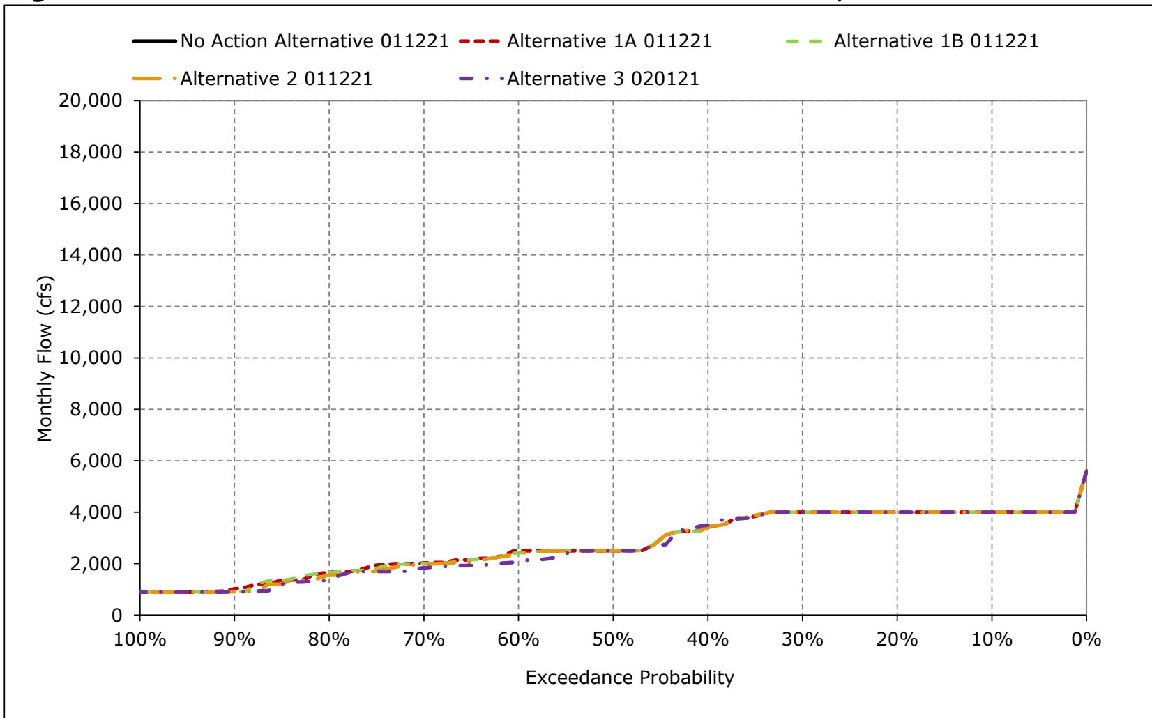
Figure 5B2-22-7. Feather River Flow downstream of Thermalito, October
