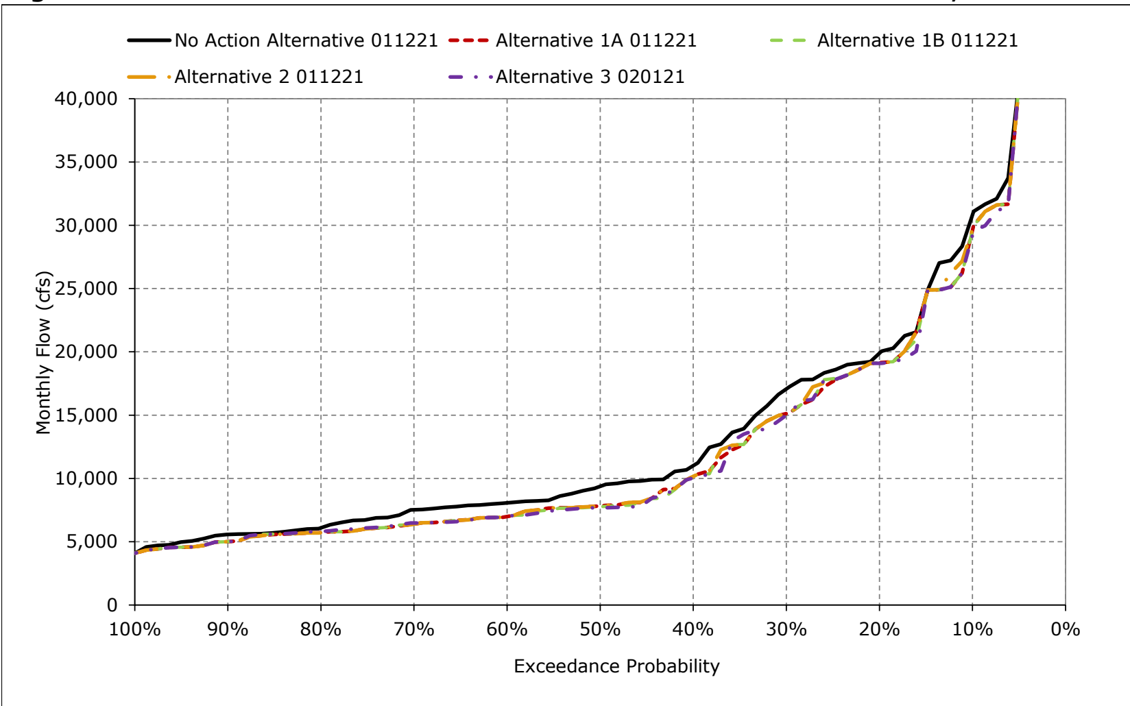
Figure 5B2-12-12. Sacramento River below Red Bluff Diversion Dam Flow, March
