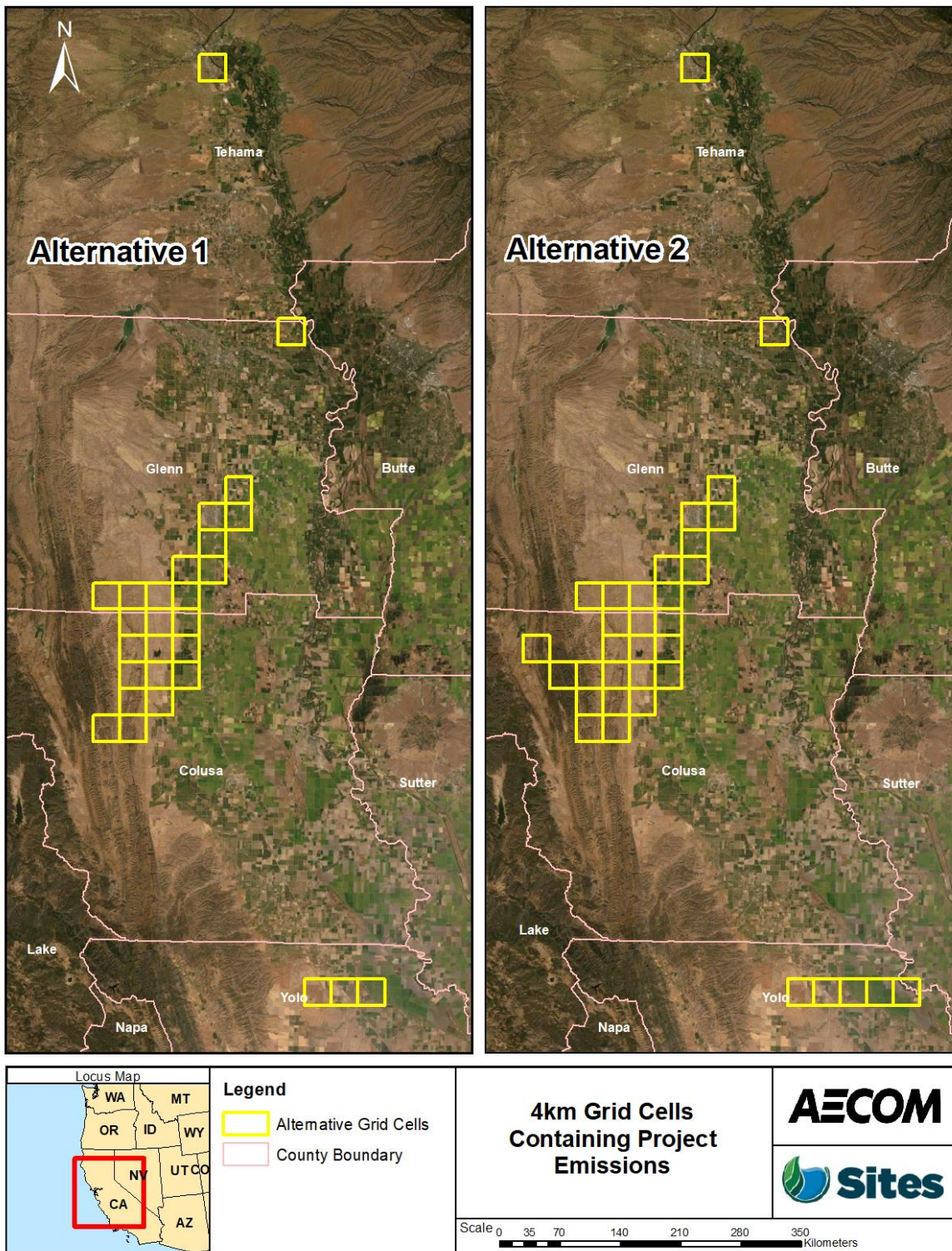
Figure 20D-2. Project Grid Cells for Each Alternative
