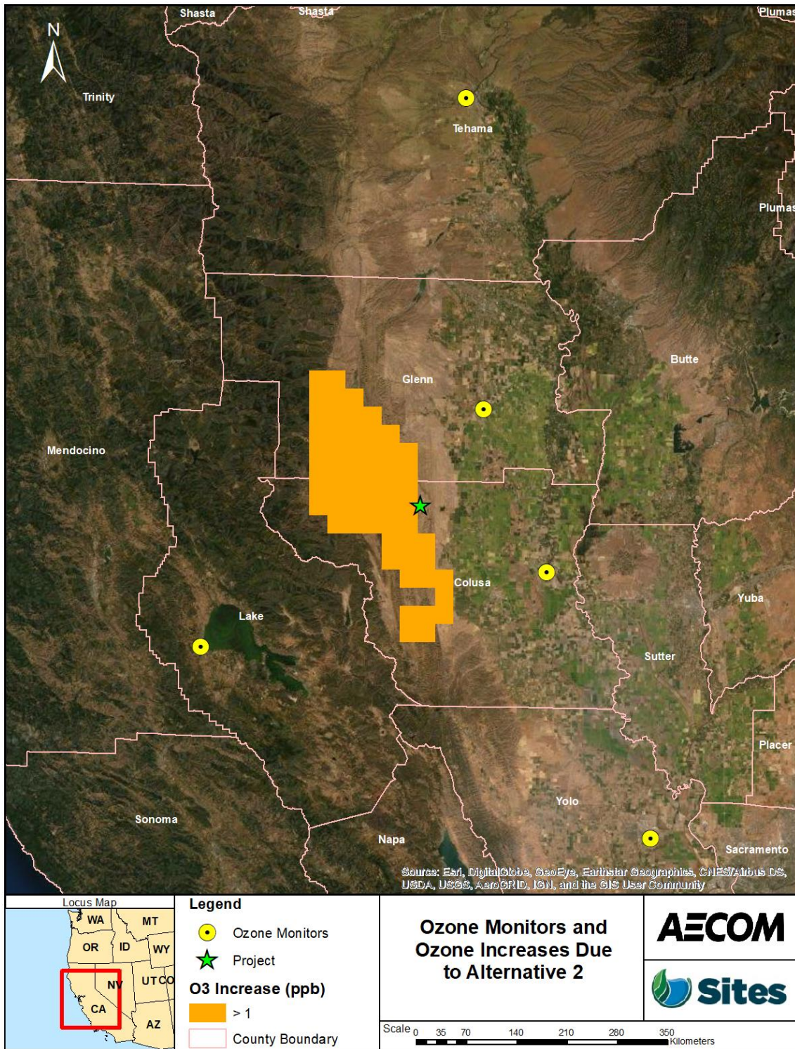
Figure 20D-4. Ozone Monitors and Ozone Increases Due to Alternative 2
