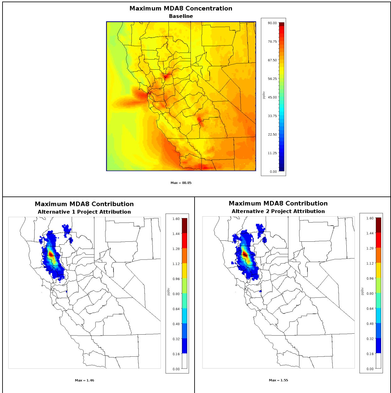
Figure 20D-3. Maximum Baseline MDA8 Concentrations and Maximum Project Contributions for each Alternative
