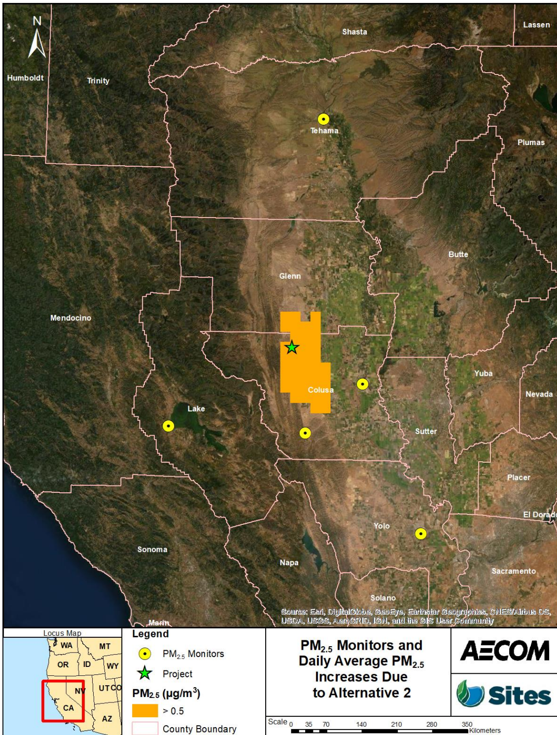
Figure 20D-7. PM 2.5 Monitors and Daily Average PM 2.5 Increases Due to Alternative 2
