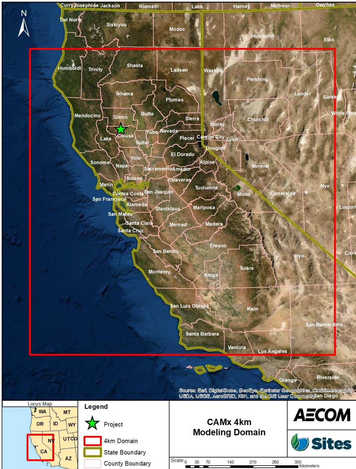
Figure 20D-1. CAMx Modeling Domain
