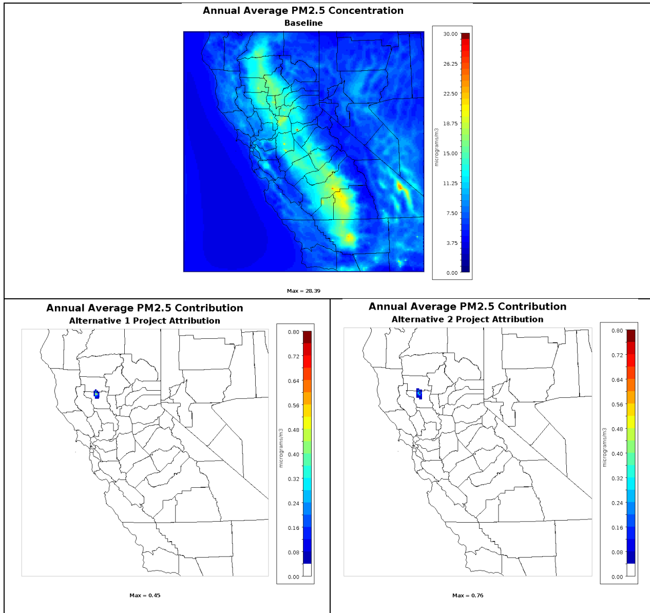
Figure 20D-6. Annual Average Baseline PM 2.5 Concentrations and Maximum Project Contributions for each Alternative
