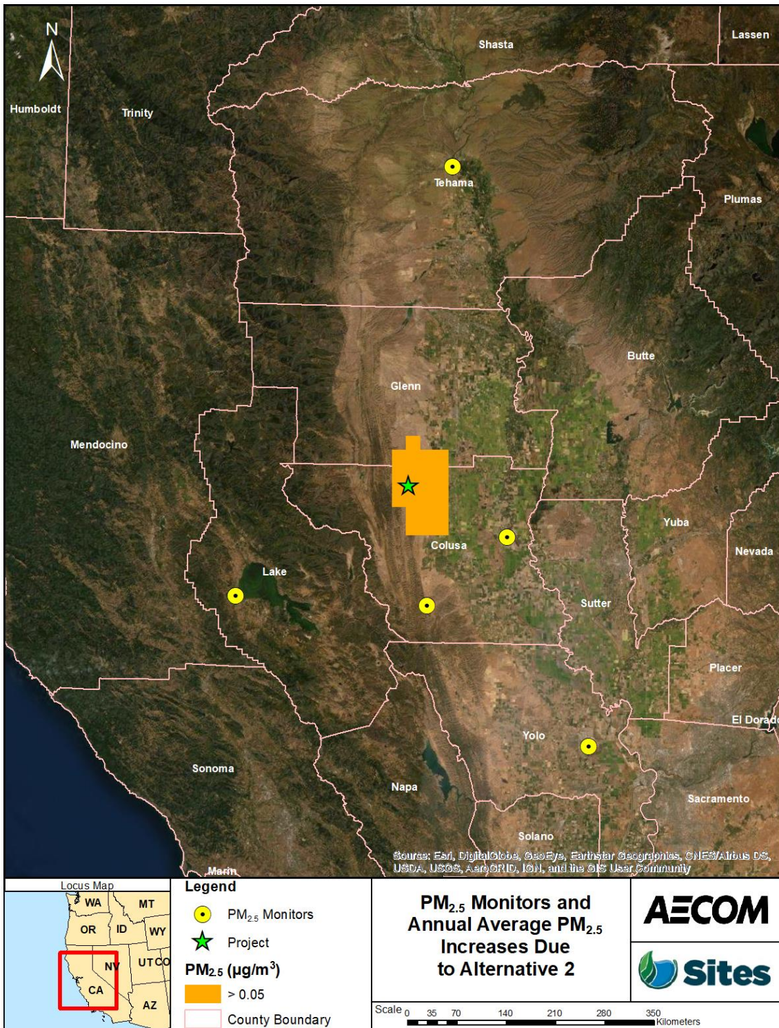
Figure 20D-8. PM 2.5 Monitors and Annual Average PM 2.5 Increases Due to Alternative 2
