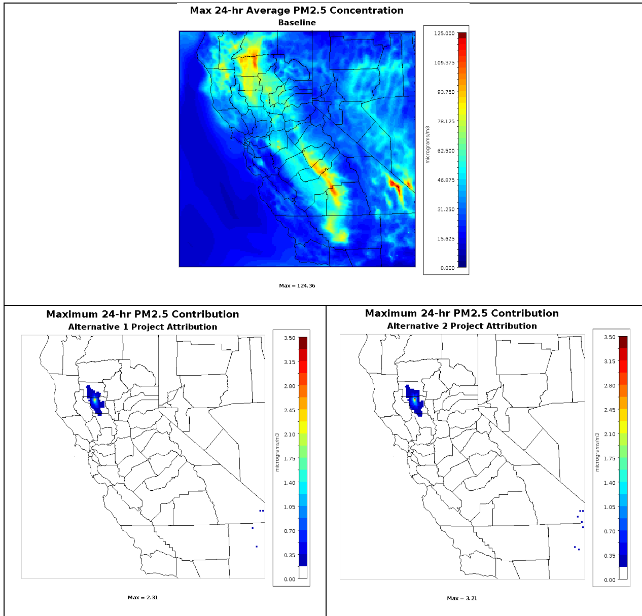
Figure 20D-5. Maximum Daily Average Baseline PM 2.5 Concentrations and Maximum Project Contributions for each Alternative
