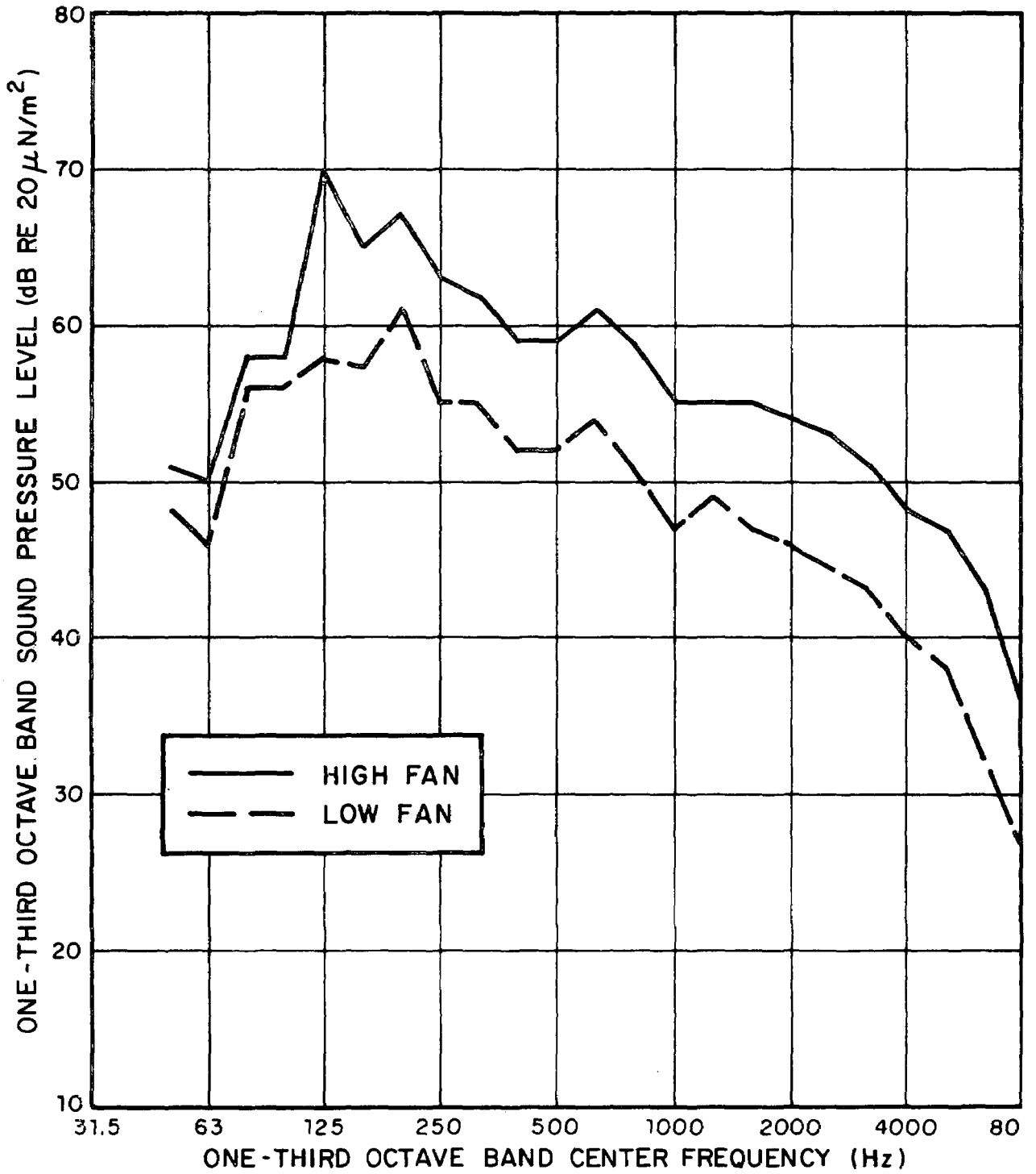
FIG. 7. SOUND PRESSURE LEVELS FROM AIR CONDITIONER ON TWO SETTINGS (MEASURED AT 3 ft)
