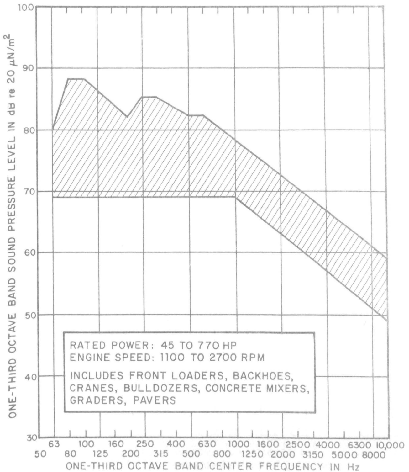
FIG. A.1 ENVELOPE OF SOUND PRESSURE LEVELS FROM 29 DIESEL-POWERED ITEMS OR CONSTRUCTION EQUIPMENT (MEASURED AT 50 FT)
