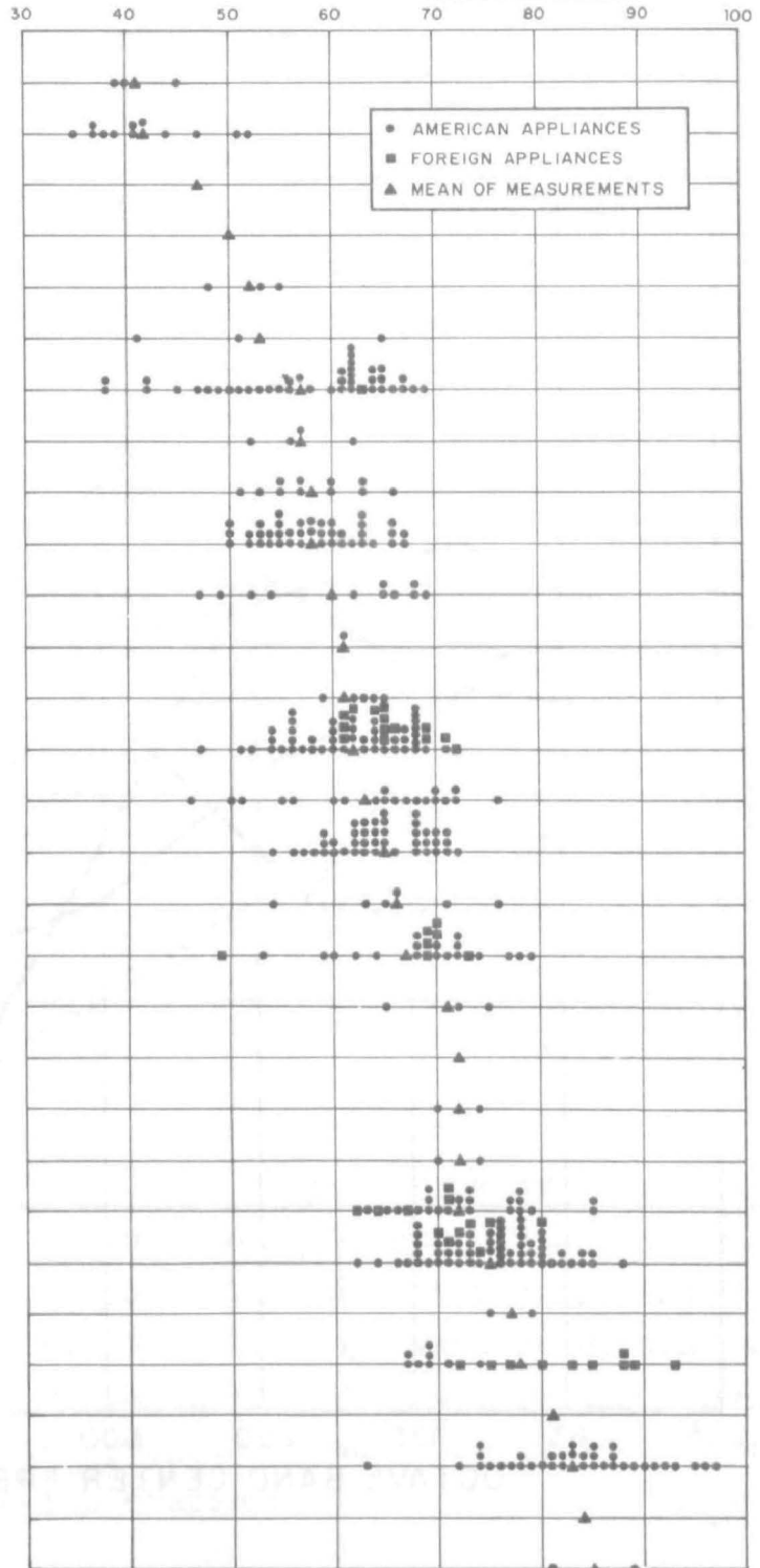
FIG. 3. A SUMMARY OF NOISE LEVELS FOR APPLIANCES MEASURED AT A DISTANCE OF 3 FT.
