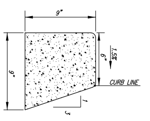
0" CURB DETAIL (PVT) NOT TO SCALE SEE SPSSD G-1 FOR ADDITIONAL INFORMATION AND G-10 FOR JOINT DETAILS
