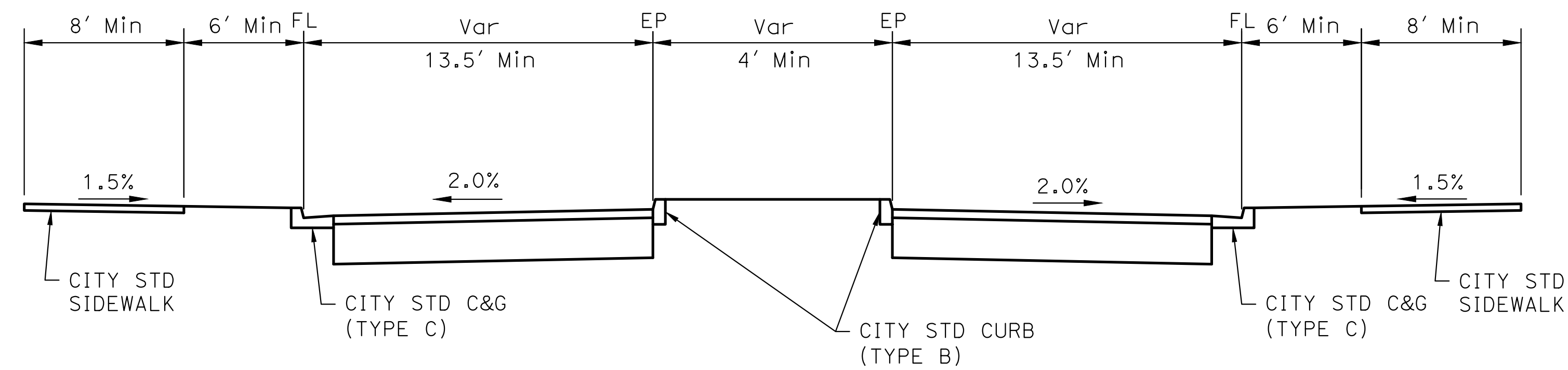
MCKINNON STREET AT ROUNDABOUT APPROACHES
