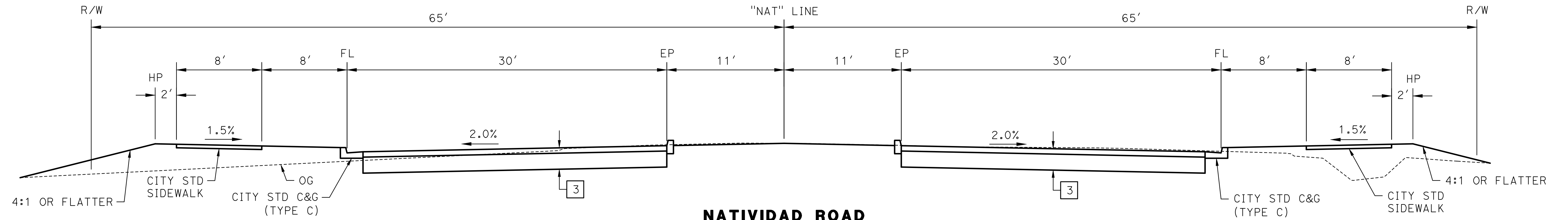
NATIVIDAD ROAD AT NORTHERN CONFORM (BY OTHERS)
