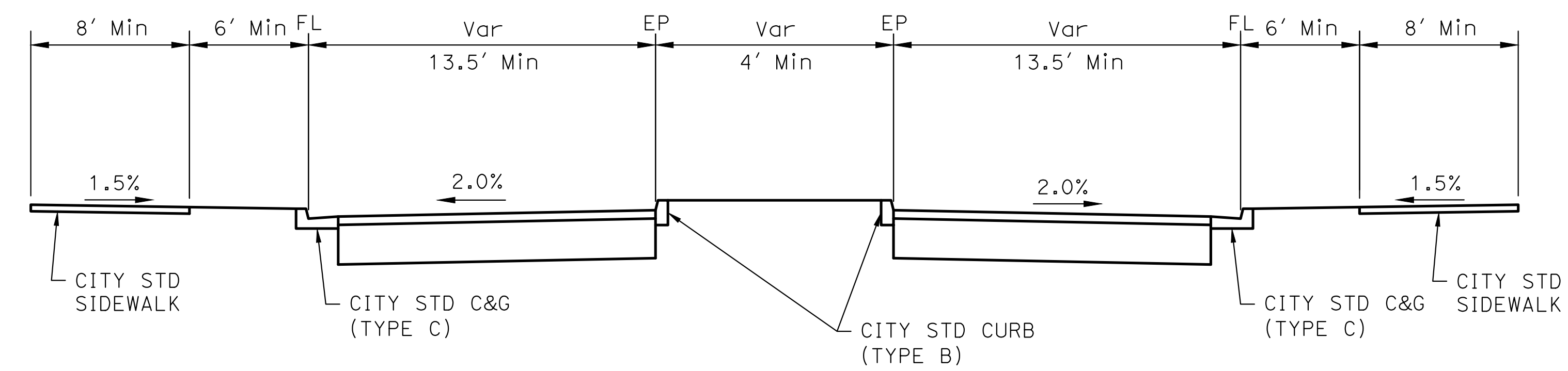
INDEPENDENCE BOULEVARD AT ROUNDABOUT APPROACHES
