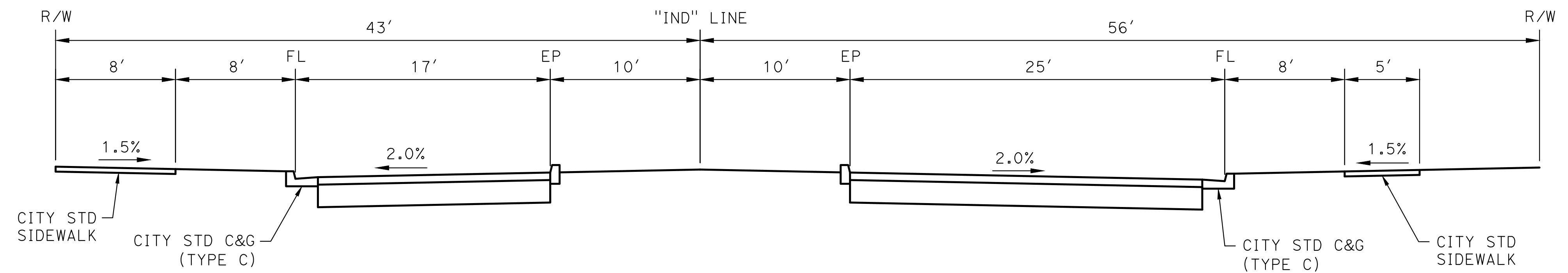
INDEPENDENCE BOULEVARD AT NORTHERN CONFORM (BY OTHERS)
