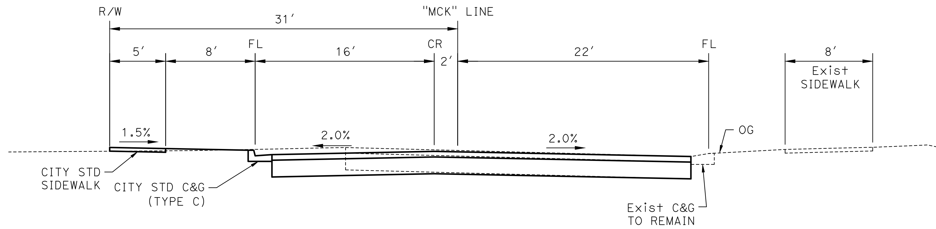
MCKINNON STREET AT NORTHERN CONFORM (BY OTHERS)
