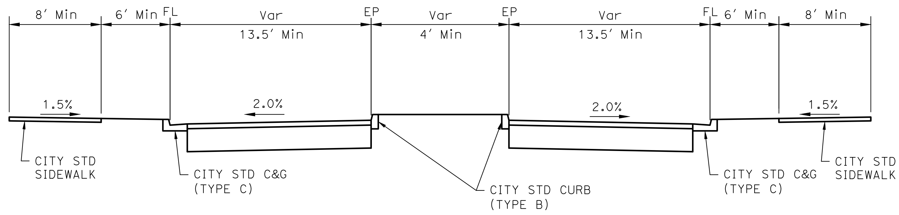
EL DORADO DRIVE AT ROUNDABOUT APPROACHES
