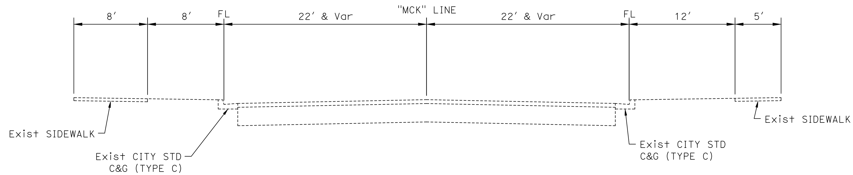
MCKINNON STREET AT SOUTHERN CONFORM (EXISTING)
