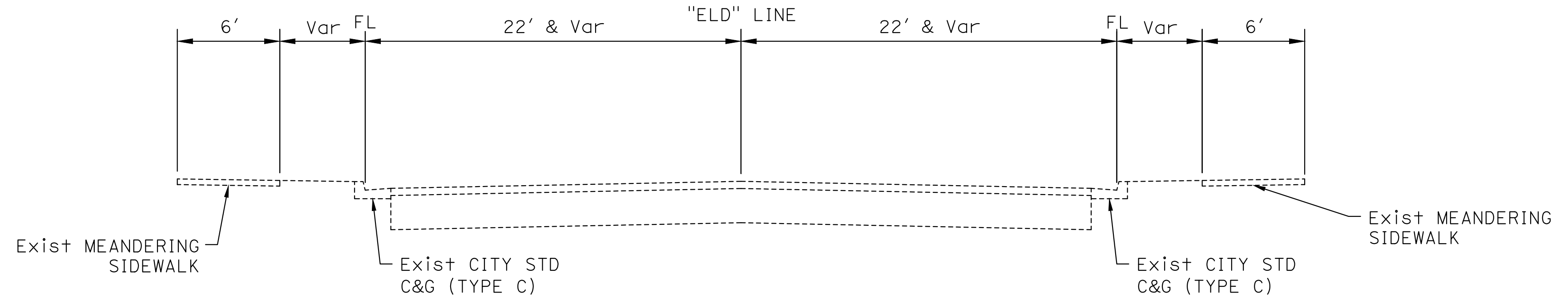
EL DORADO DRIVE AT SOUTHERN CONFORM (EXISTING)
