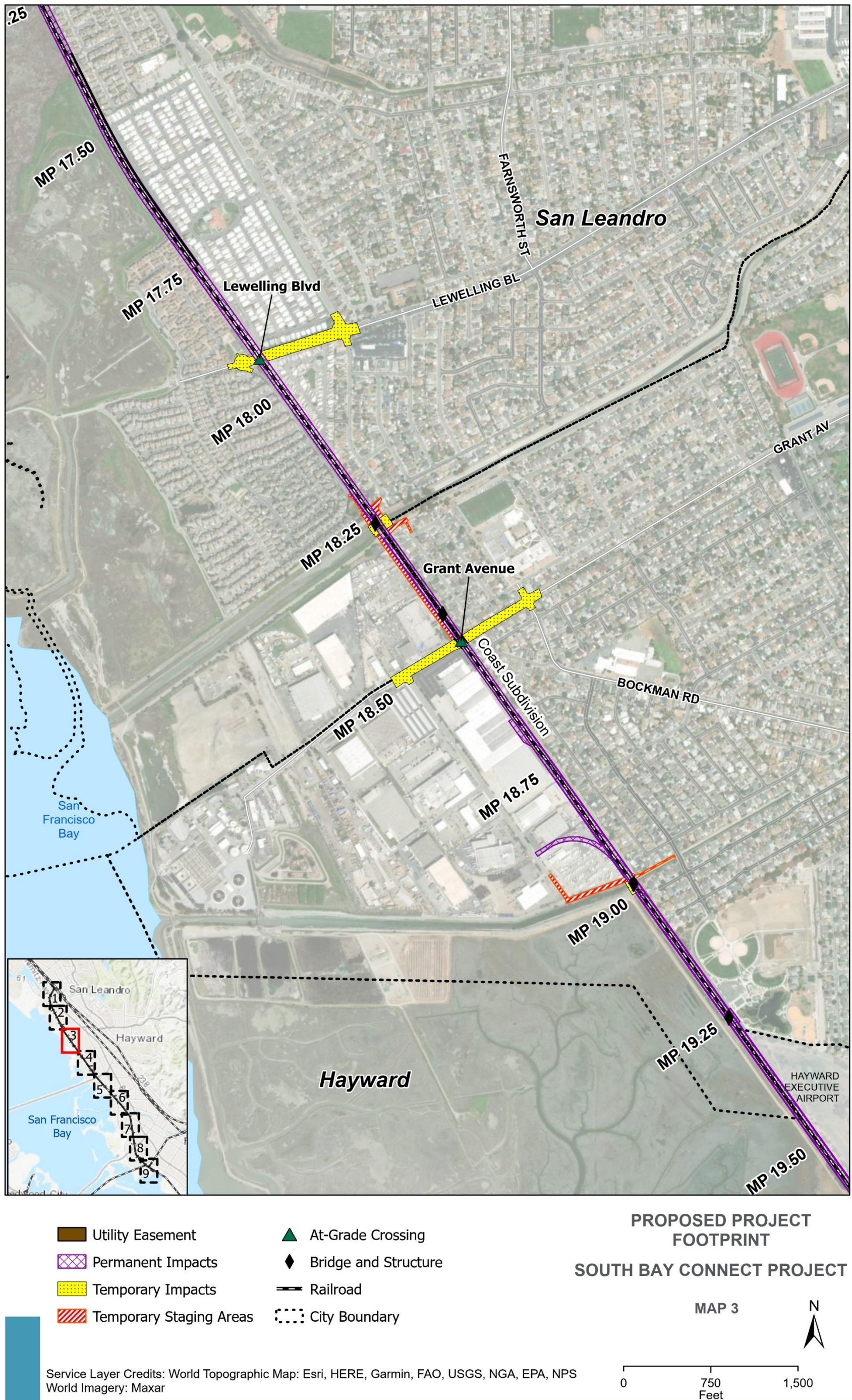
Figure 2-4. Proposed Project Footprint – Segment C
