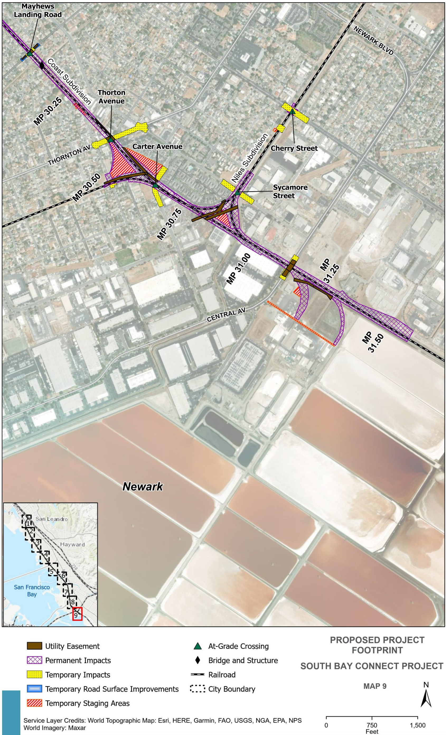
Figure 2-10. Proposed Project Footprint—Segment I
