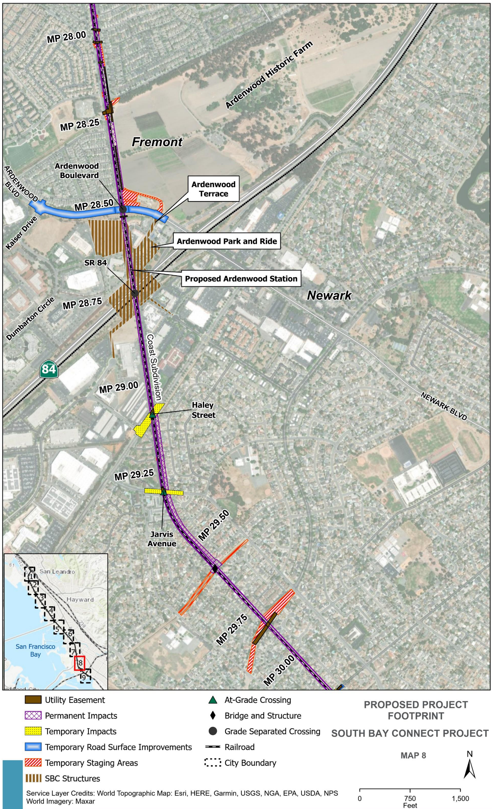
Figure 2-9. Proposed Project Footprint – Segment H
