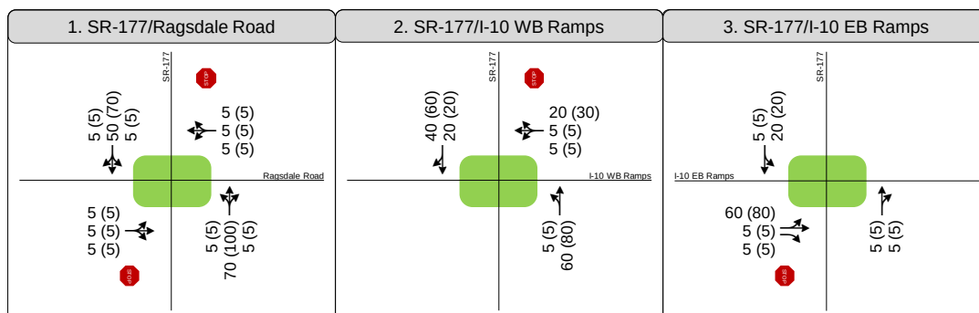
Figure 5 Peak Hour Traffic Volumes and Lane Configurations - Existing Conditions
