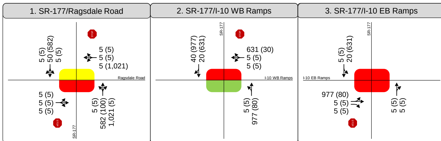
Figure 9 Peak Hour Traffic Volumes and Lane Configurations - Ambient Plus Project Conditions
