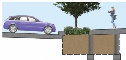
SUSPENDED SIDEWALK Thickened sidewalk with reinforcement and/or footings can be used allowing tree roots to grow below the sidewalk.
