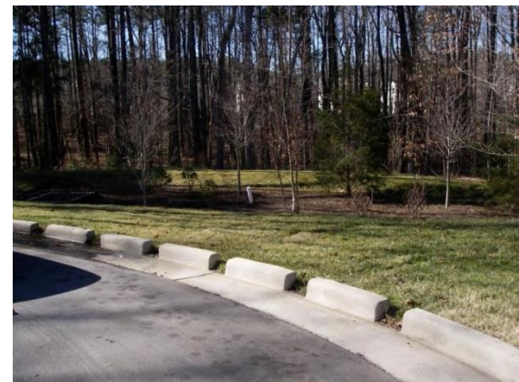
Curb cuts with filter strip/dispersion area
