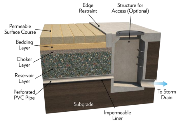
Reservoir layer with underdrain and impermeable liner
