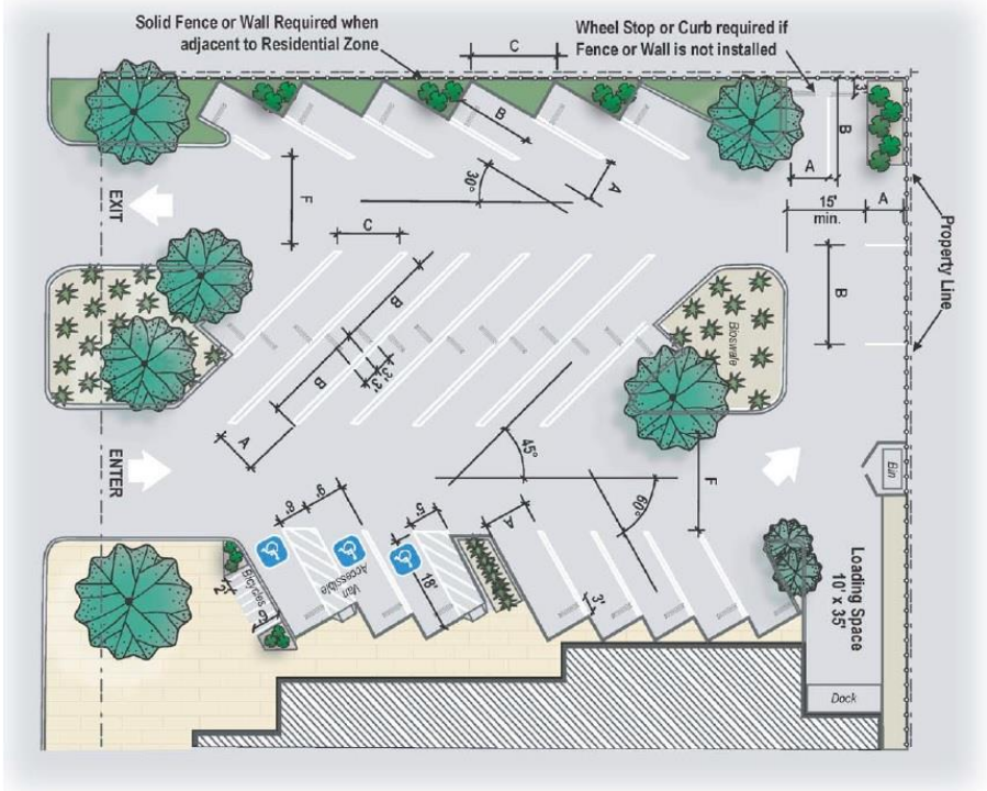
CONCEPTUAL PARKING LOT DIAGRAM (Source: County of San Diego, Parking Design Manual)
