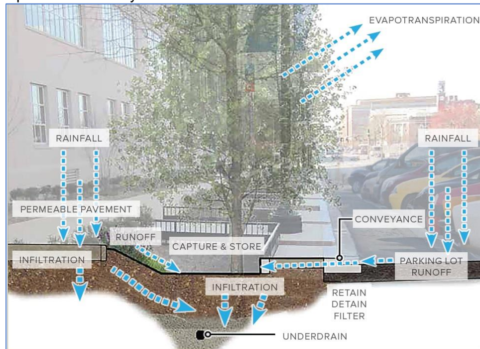
Stormwater Diagram
