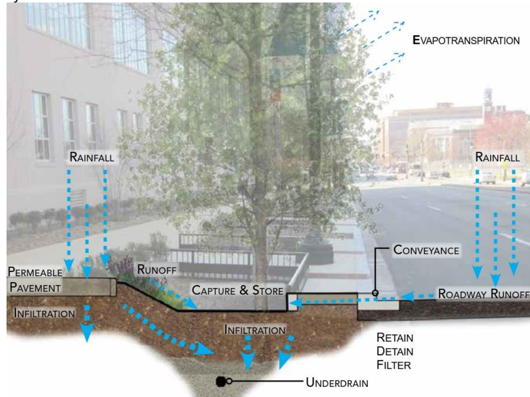
Green Streets Stormwater Diagram
