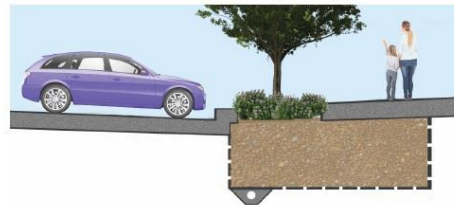
STRUCTURAL SOILS A specific mix of stone and soil that supports the sidewalk while allowing tree roots to grow normally.
