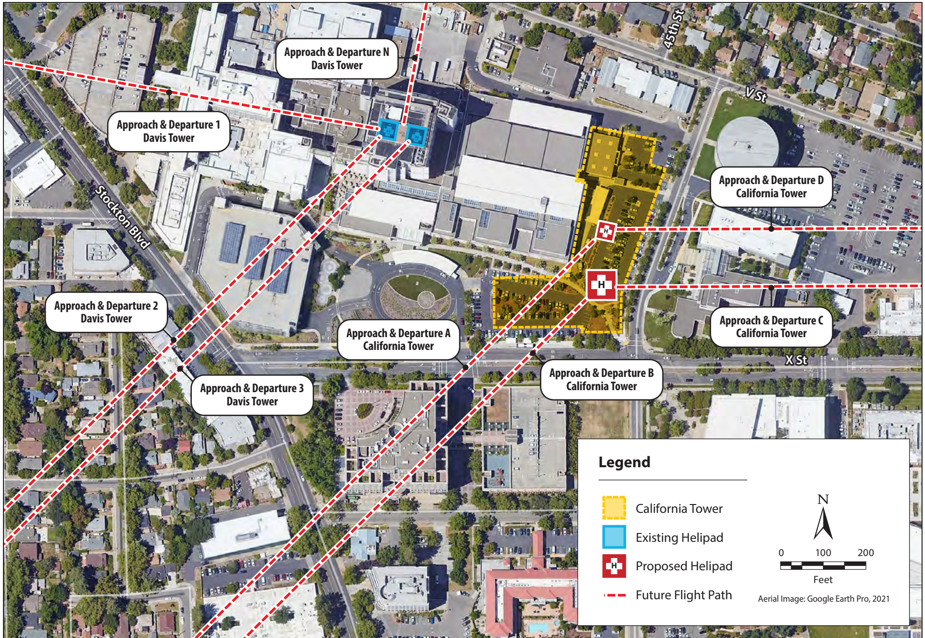
Figure 13 Future Helicopter Flight Paths Davis Tower and CA Tower
