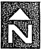
Base Map: Alquist-Priolo Earthquake Fault Zones, 7.5 minute, Alberhill Quadrangle, topographic base USGS 1954, photorevised 1973.
