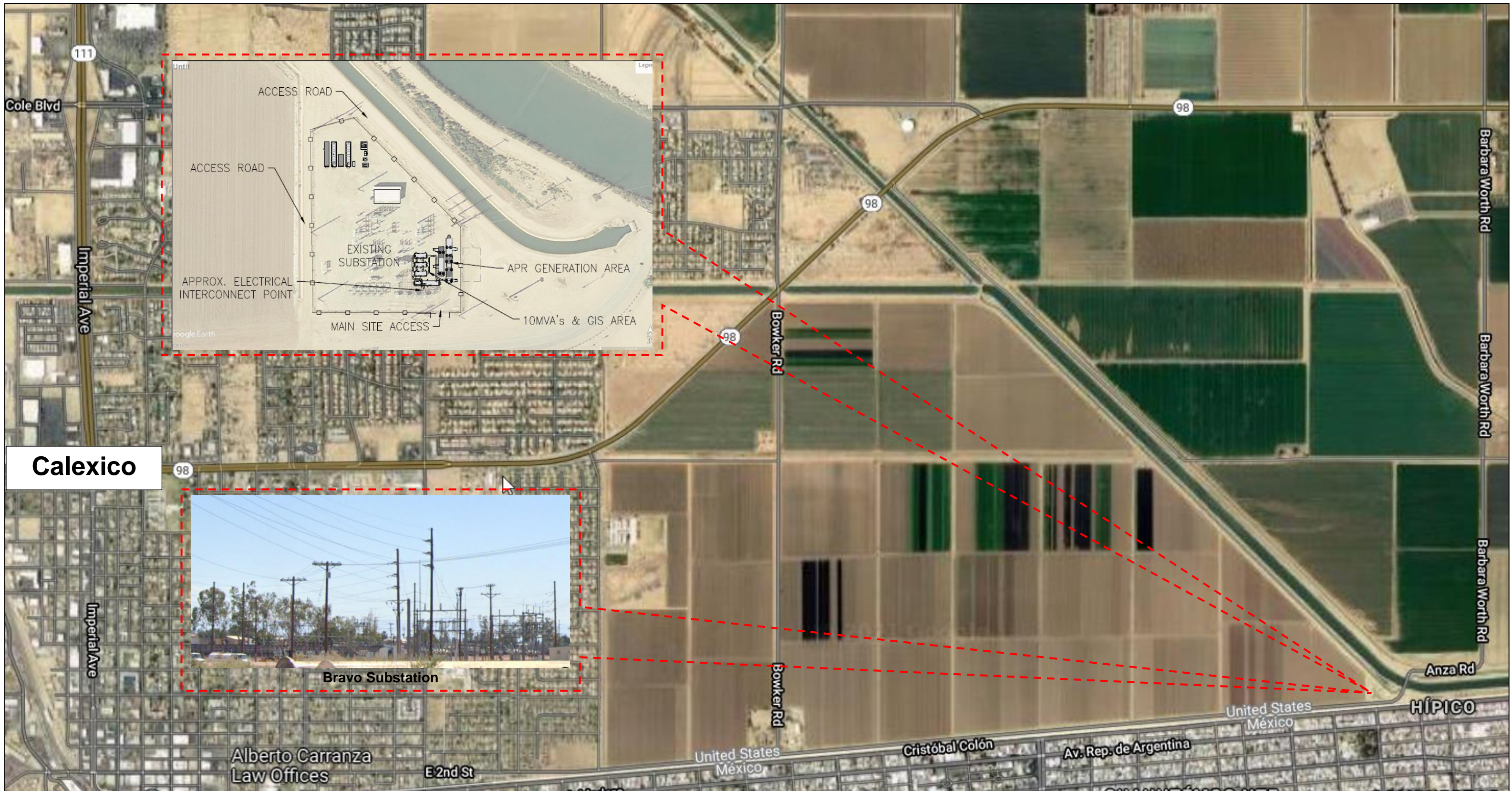
Bravo Substation Location Map & Site Plan
