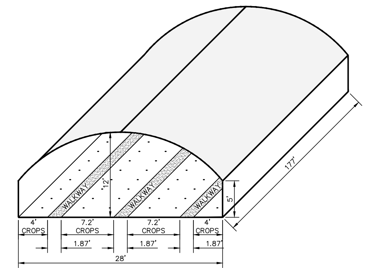
HOOP HOUSE CROP DESIGN DETAIL NTS
