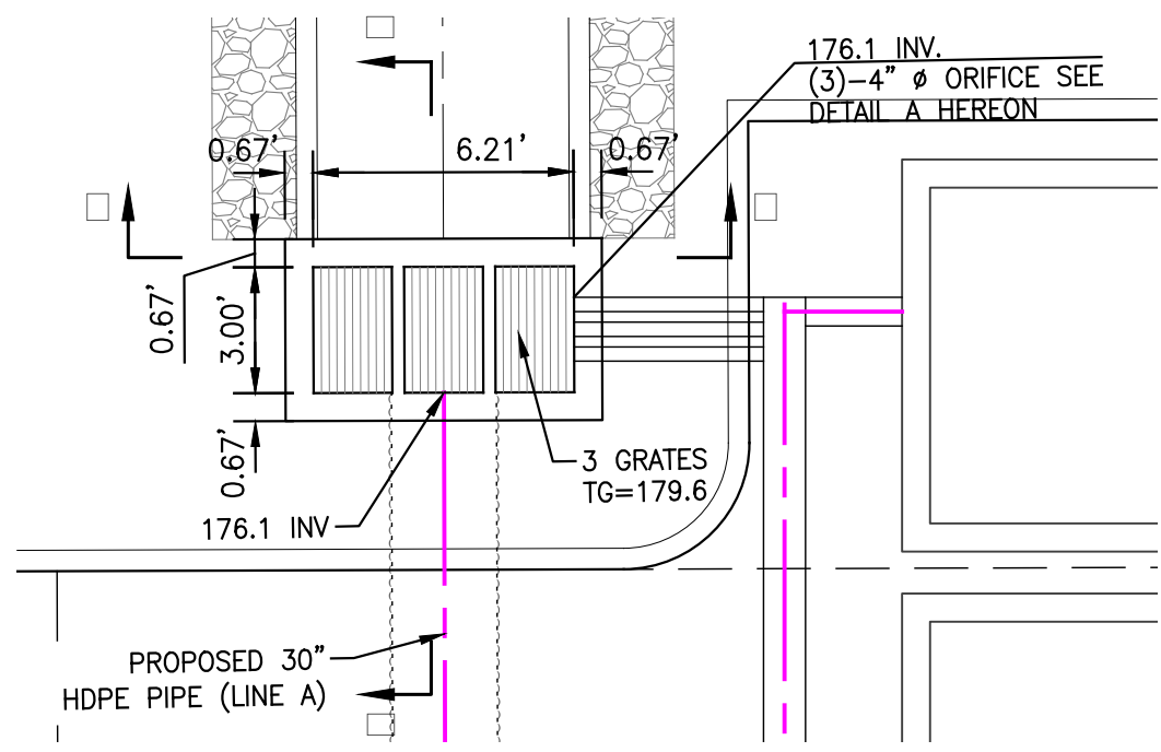
GRATING CATCH BASIN DETAIL STRUCTURE DETAIL PER SPPWC STD. DWG. 305-4, MODIFIED AS SHOWN
