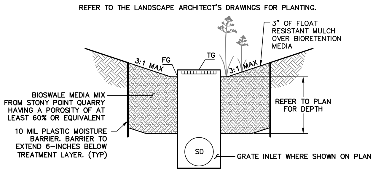
① VOLUME CAPTURE FACILITY NO SCALE
