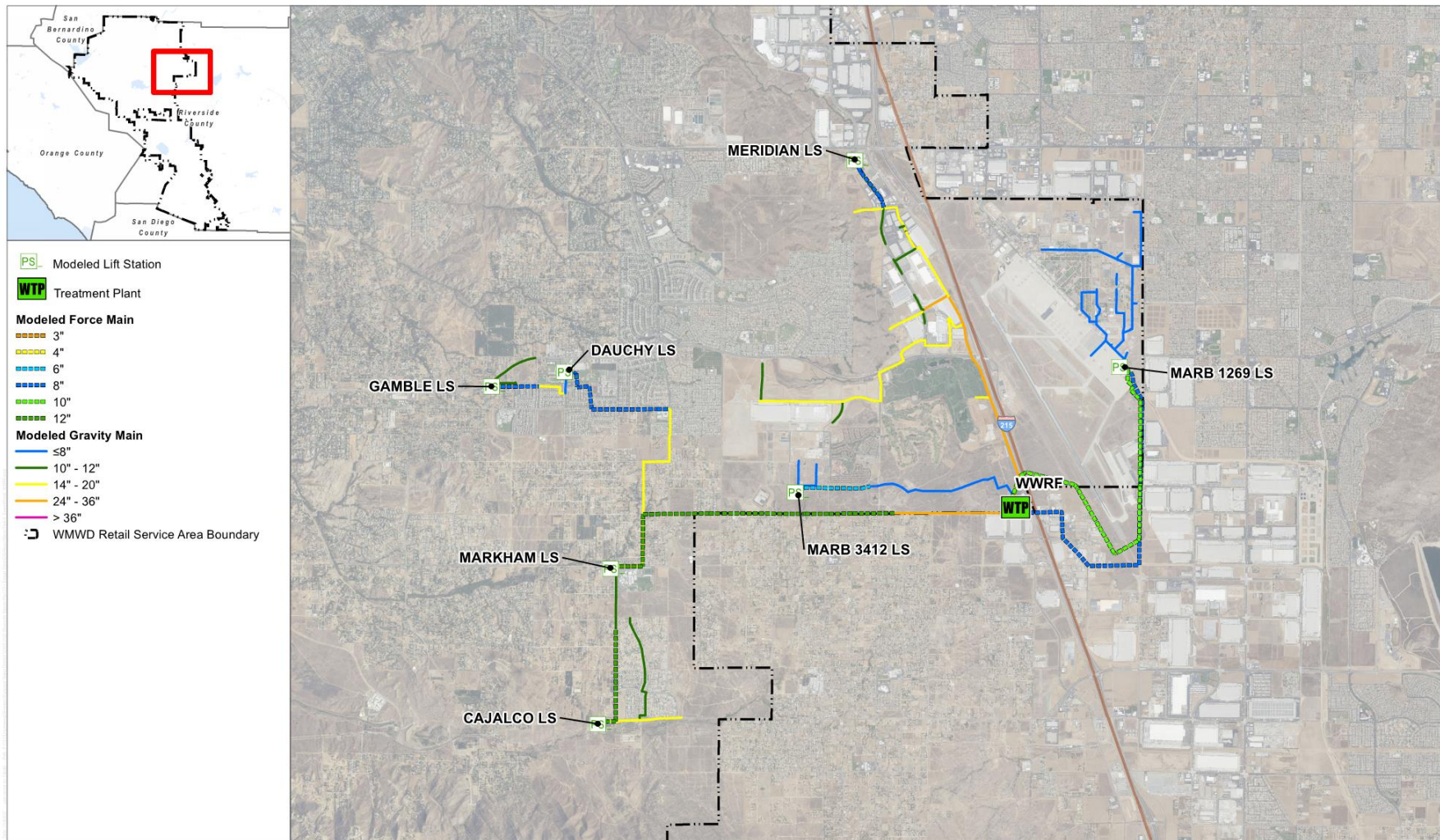
Figure 4-3: Sewer Model WWRP
