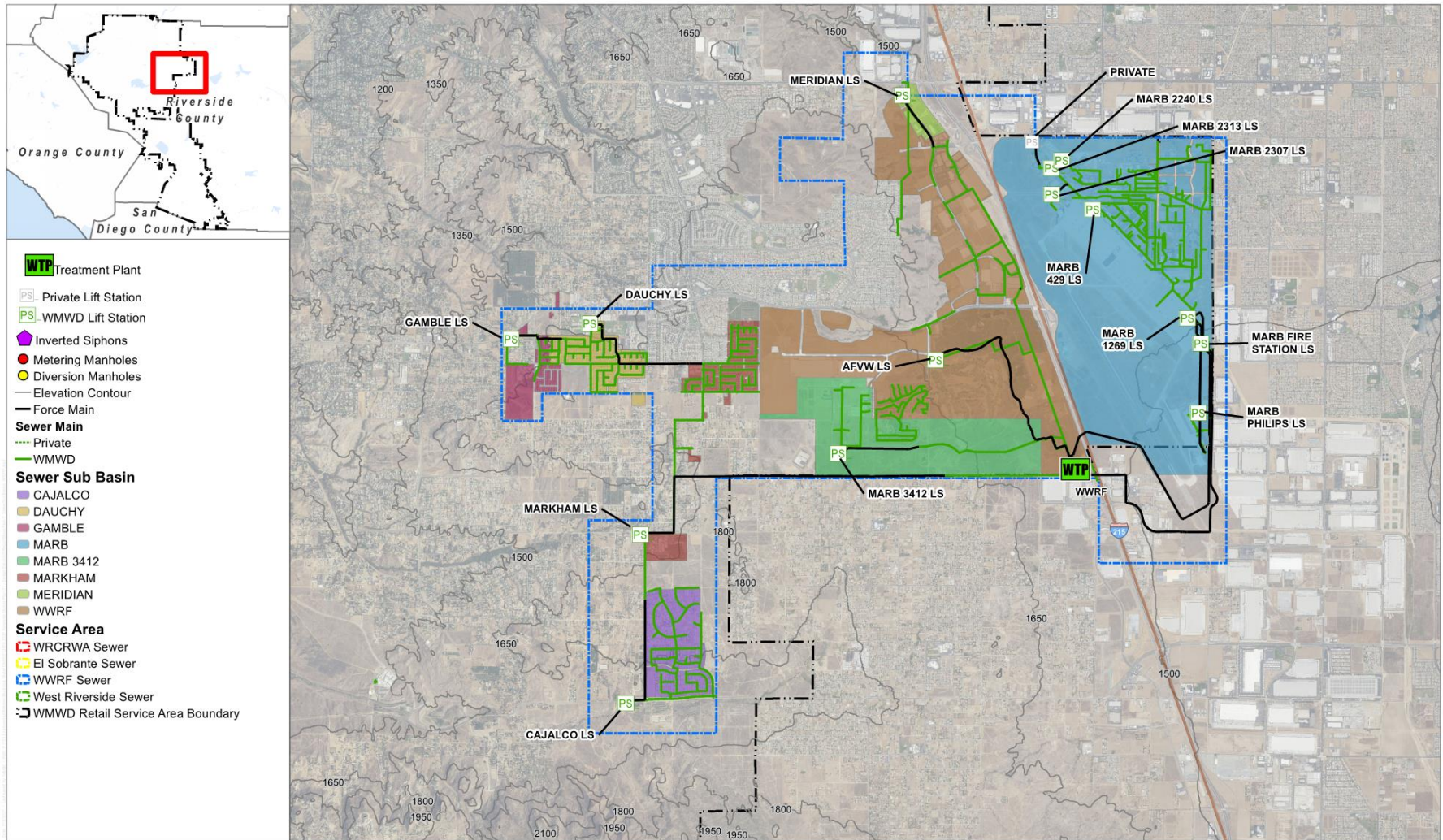
Figure 4-5: Sewer Sub Basins – WWRF Service Area
