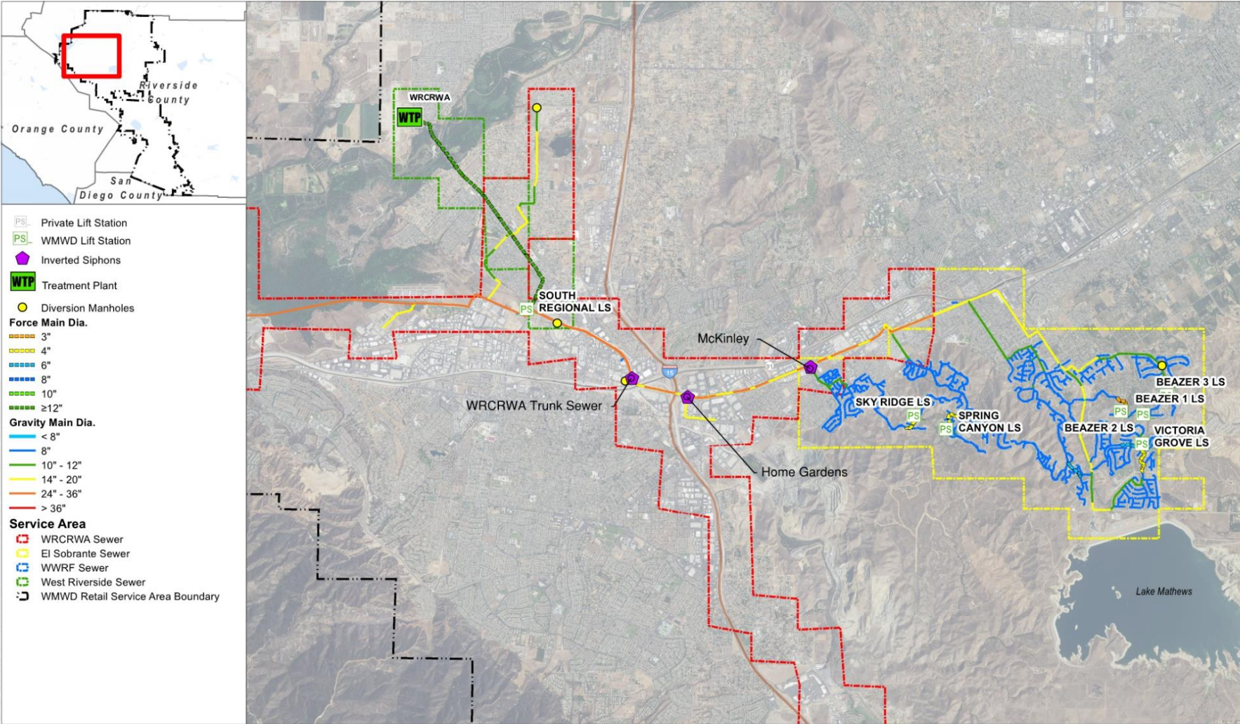
Figure 2-10: Western Wastewater Study Area - WRCRWA
