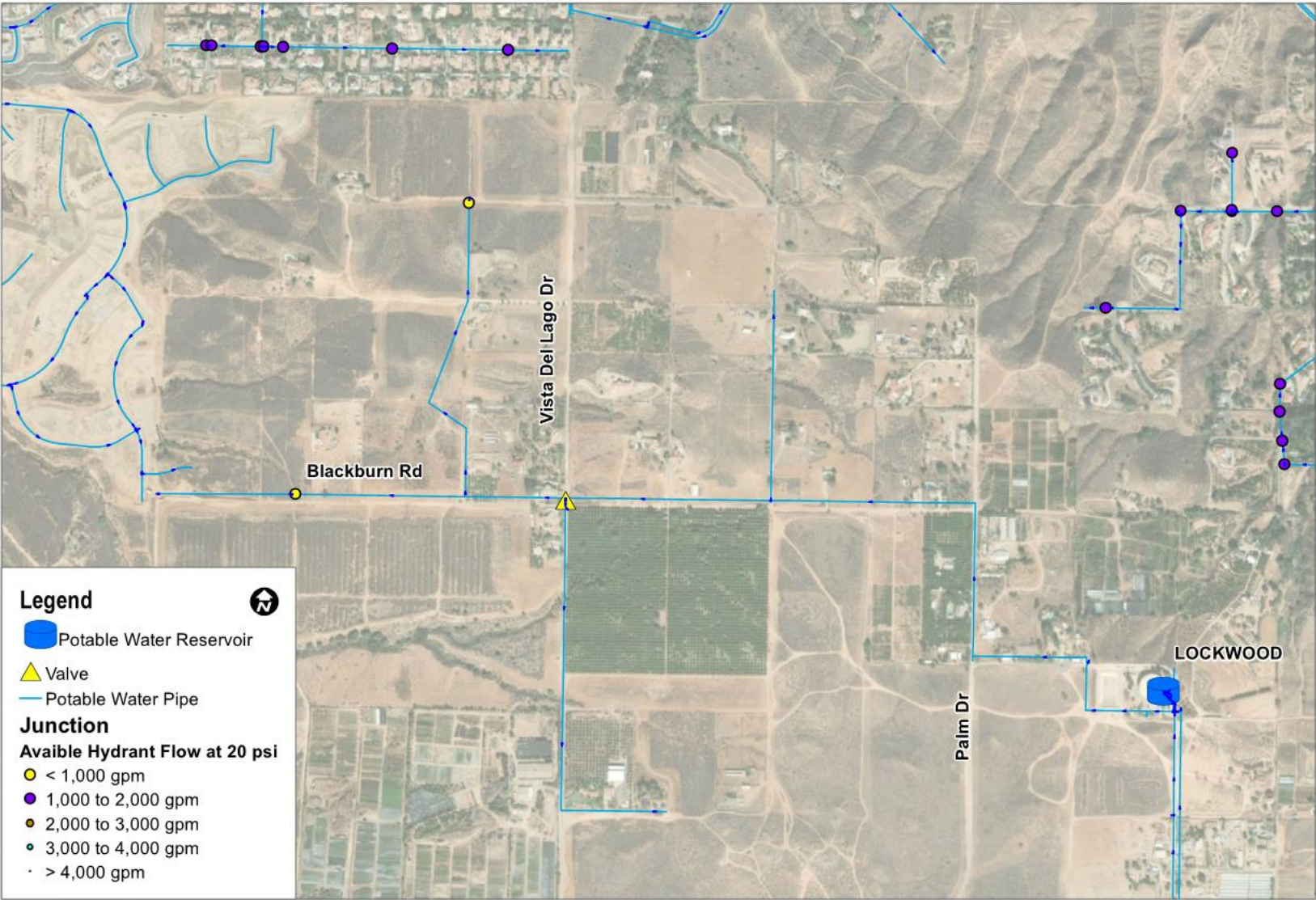
Figure 6-3: Blackburn Road Existing Pipelines and Hydrants
