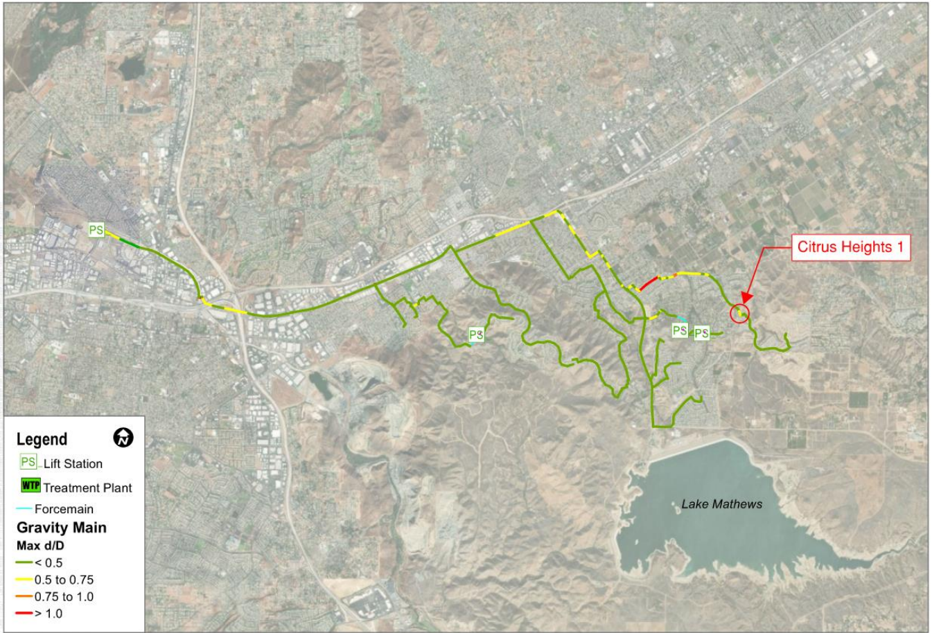
Figure 8-3: Near-Term Sewer Gravity and Force Main Recommendations 1
