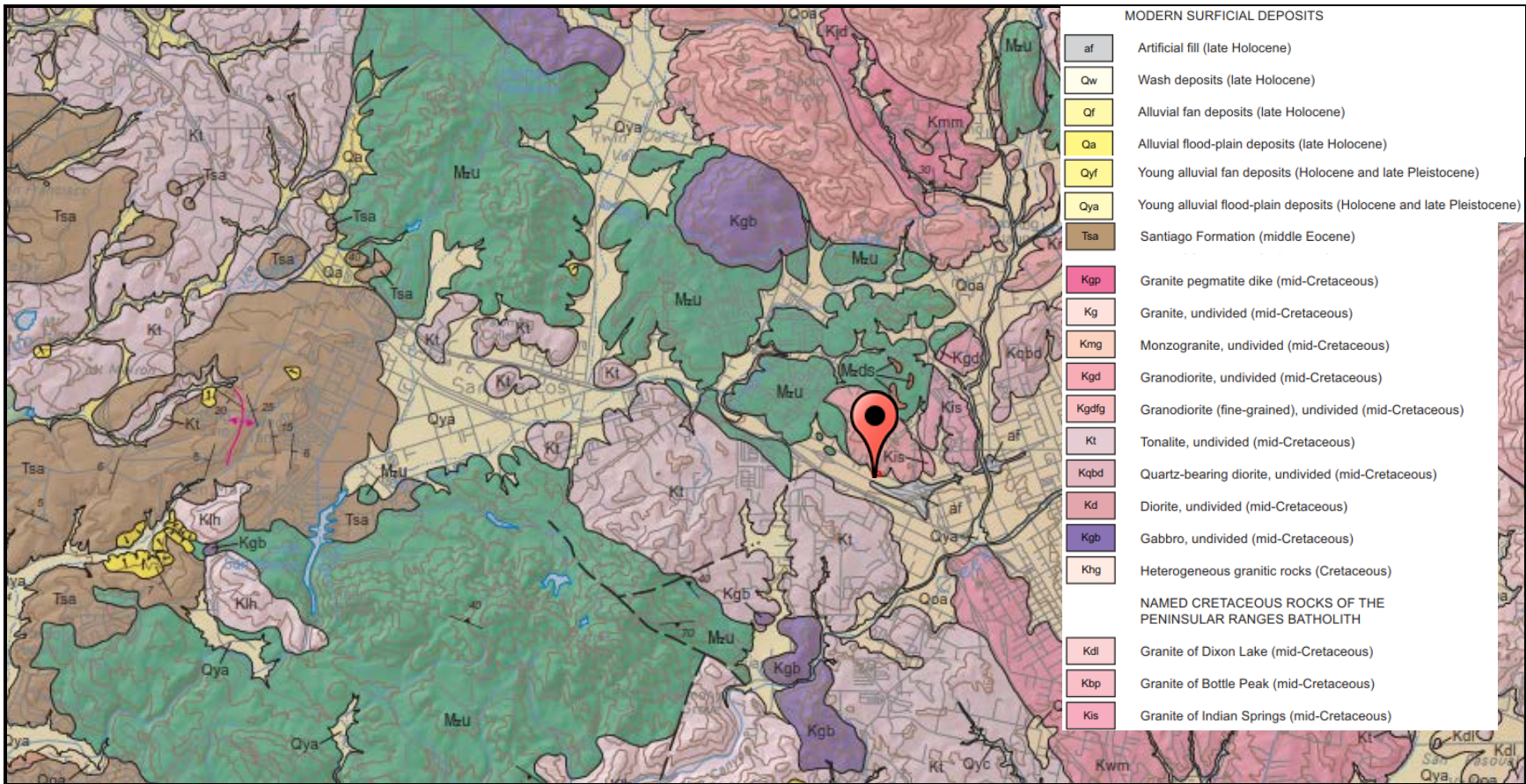
Source: CGS, Geologic Map of the Oceanside 30' x 60' Quadrangle, 1: 100,000 scale. Compiled by Kennedy and Tan, 2007.
