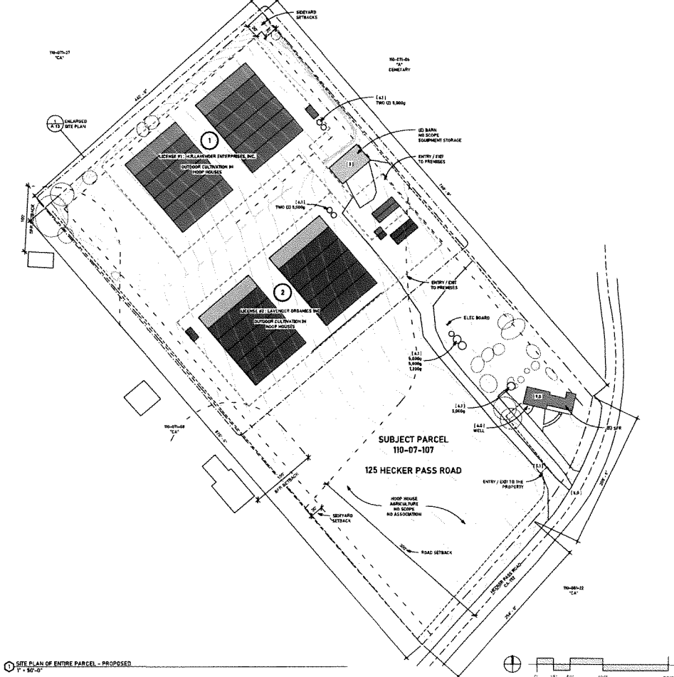
① SITE PLAN OF ENTIRE PARCEL - PROPOSED 1" = 50'-0"
