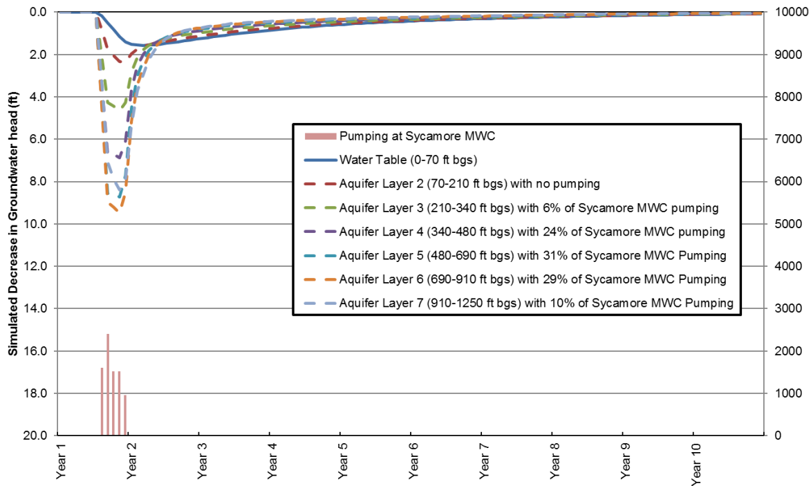
Figure 3-1. Simulated Decrease in Groundwater Head at Location 21 (See Figure H-1b for Location) under the Proposed Action
