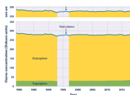
Figure 5. Global Atmospheric Concentrations of Ozone, 1979–2018
