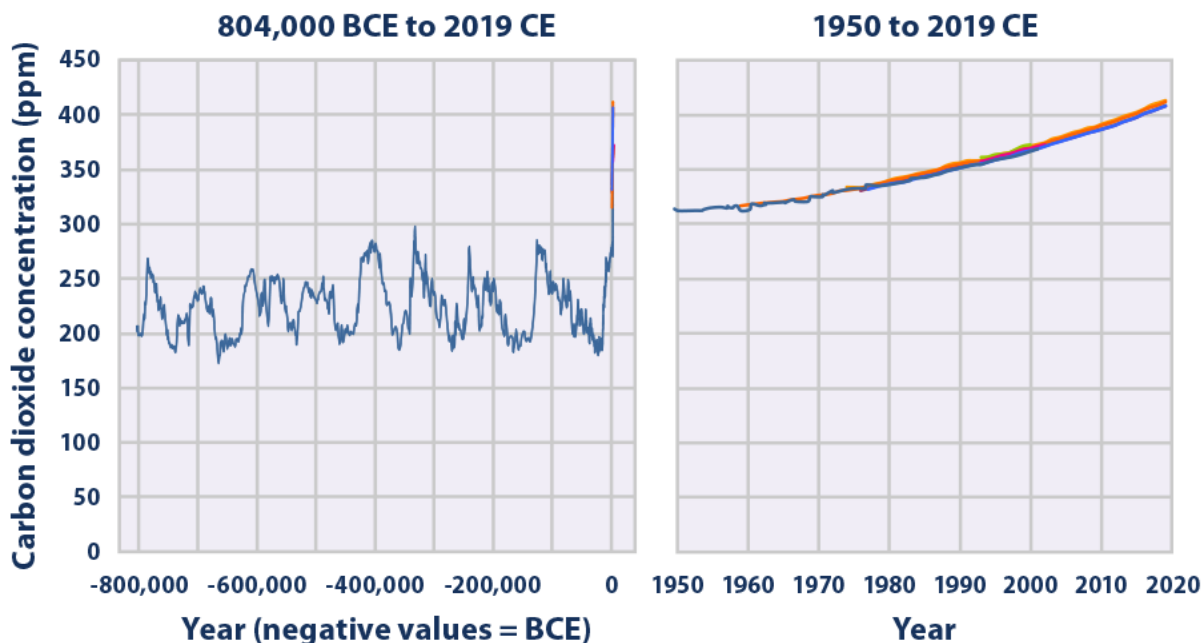
Figure 1. Global Atmospheric Concentrations of Carbon Dioxide Over Time
