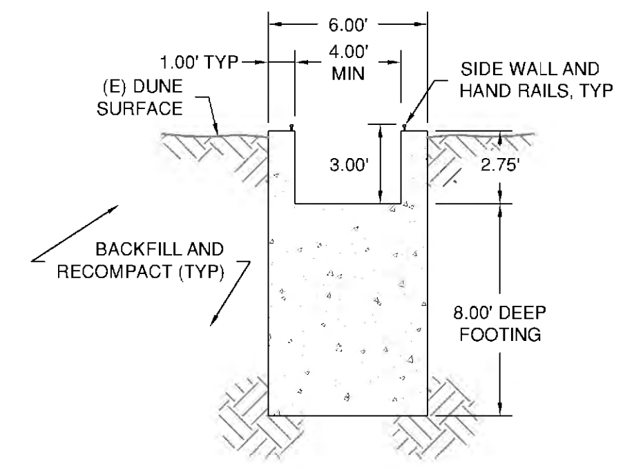
A SECTION 1"=5'
