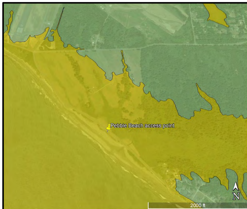
Figure 3: Projected tsunami runup, Pebble Beach access point (CGS, 2021)
