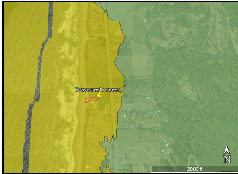
Figure 2: Projected tsunami runup, Wavecrest Beach access point (CGS, 2021)
