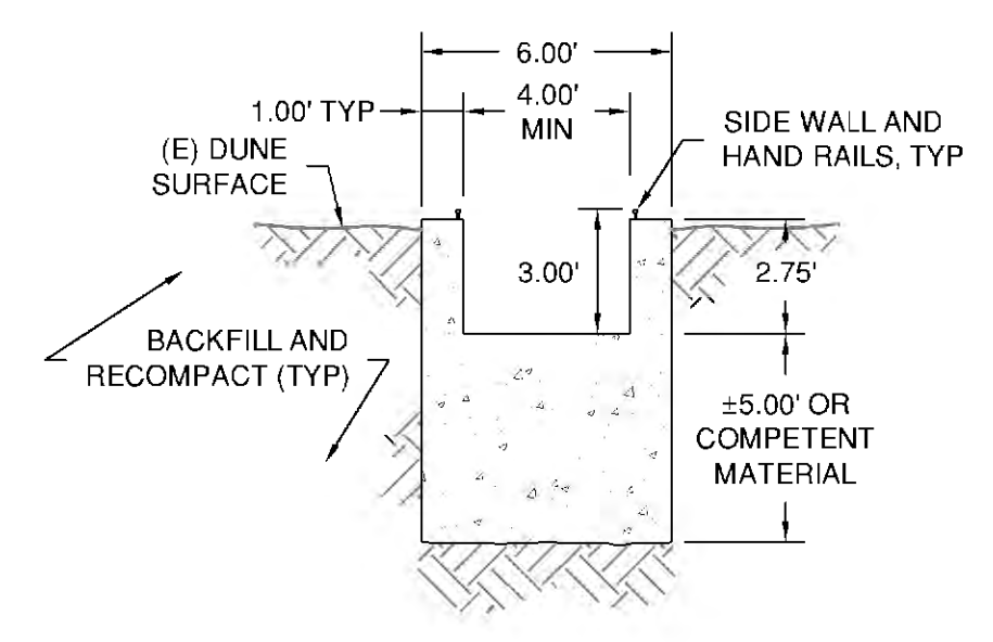
B SECTION 1"=5'
