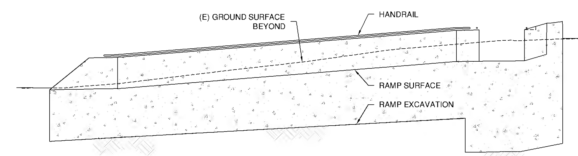
C TYPICAL SECTION 1"=5'
