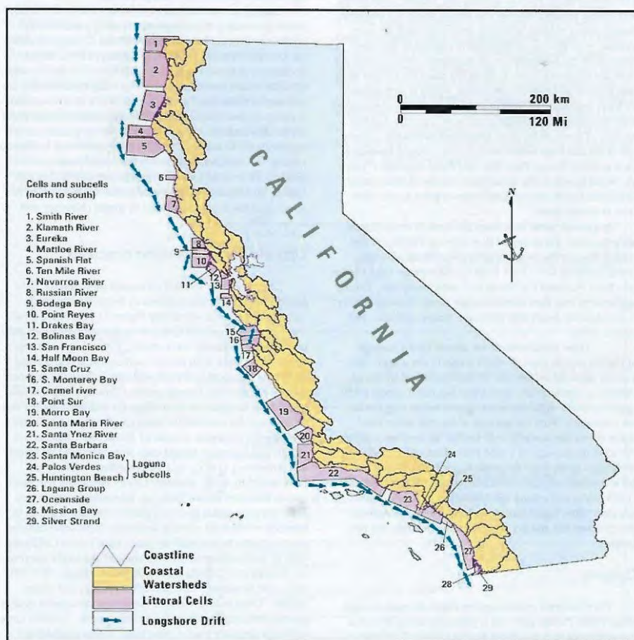
Figure 6: Major littoral cells, coastal watersheds, and conceptual net longshore drift directions for the California coast, modified from Habel and Armstrong (1977) and Hapke et al. (2006).
