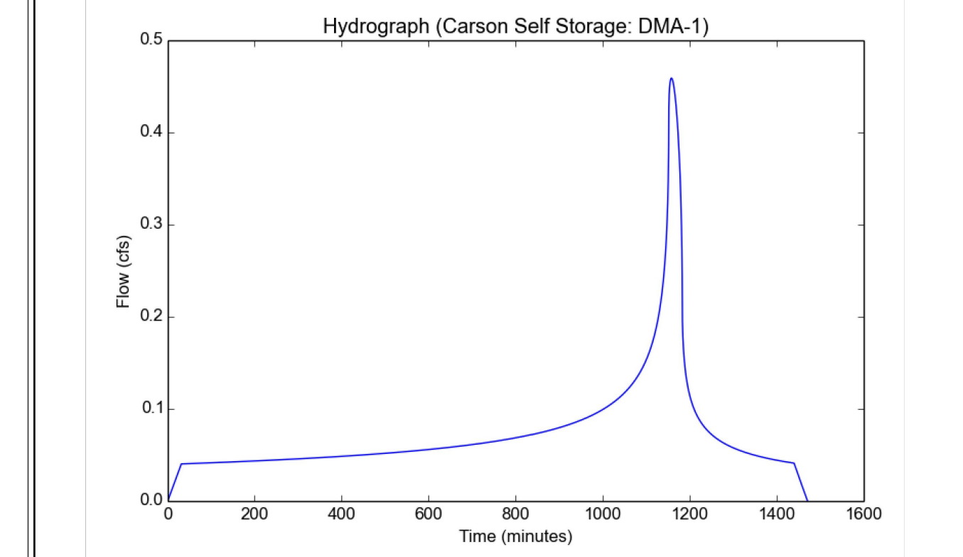
PROJECT HYDROGRAPH
