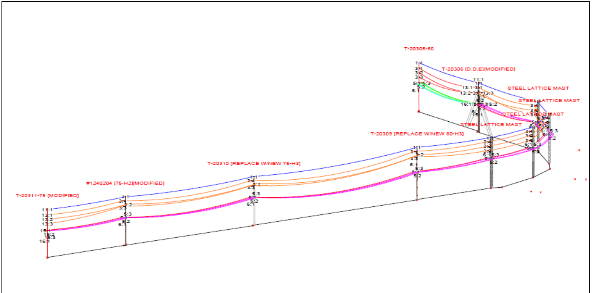
R-Line UPGRADE PHASE 2 – SALT CREEK Project (No. 200253) Line Segment Relocation/Replacement Illustration
