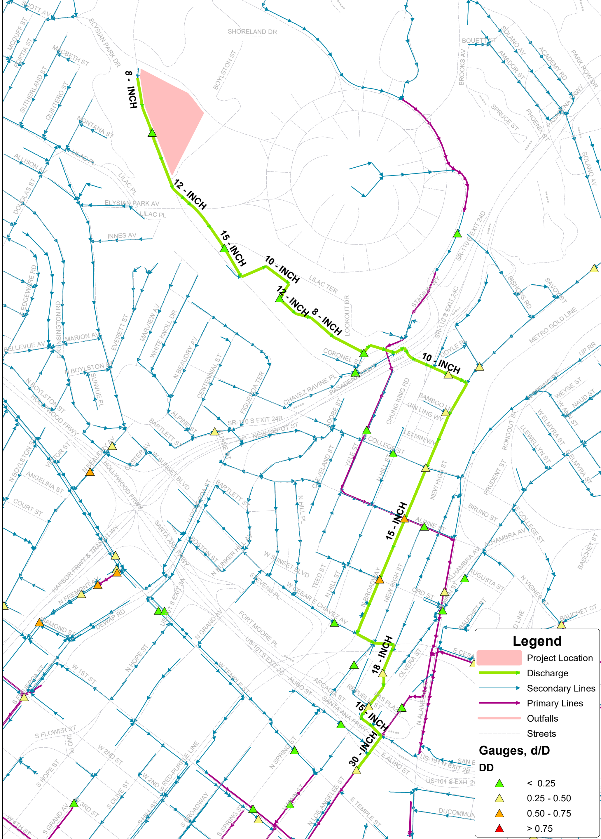
Figure 1 Barlow Respiratory Hospital Project Sewer Map
