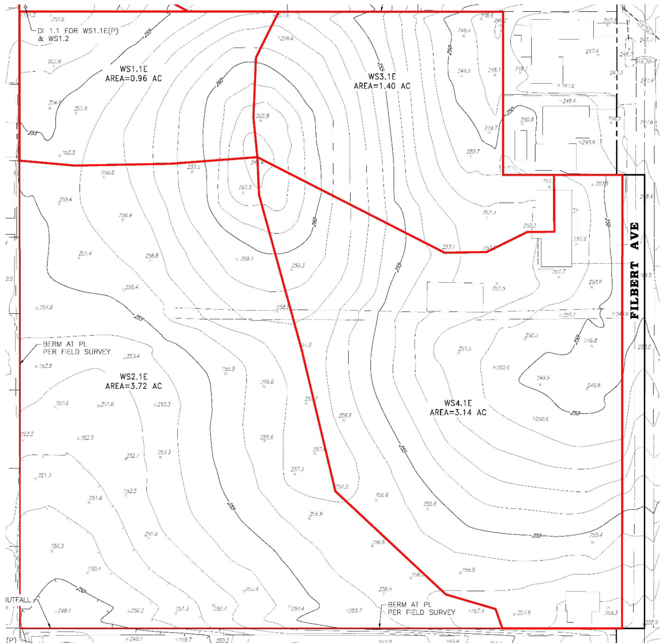
Plate IS-8: Existing Watersheds Onsite
