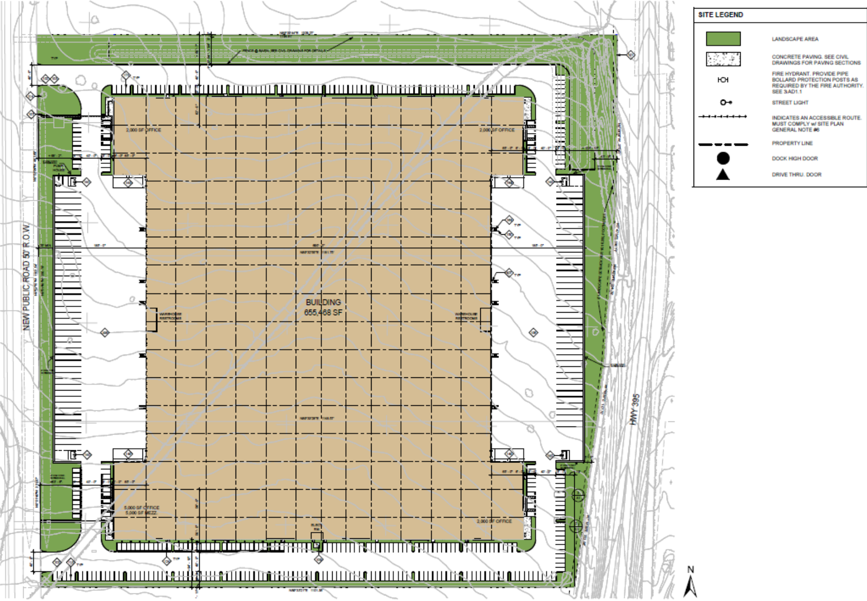
Figure 2: Site Plan
