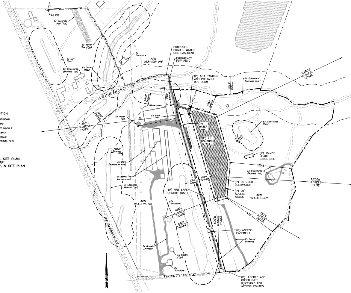
OVERALL SITE PLAN
