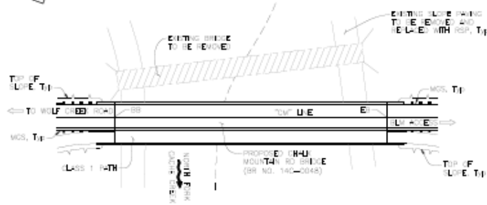
PLAN NO SCALE
