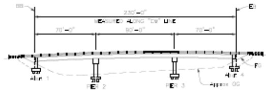
ELEVATION NO SCALE
