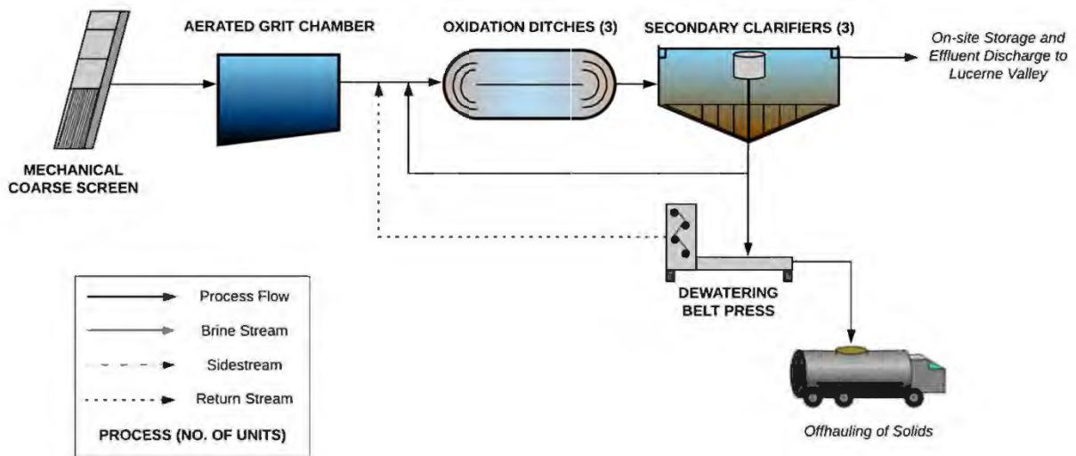
Exhibit 3-2: EXISTING TREATMENT PROCESS SCHEMATIC
