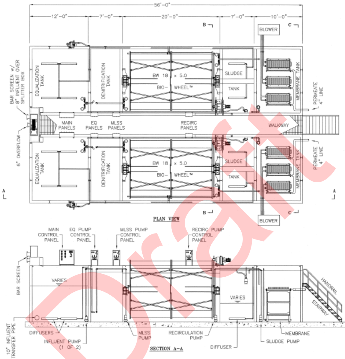
Figure 3-4 Existing Facilities
