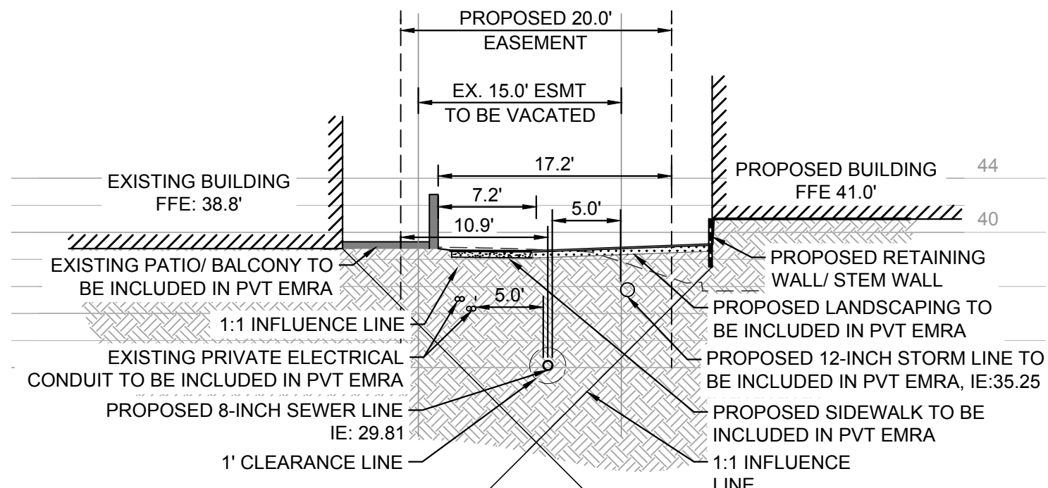
SEWER CROSS SECTION B-B SCALE: 1" = 10'
