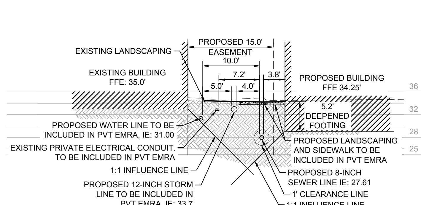
SEWER CROSS SECTION C-C SCALE: 1" = 10'
