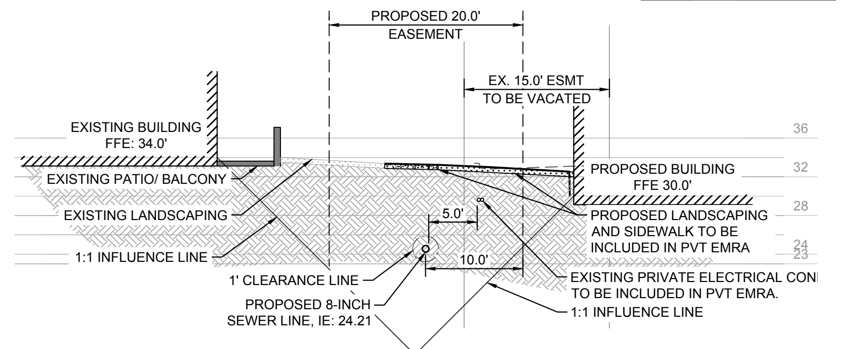
SEWER CROSS SECTION D-D SCALE: 1" = 10'
