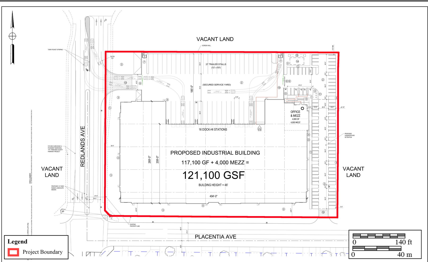
Figure 3 Site Plan
