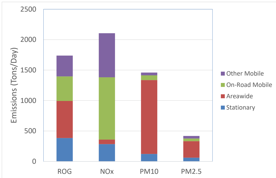
Figure 1: California 2012 Emissions Inventory
