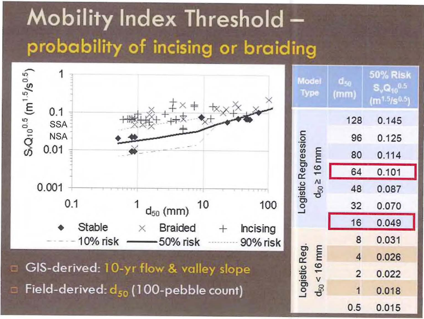
Figure 2.5: Probability of incising/braiding based on logistic regression of Screening Index and d_{50}
