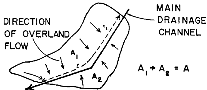
Figure-2-2 Irregular subcatchment shape for width calculations (DiGiano et al., 1977, p.165).
