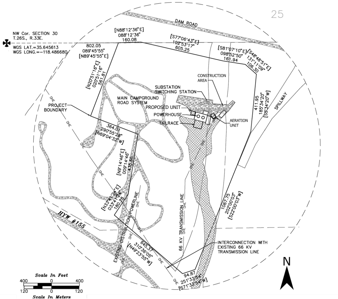
Figure 2-2. Isabella Project Area showing existing generating facilities, proposed generating unit, and Construction Area.
