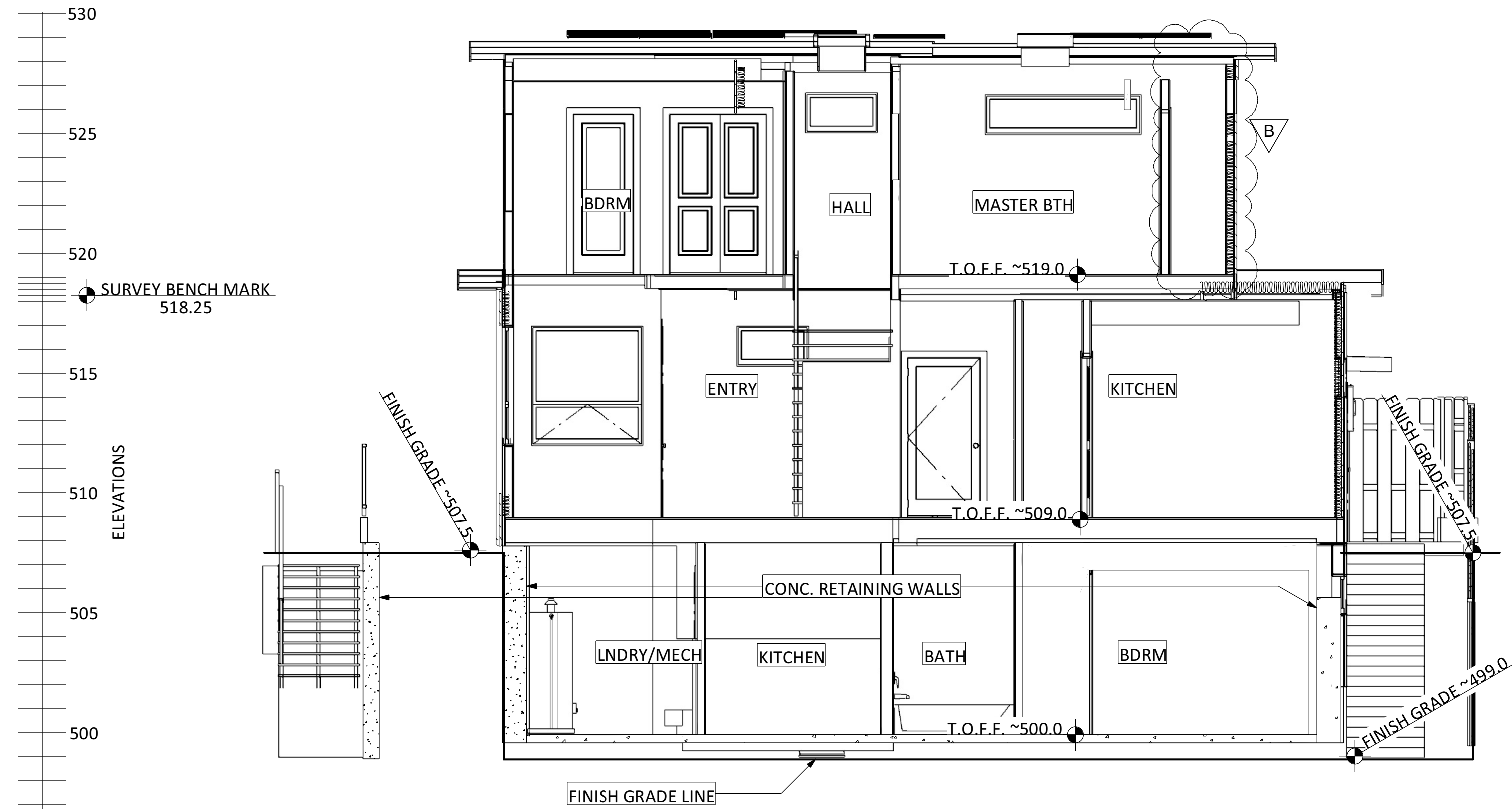
2 CROSS SECTION 2-2 Scale 1/4" = 1'-0"
