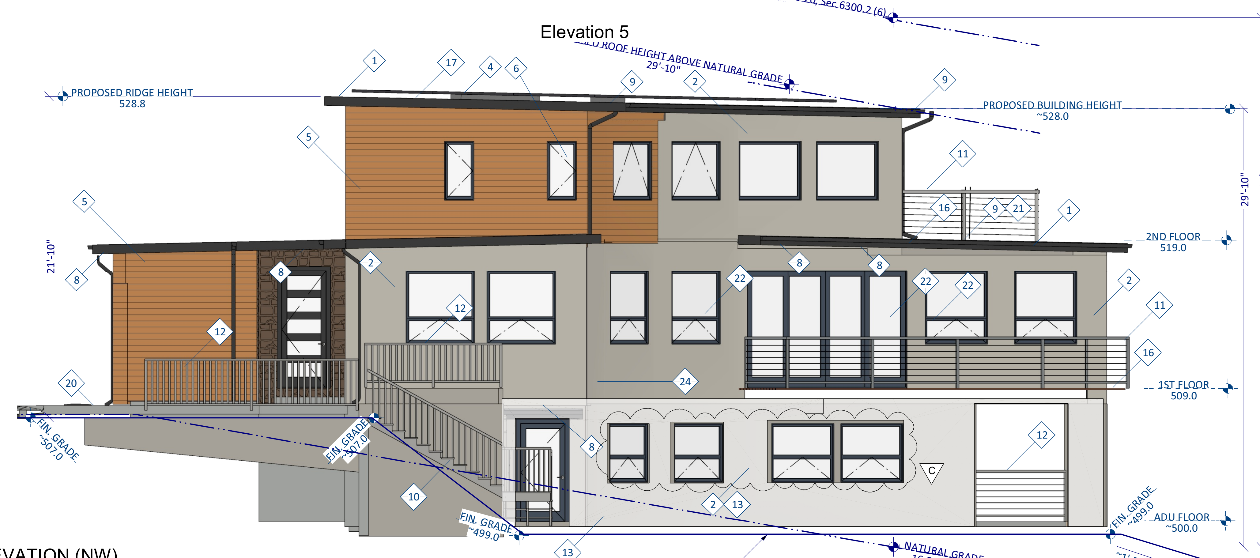
1 RIGHT ELEVATION (NW) scale 1/4" = 1'-0"
