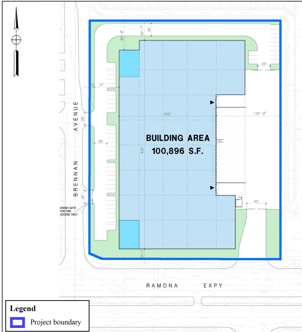
Figure 3 Conceptual Site Plan The Ramona and Brennan Project
