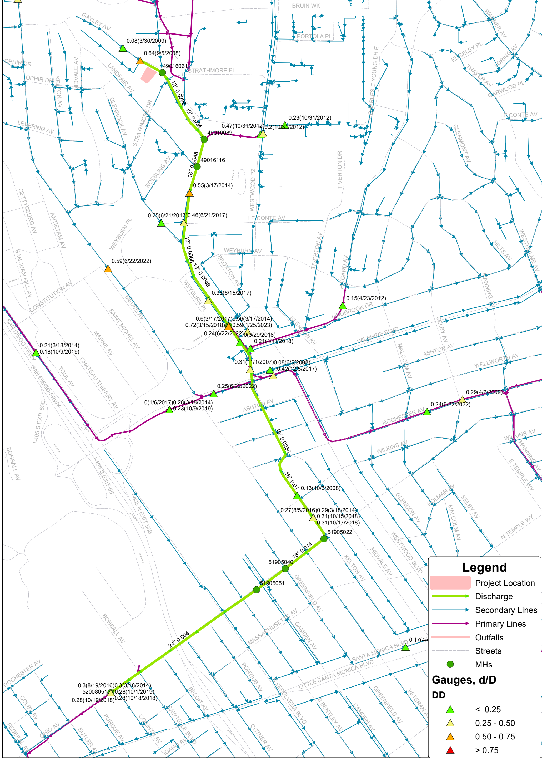
Figure 1 565 1-51 S GAYLEY AVE Sewer Map
