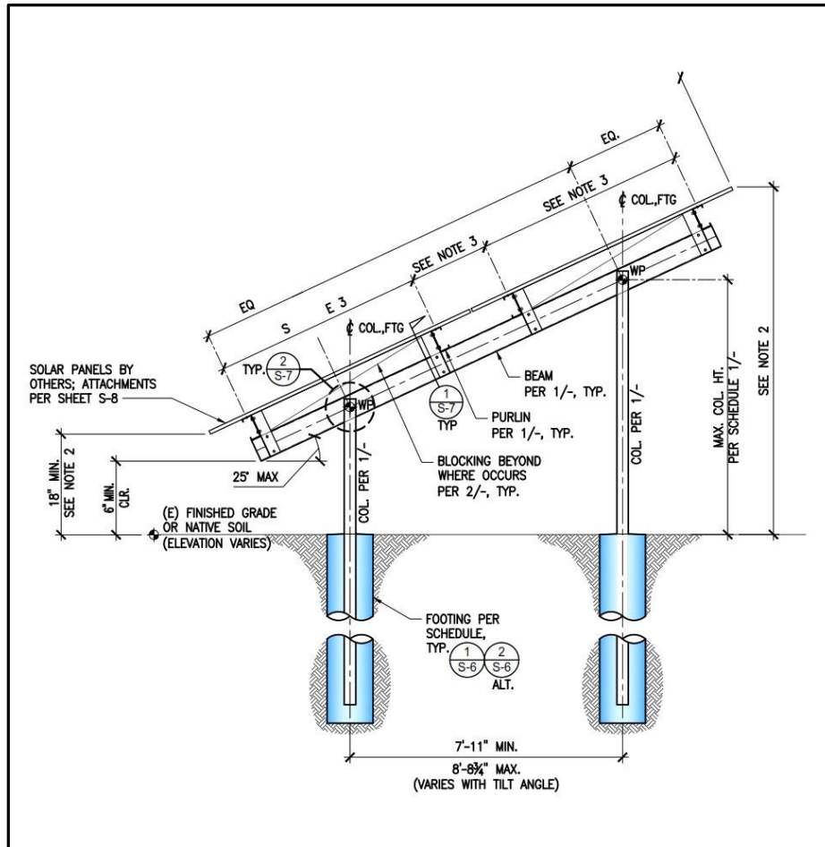
Figure 1 – Example pV Ground-Mounted Array, Section View
