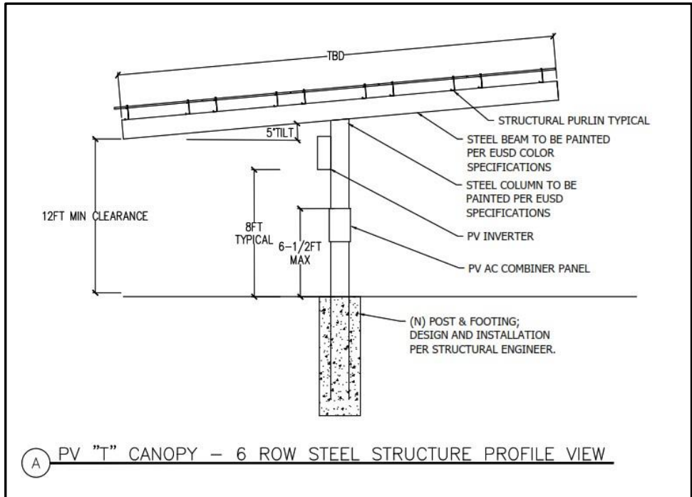
Figure 2 - Example pV Parking Lot Canopy Array, Section View
