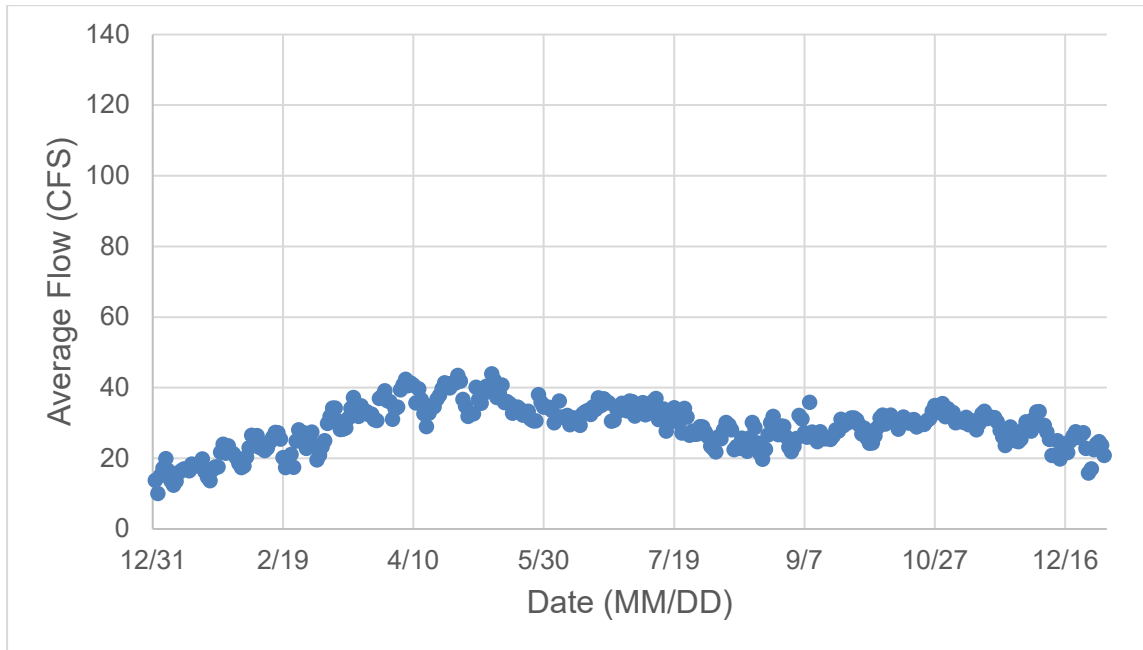
Figure D-5. South Central Drain (723SCNTDR) Average Daily Flow (2015-2019)
