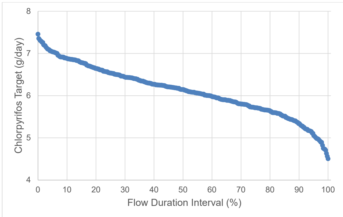
Figure D-17. Holtville Main Drain (723HVLDRN) Chlorpyrifos Load Duration Curve
