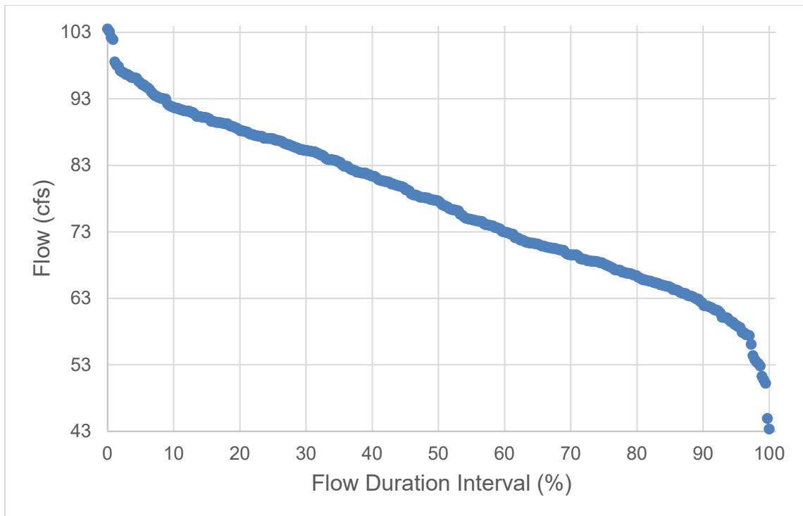
Figure D-11. Rose Drain (723ROSDRN) Flow Duration Curve
