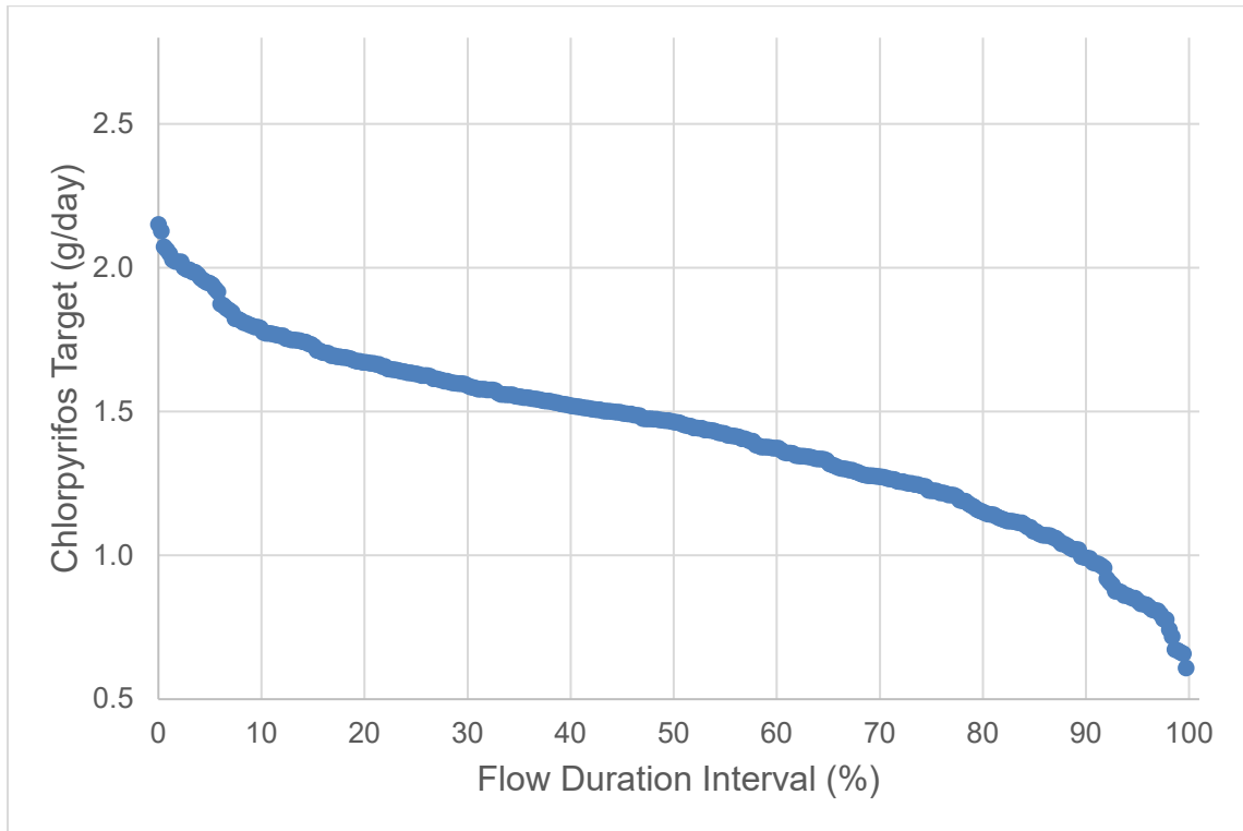
Figure D-19. South Central Drain (723SCNTDR) Chlorpyrifos Load Duration Curve
