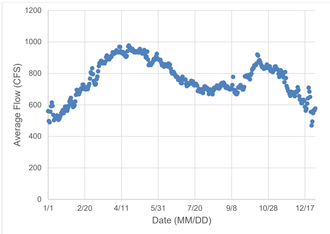
Figure D-1. Alamo River Outlet (723ARGRB) Average Daily Flow (2015-2019)
