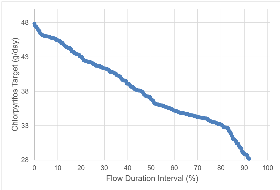
Figure D-15. Alamo River Outlet (723ARGRB) Chlorpyrifos Load Duration Curve
