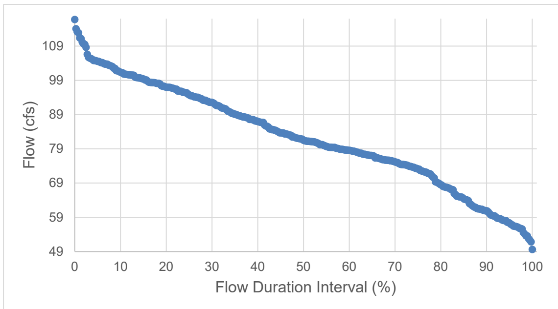
Figure D-11. Rose Drain (723ROSDRN) Flow Duration Curve
