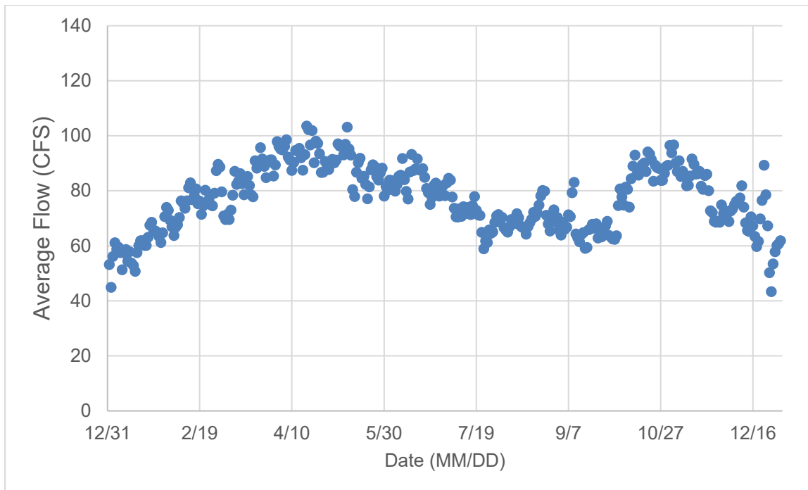
Figure D-3. Holtville Main Drain (723HVLDR) Average Daily Flow (2015-2019)
