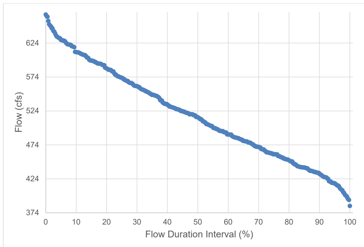
Figure D-14. New River Outlet Salton Sea (723NRWM) Flow Duration Curve
