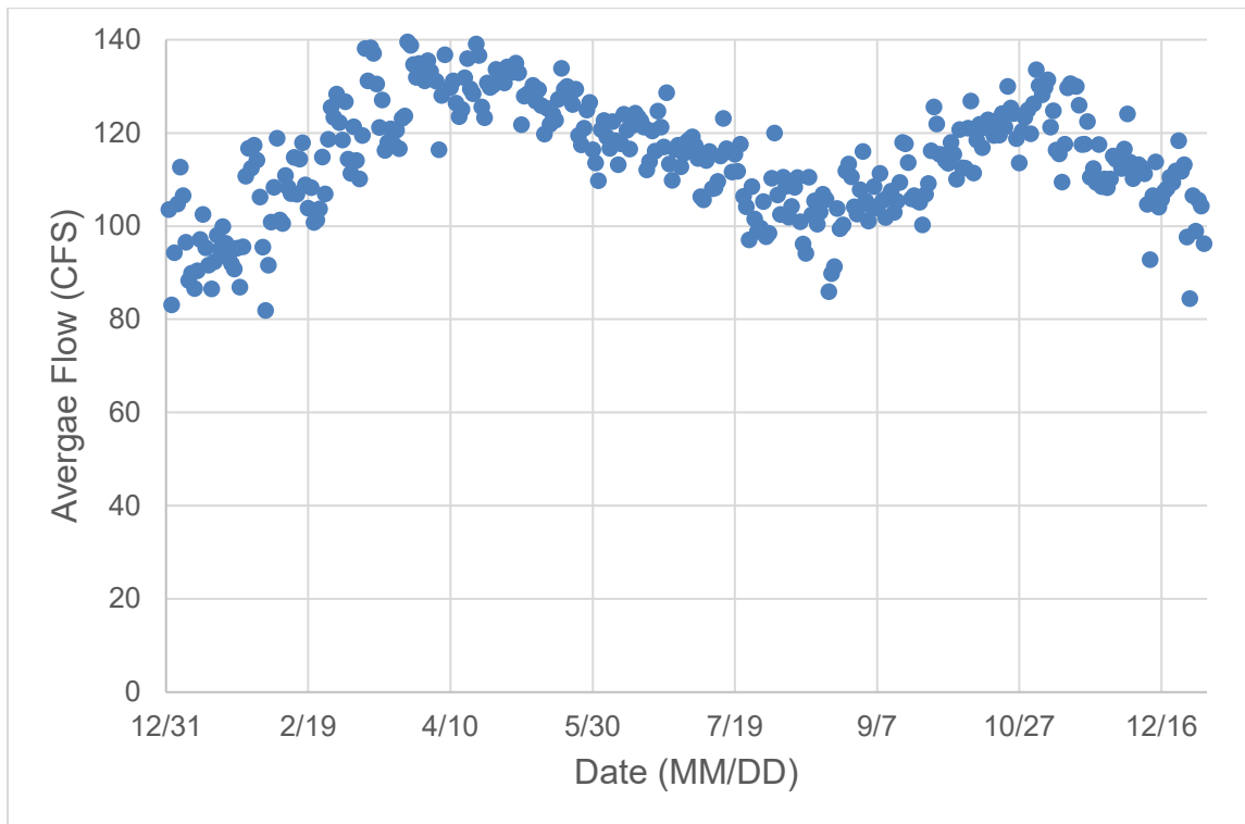
Figure D-2. Central Drain (723CNTDRN) Average Daily Flow (2015-2019)
