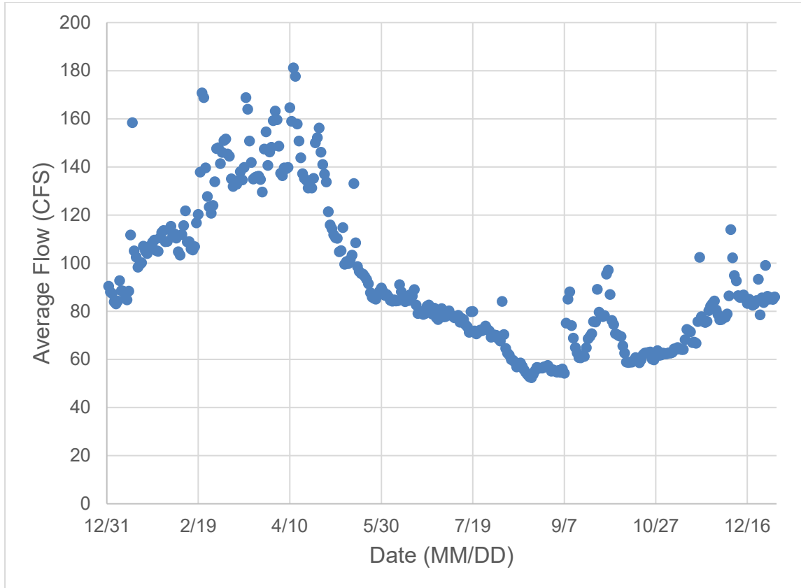
Figure D-6. New River International Boundary (723NRBDRY) Average Daily Flow (2015-2019)
