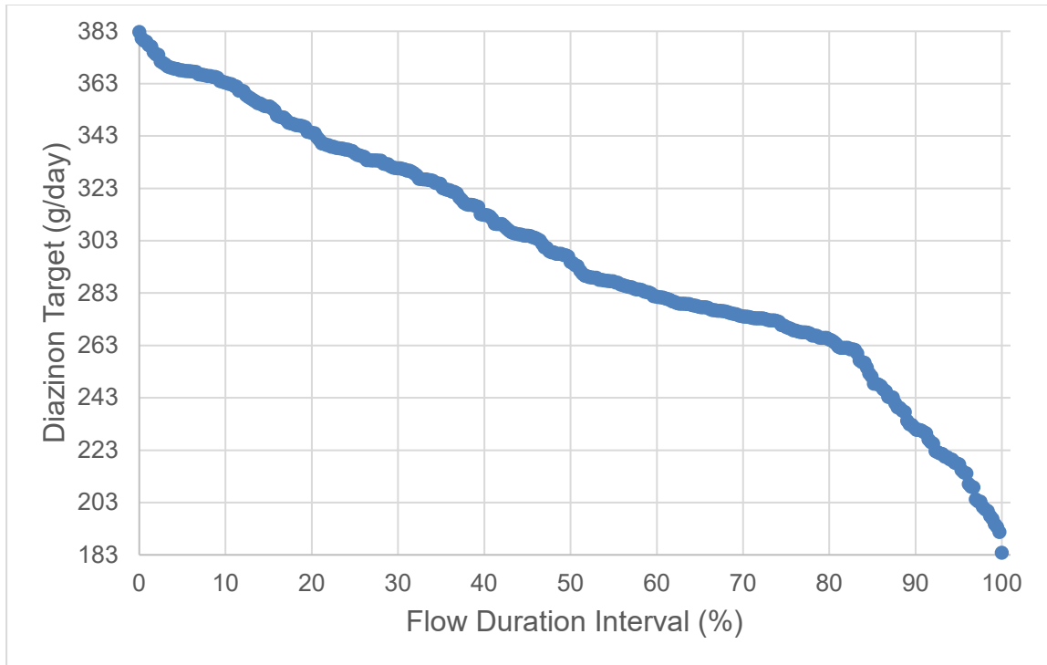
Figure D-21. Alamo River Outlet (723ARGRB) Diazinon Load Duration Curve
