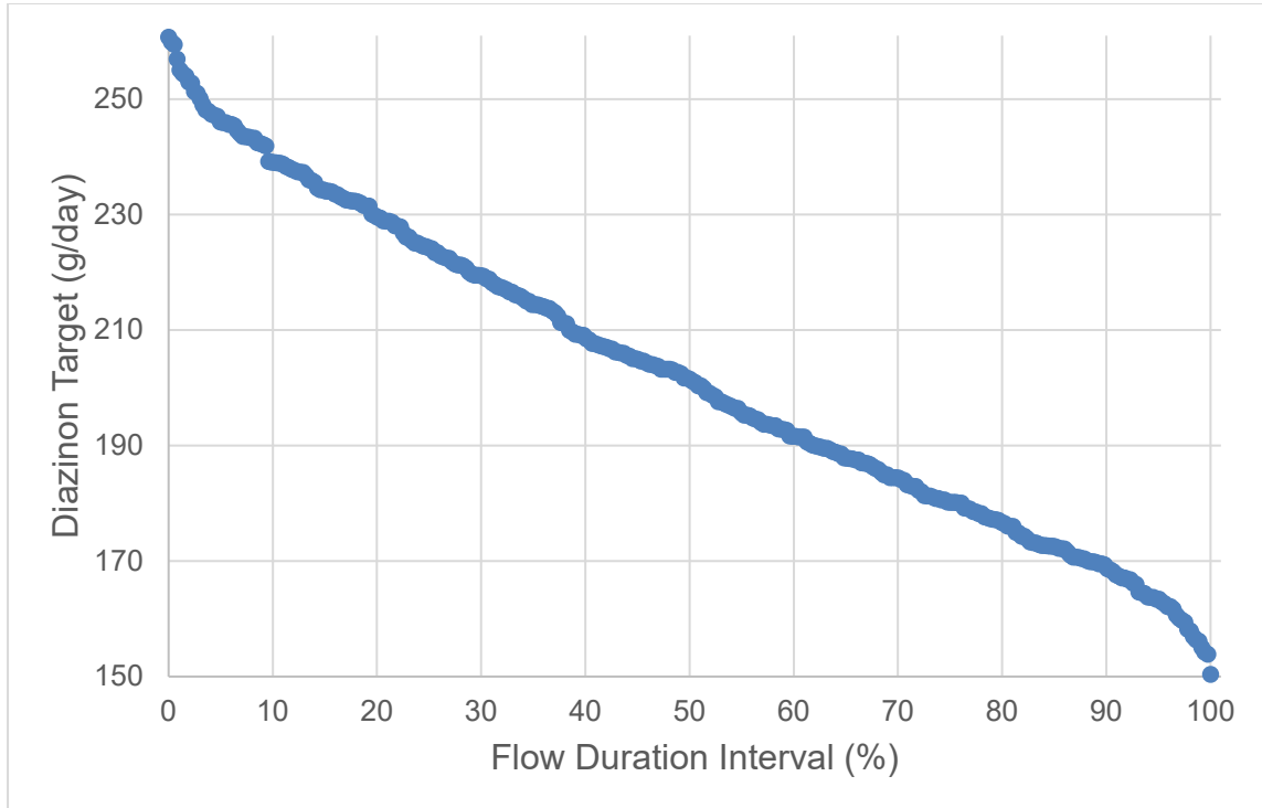
Figure D-23. New River Outlet Salton Sea (723NROTWM) Diazinon Load Duration Curve
