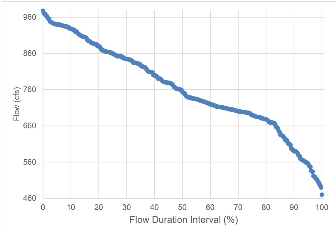
Figure D-8. Alamo River Outlet (723ARGRB) Flow Duration Curve
