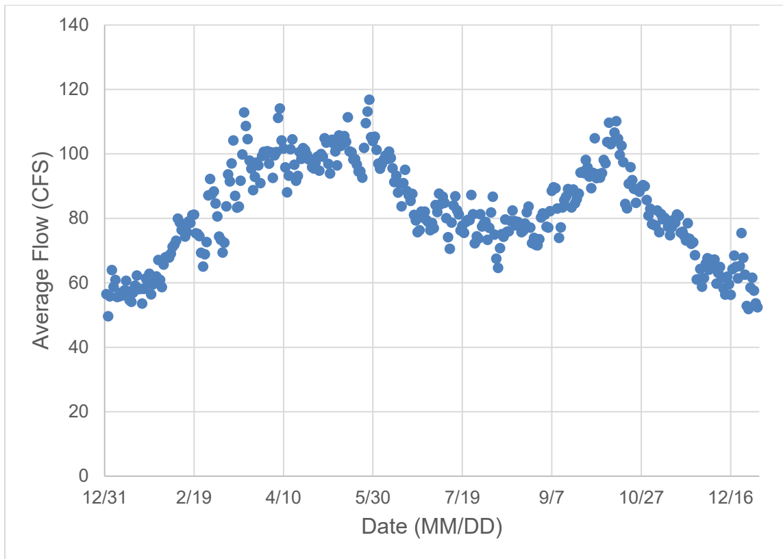
Figure D-4. Rose Drain (723ROSDRN) Average Daily Flow (2015-2019)
