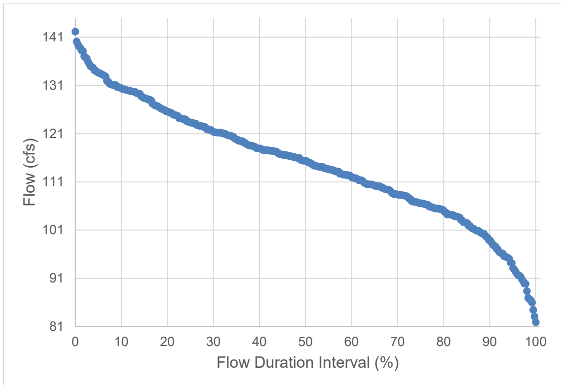
Figure D-9. Central Drain Flow (723CNTDRN) Flow Duration Curve
