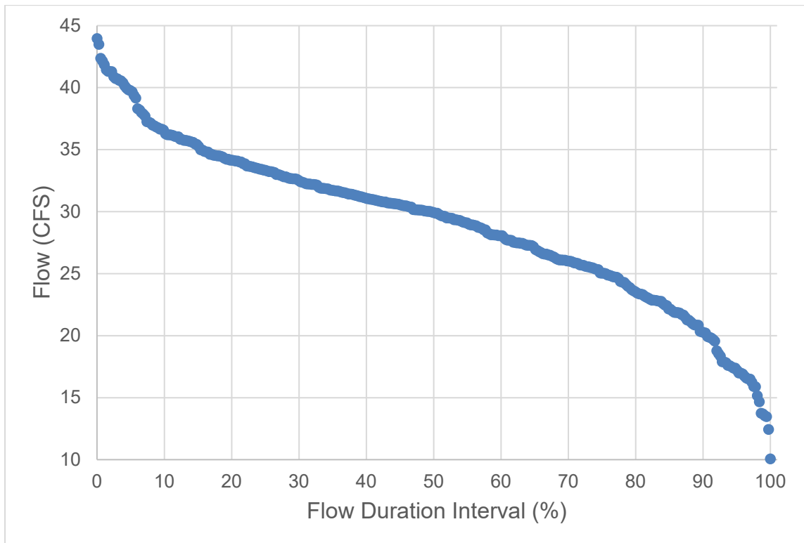
Figure D-12. South Central Drain (723SCNTDR) Flow Duration Curve
