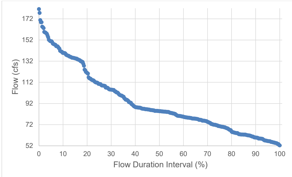
Figure D-13. New River International Boundary (723NRBDRY) Flow Duration Curve
