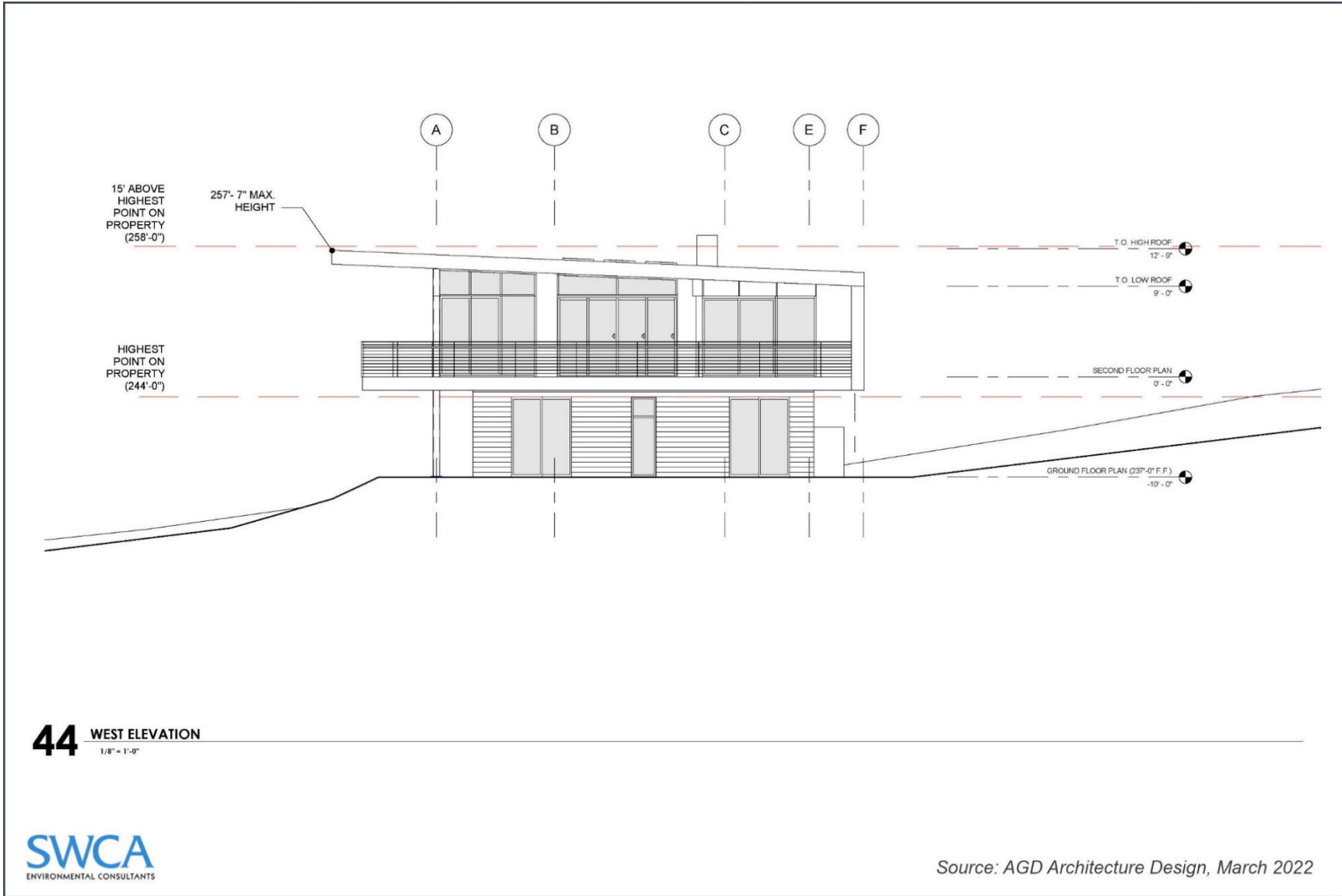
Figure 3. Elevation Drawing
