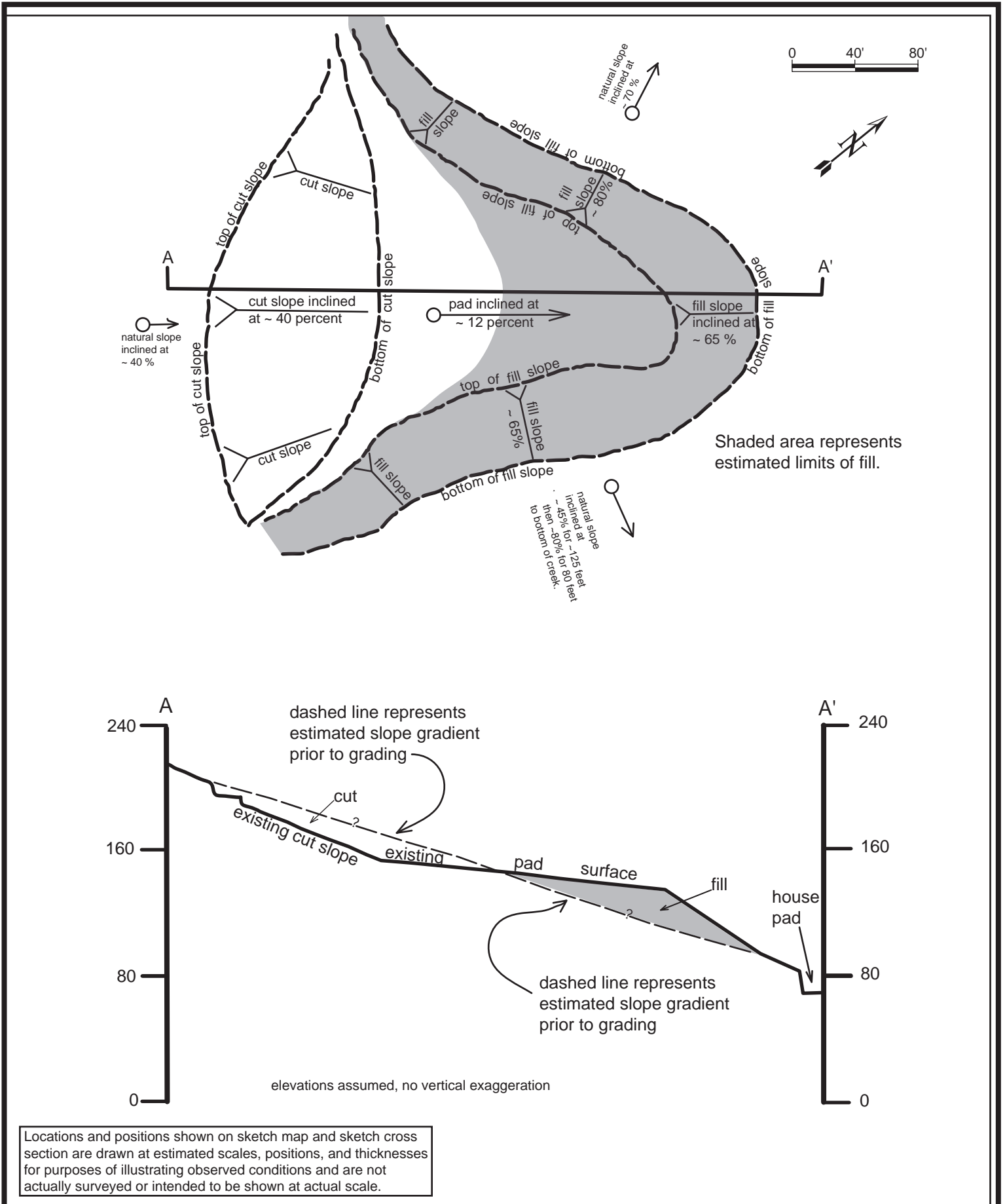
Sketch map and cross section of cut and fill pad # 1 LE Case # 11CAMUE004127-46
