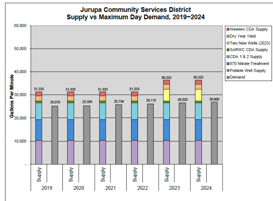
Figure 4.19-1: JCSD Supply vs Maximum Day Demand, 2019-2024
