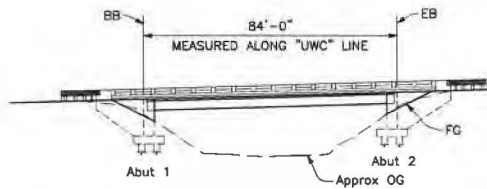
ELEVATION NO SCALE
