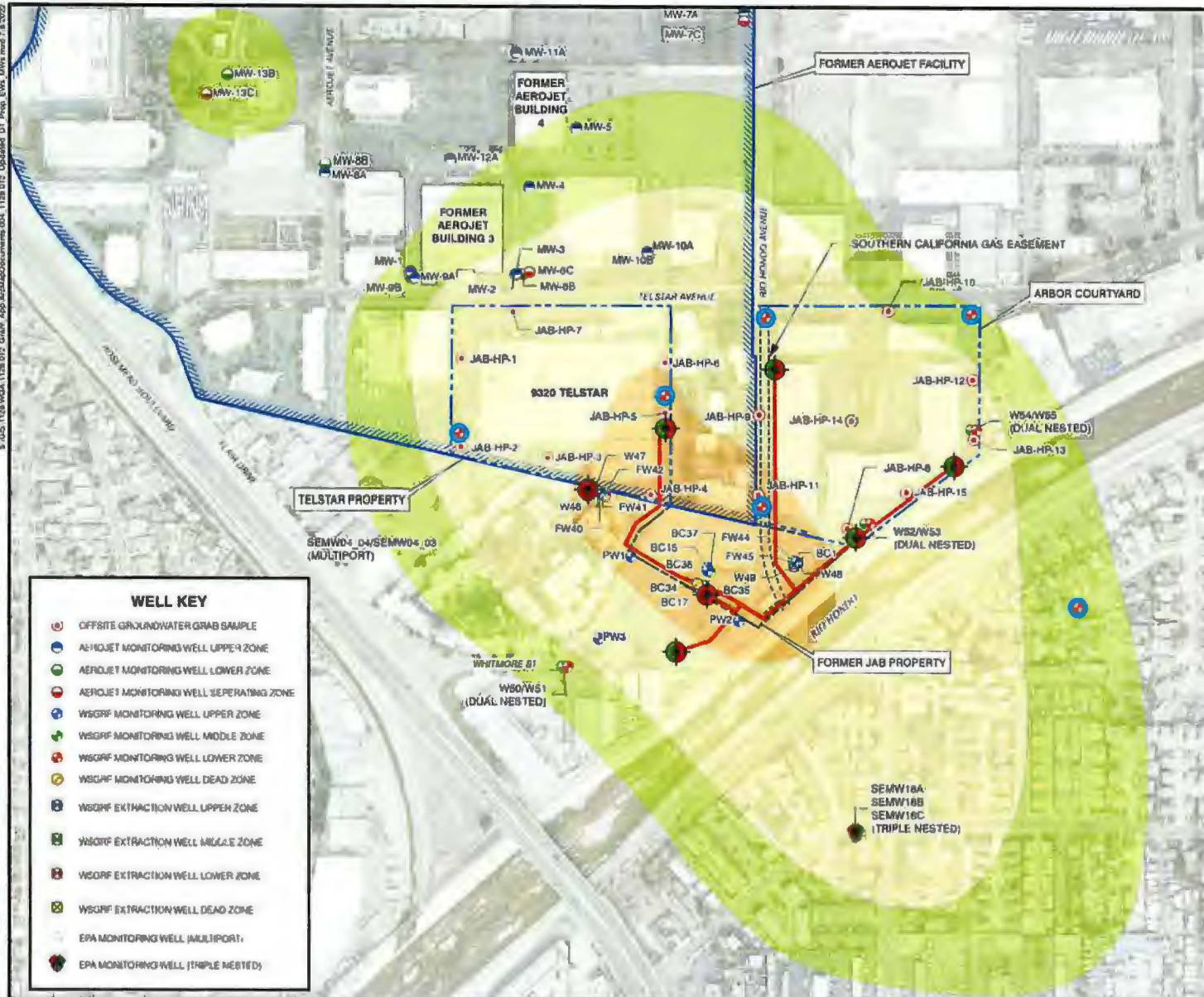
FIGURE 2-9 EXTRACTION AND MONITORING WELL LOCATIONS WSGRF EXPANSION SOUTH EL MONTE OPERABLE UNIT LOS ANGELES COUNTY, CALIFORNIA
