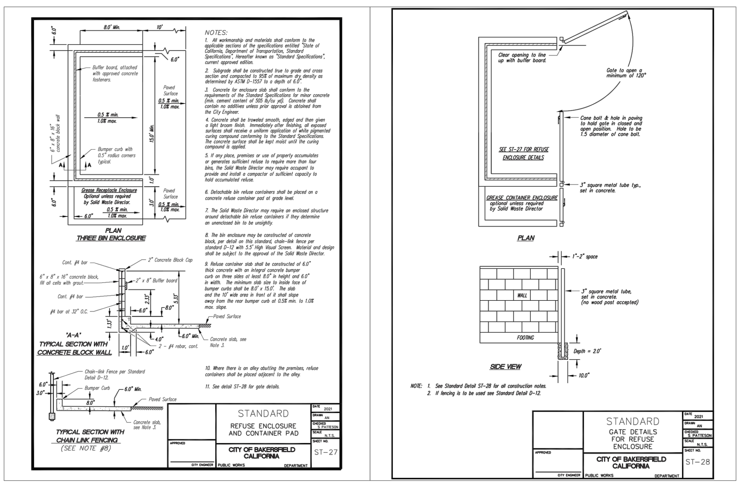
TRASH ENCLOSURE DETAILS
