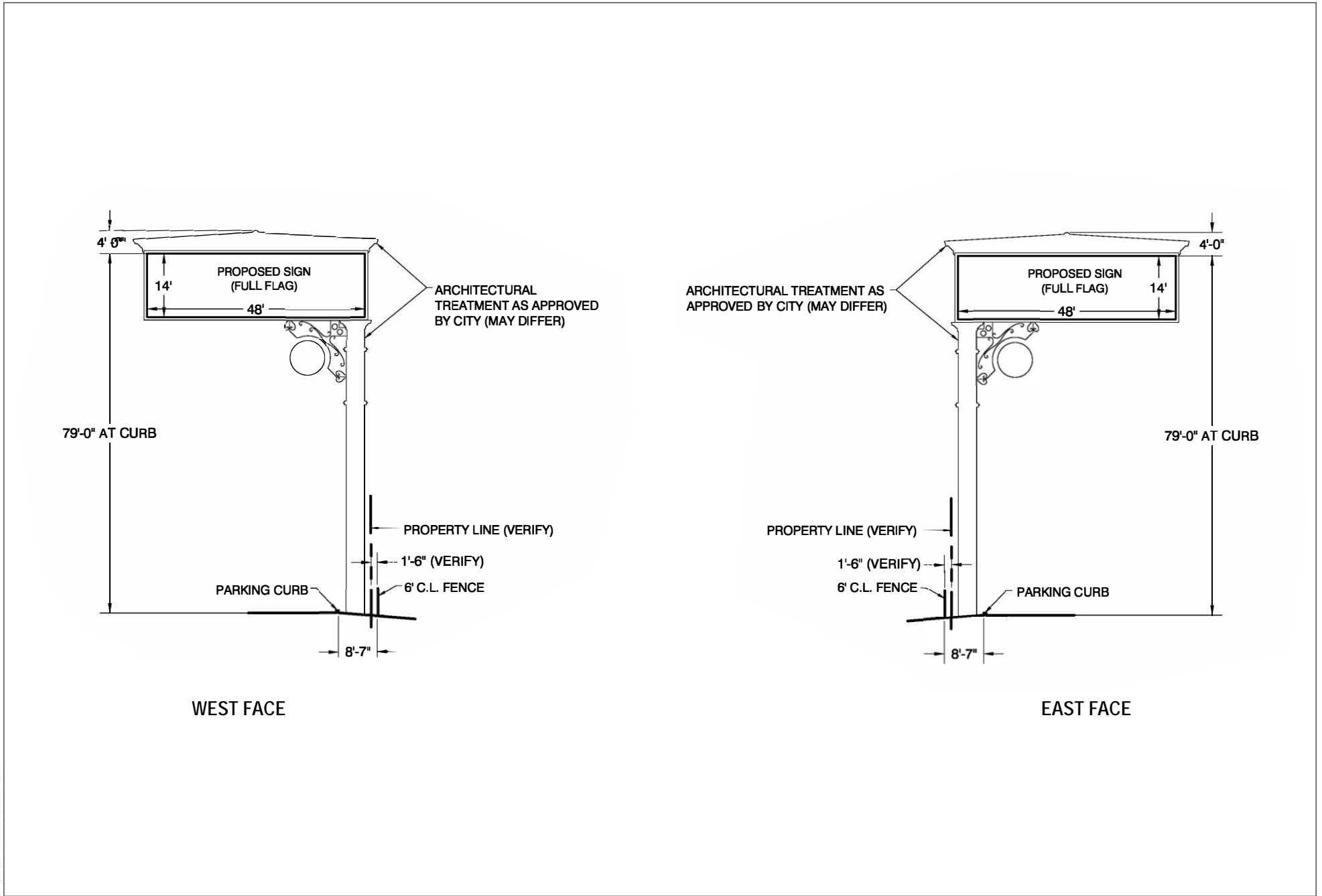
FIGURE 2-3 Project Elevations
