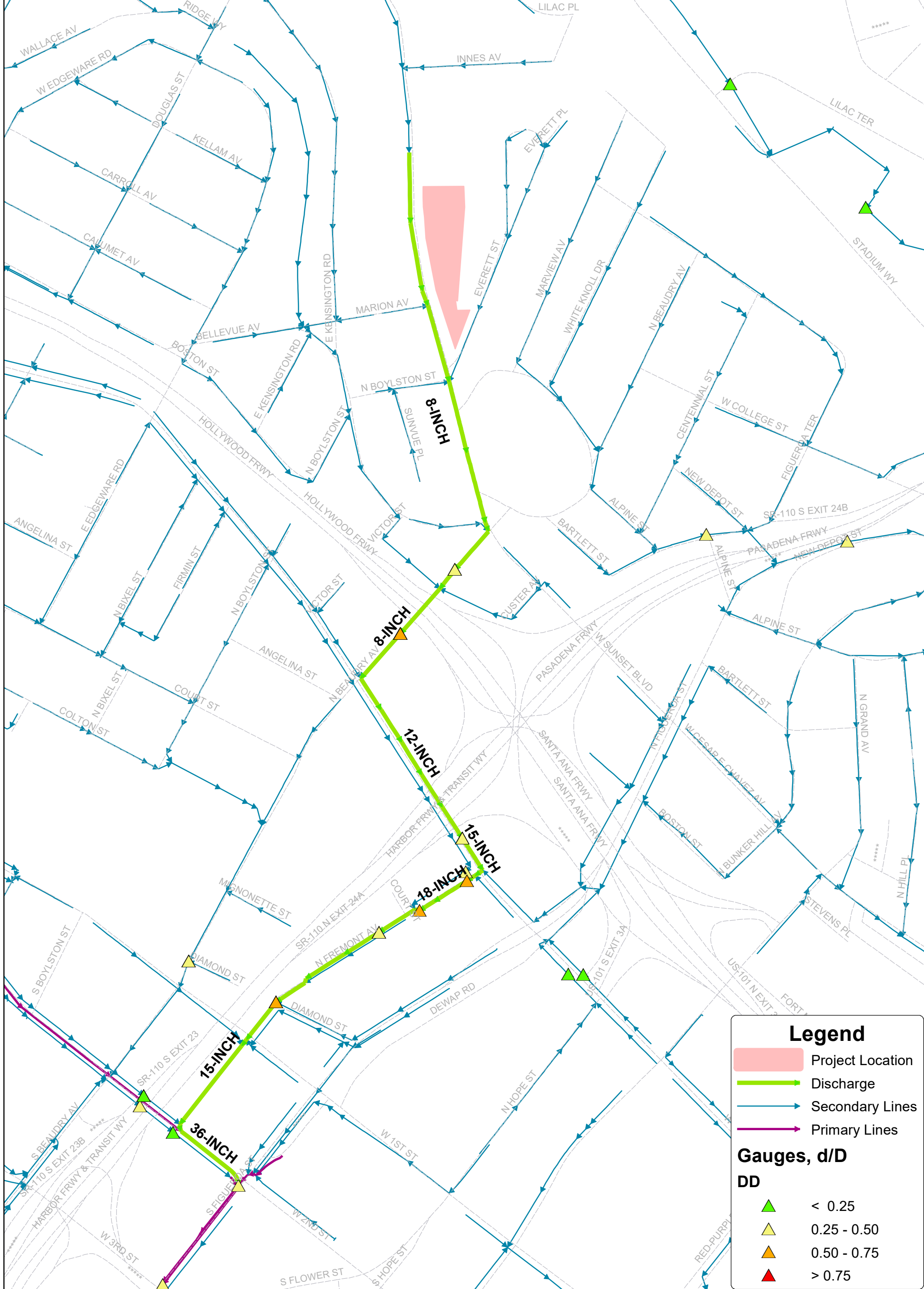
Figure 1 SUNSET AND EVERETT PROJECT Sewer Map
